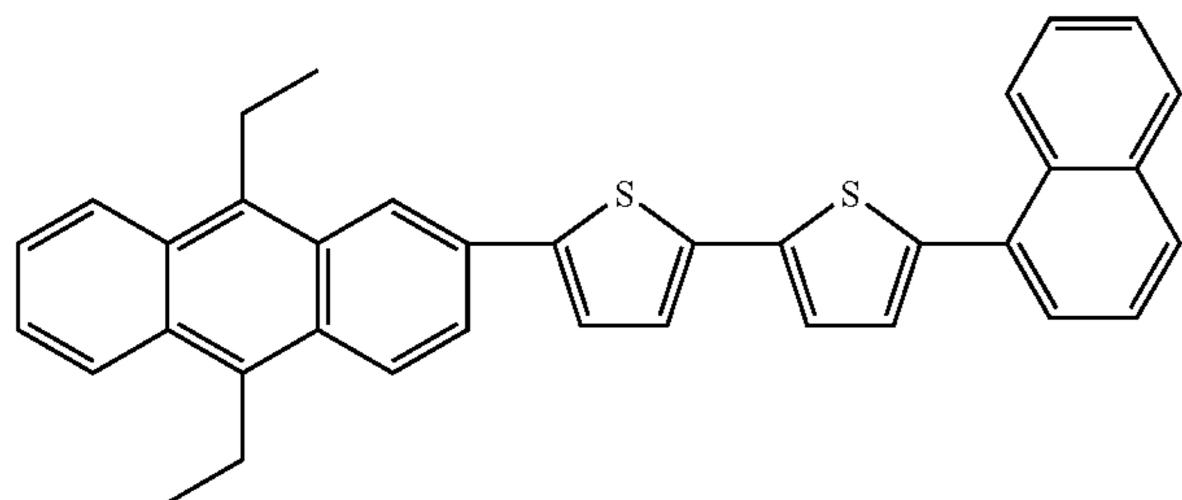
Compound 62
