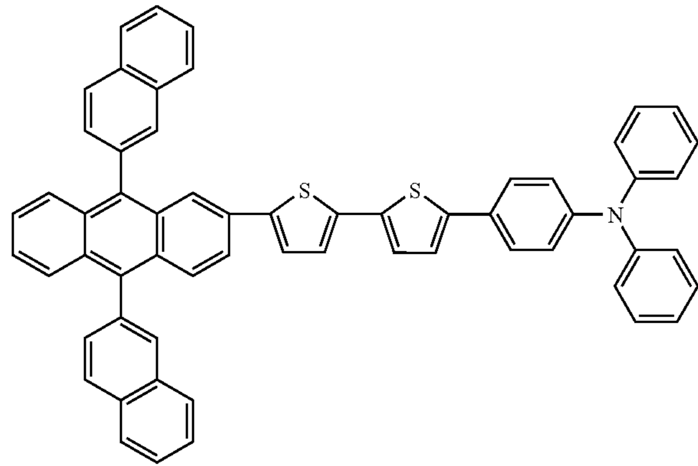
Compound 35
