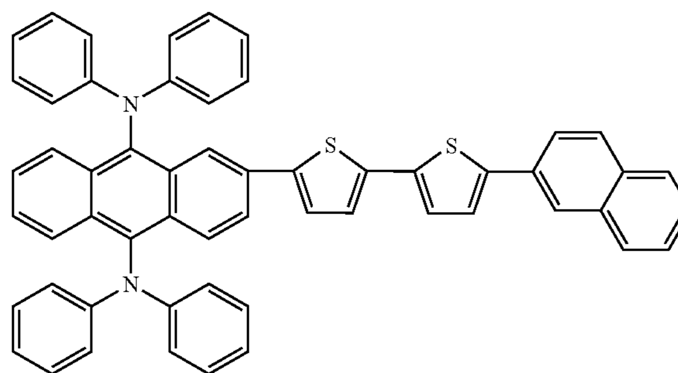
Compound 55
