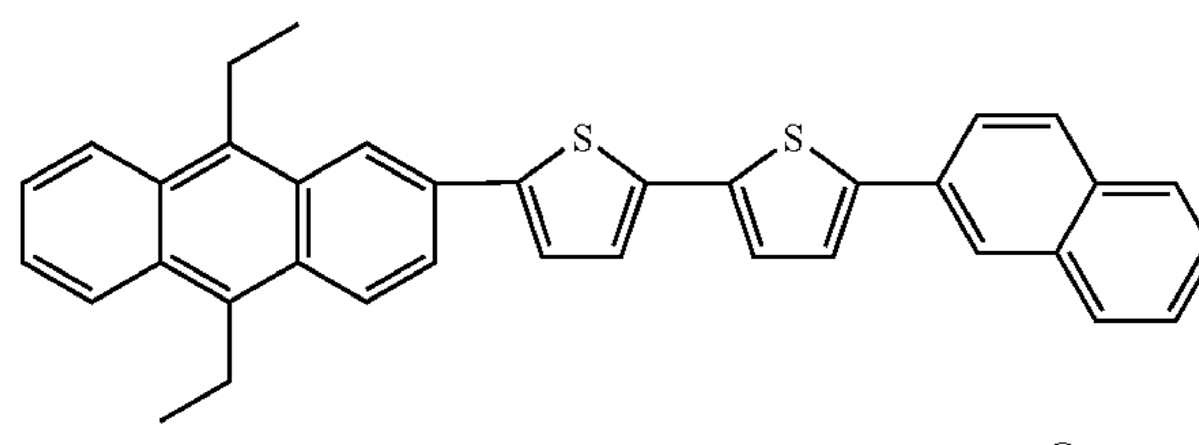
Compound 67
