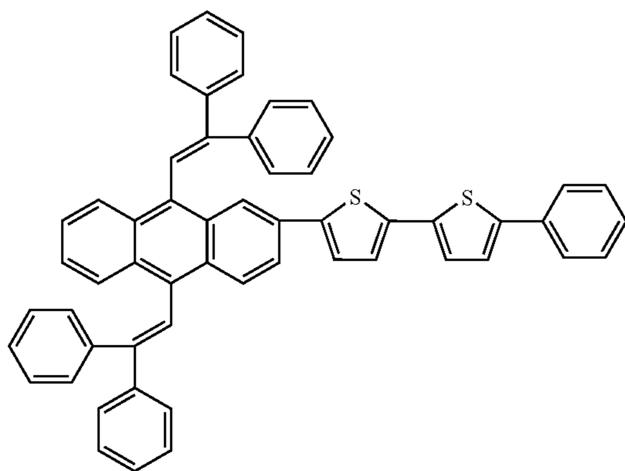
Compound 40
