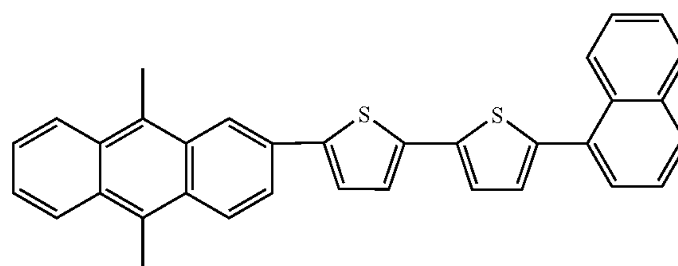
Compound 63
