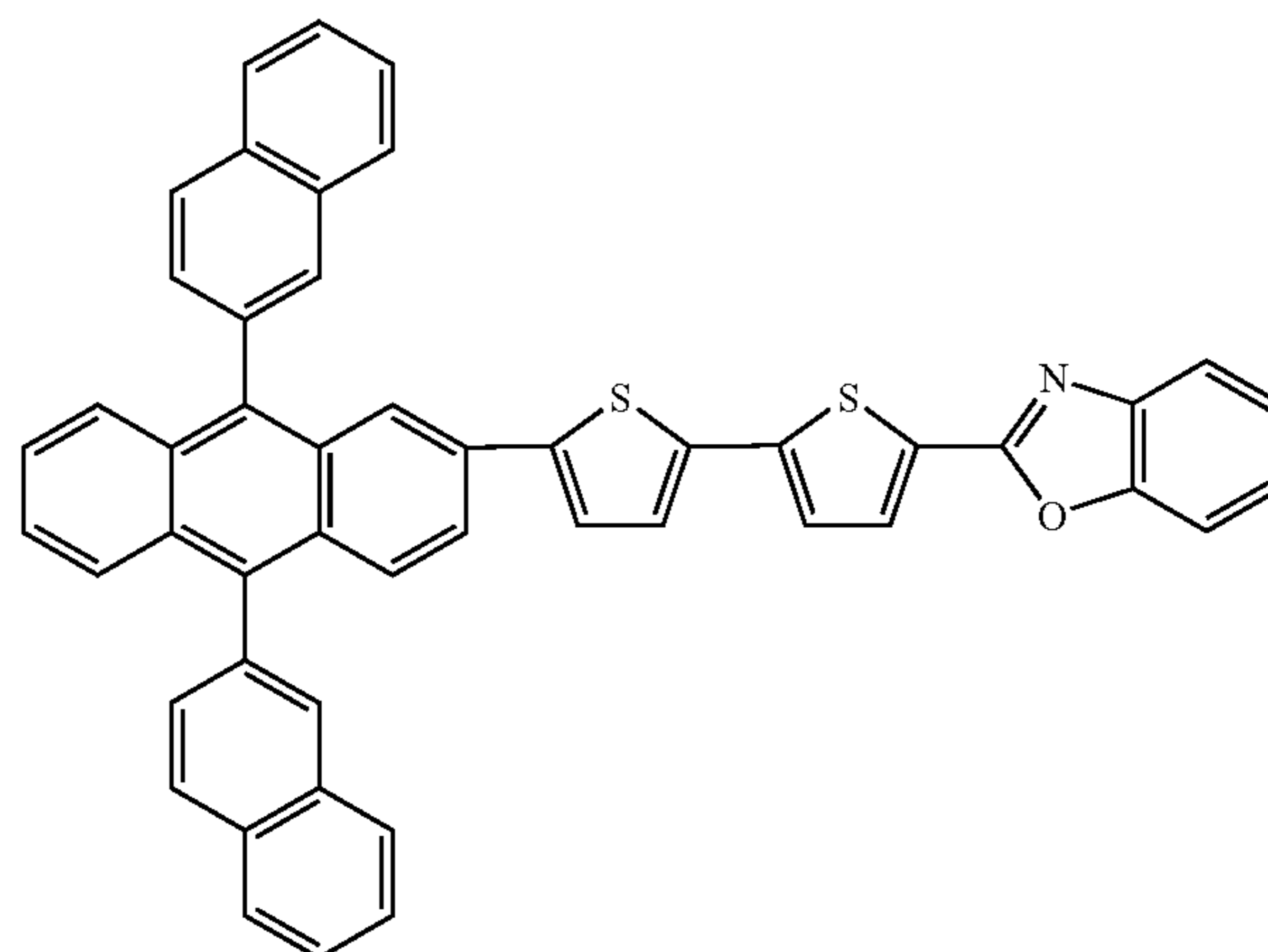
Compound 28
