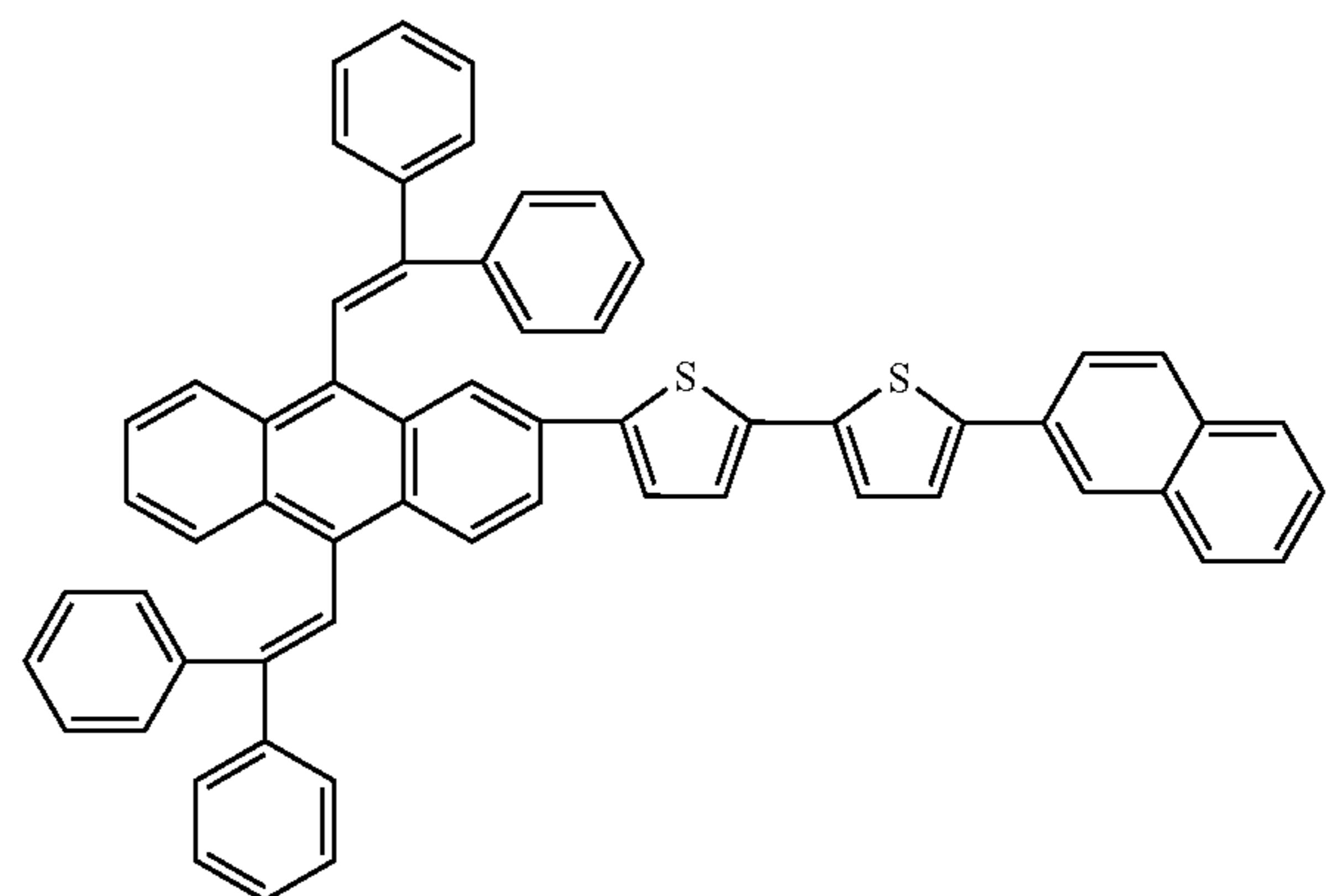
Compound 41
