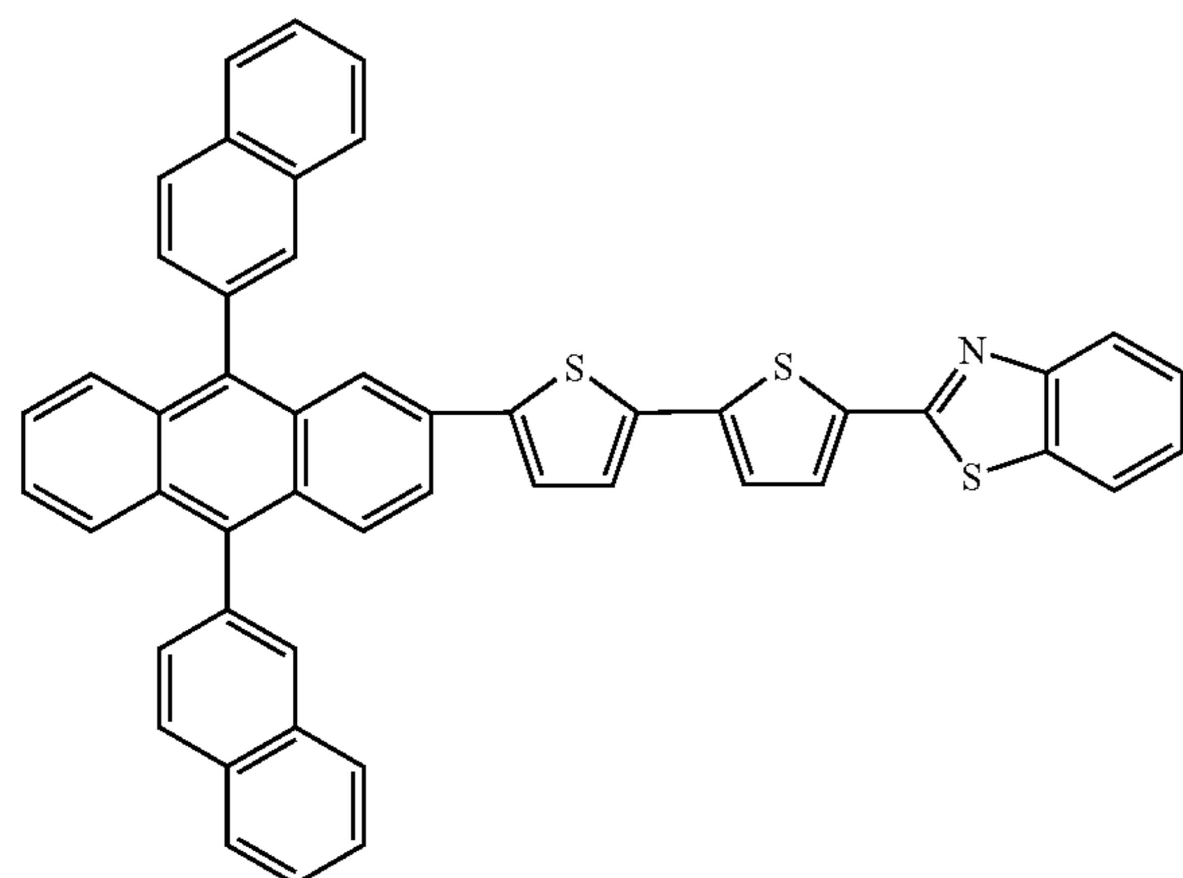
Compound 27
