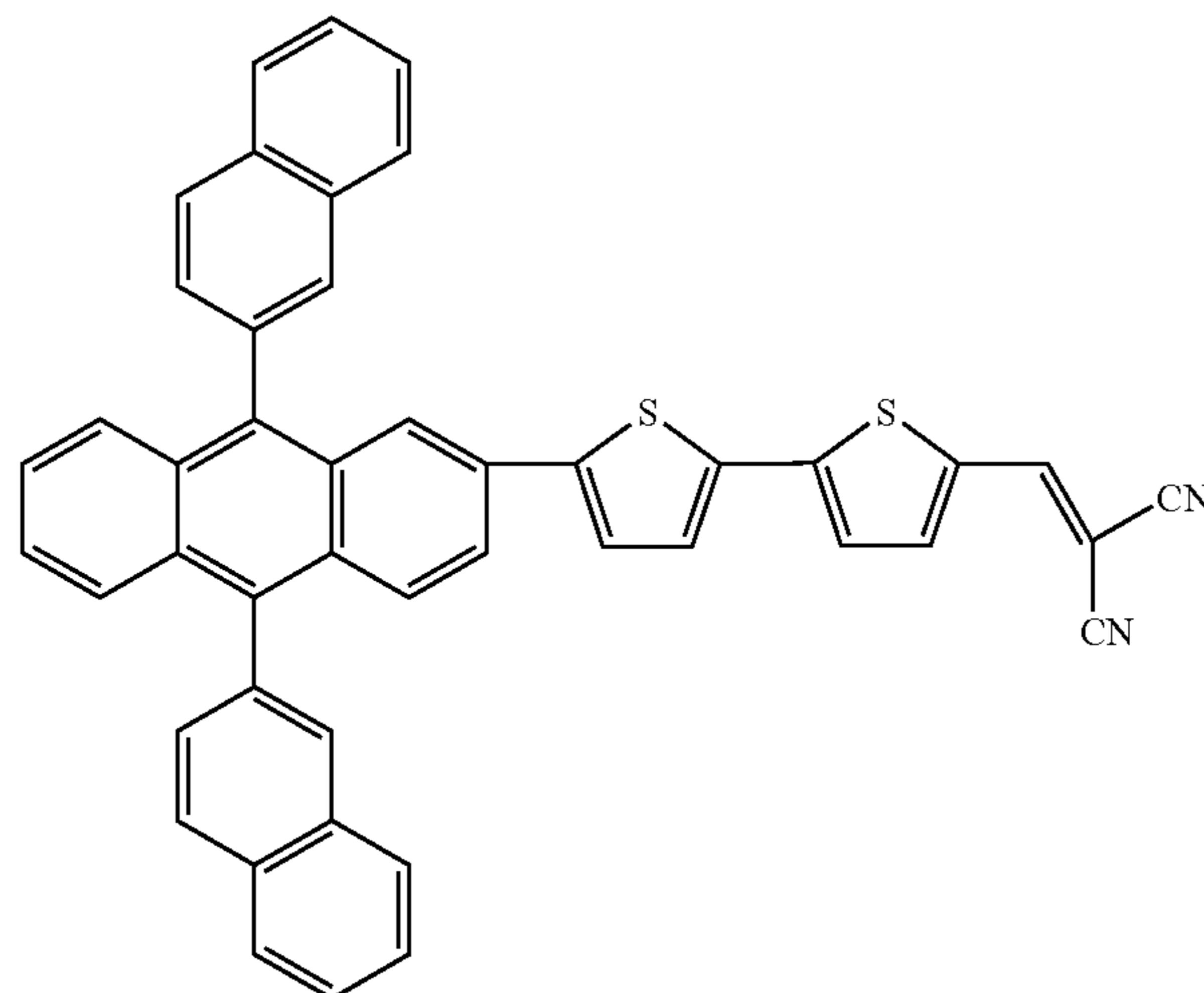
Compound 26
