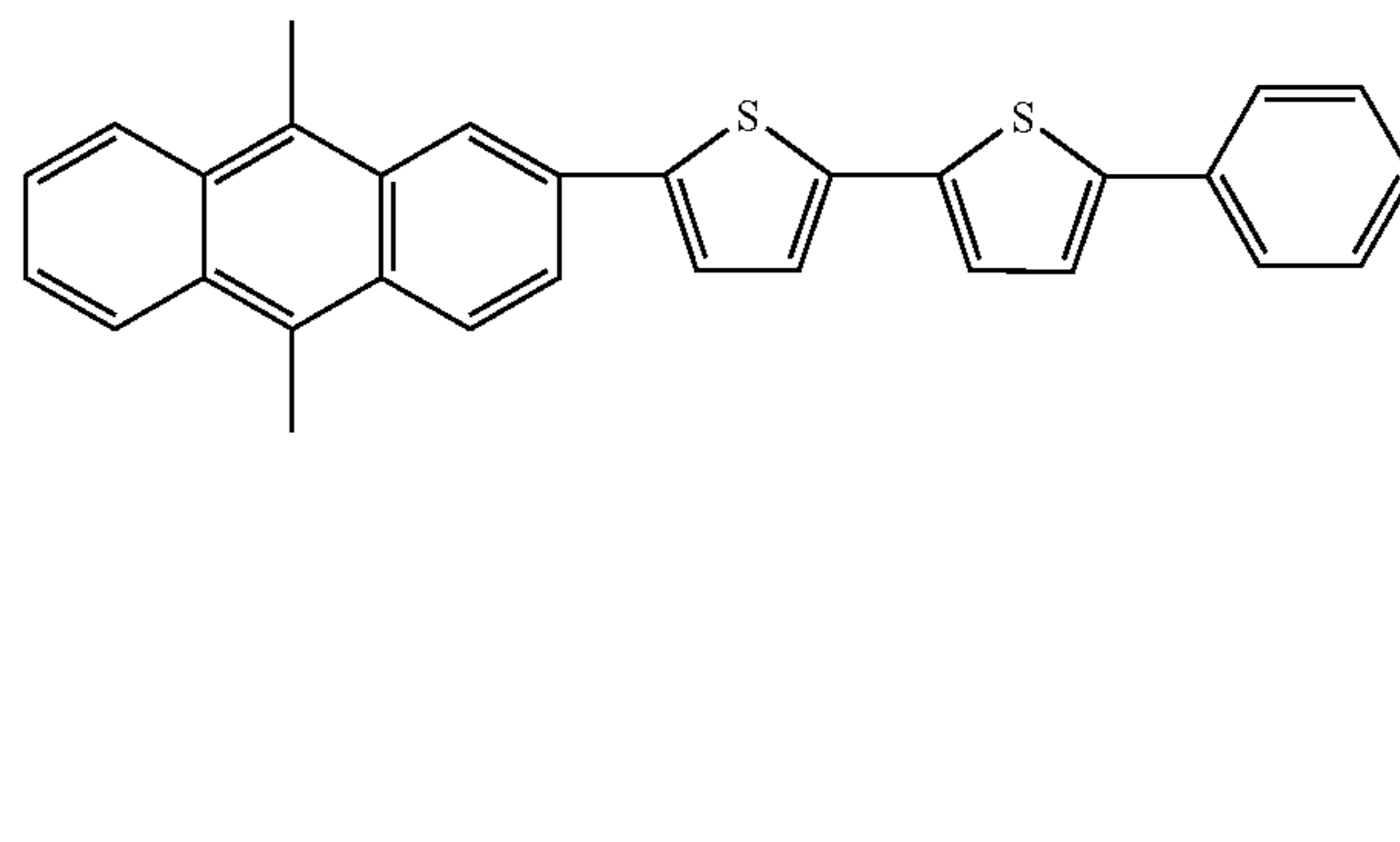
Compound 63
