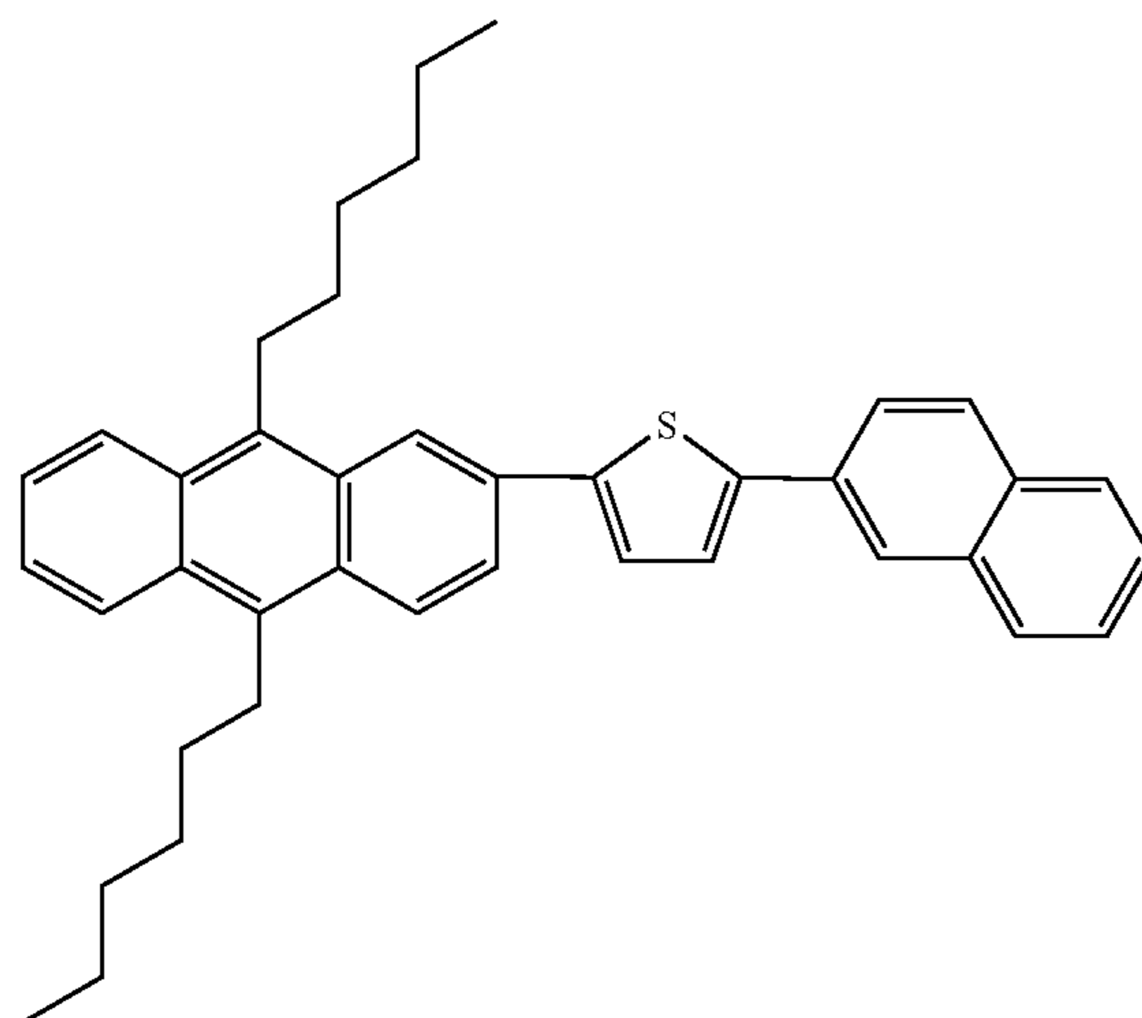
Compound 95
