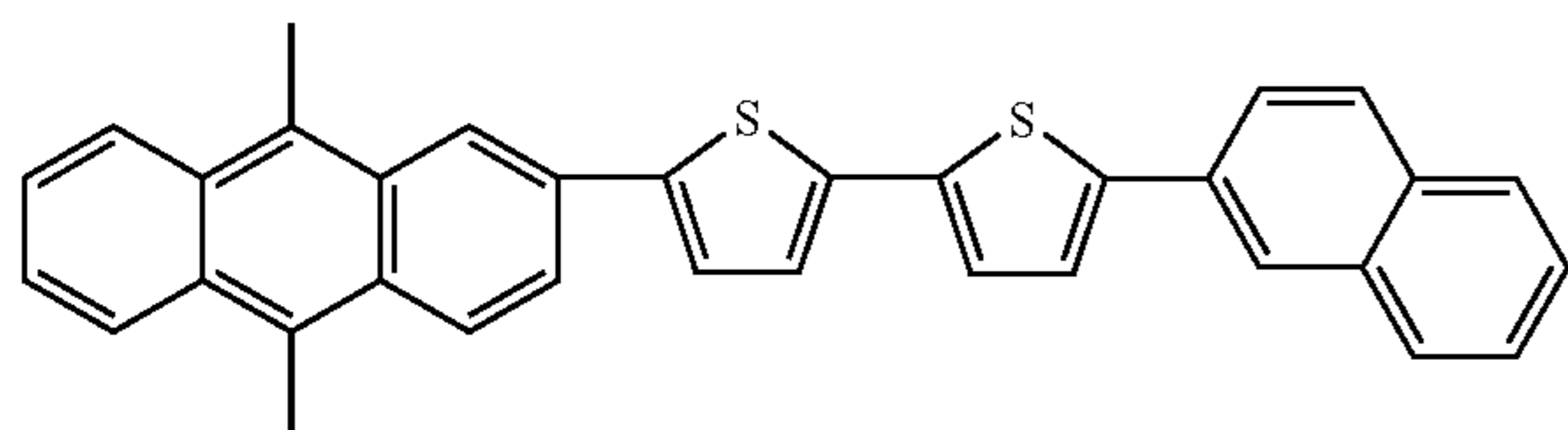
Compound 62
