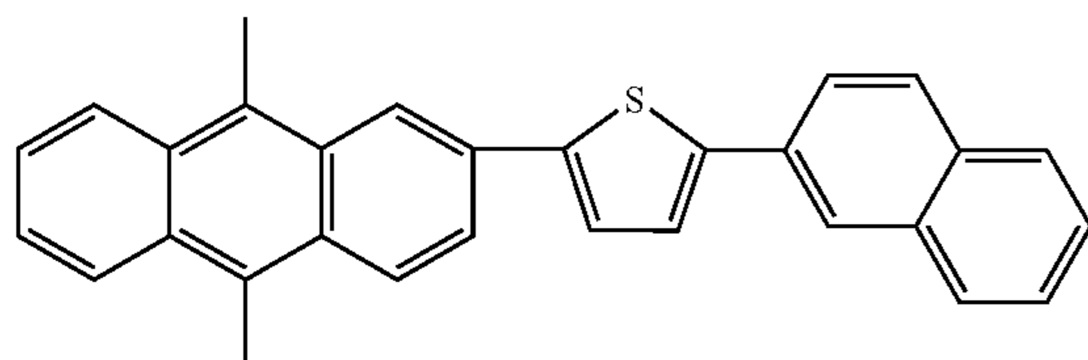
Compound 68
