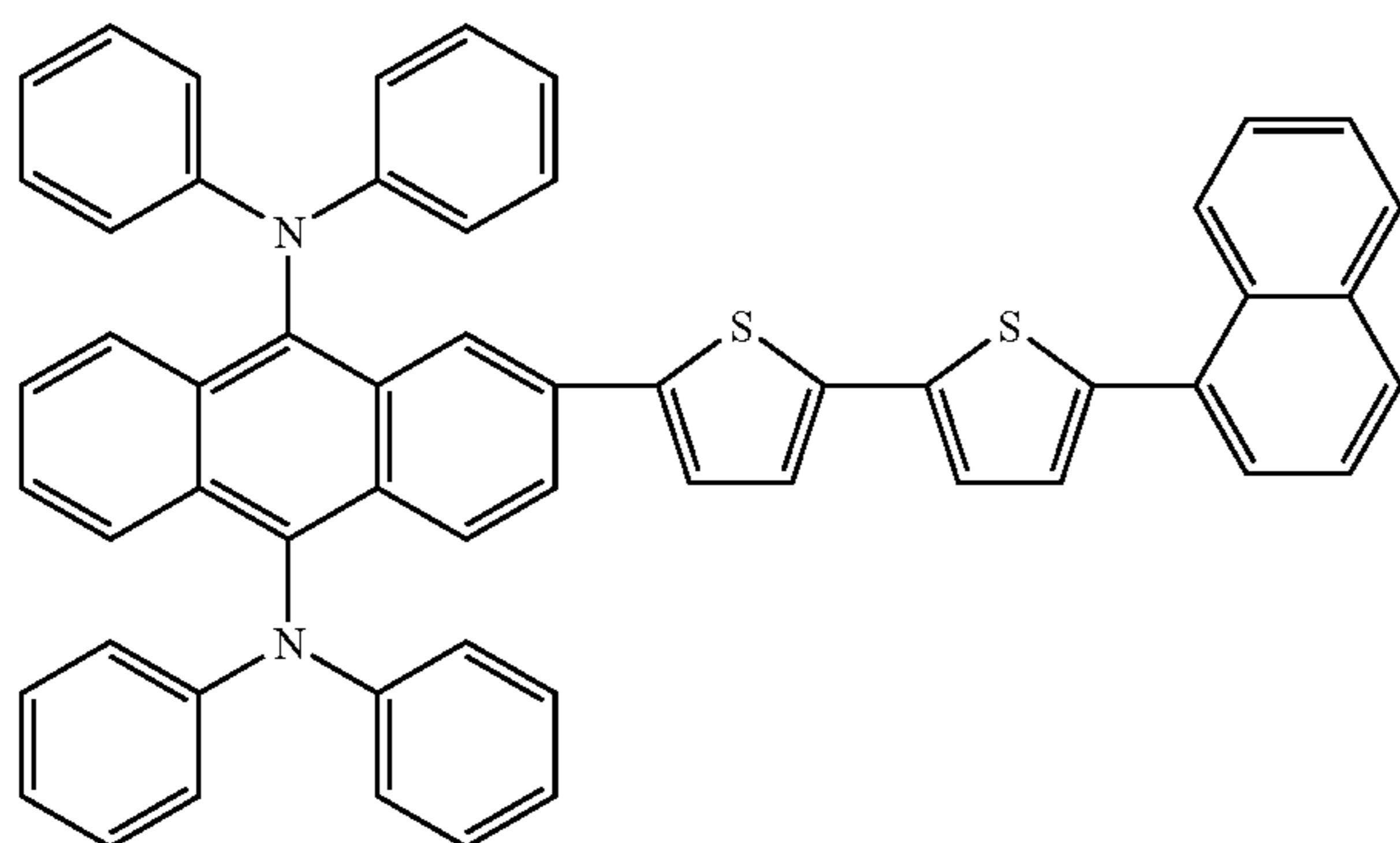
Compound 50
