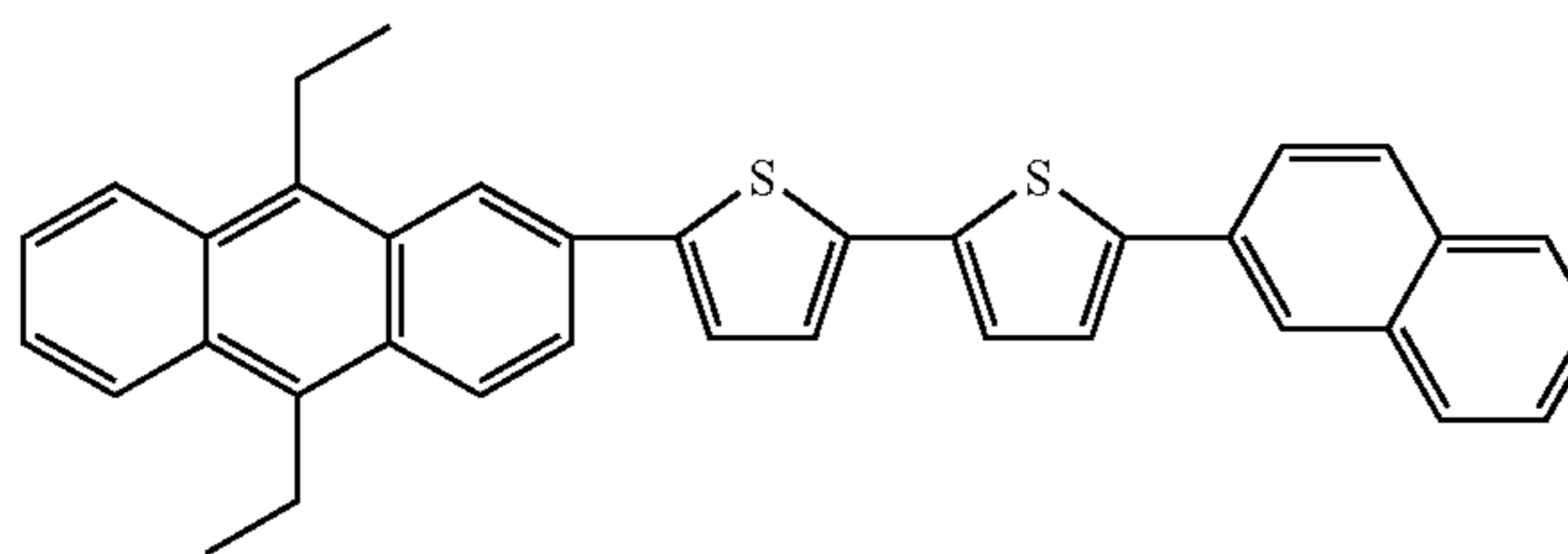
Compound 63
