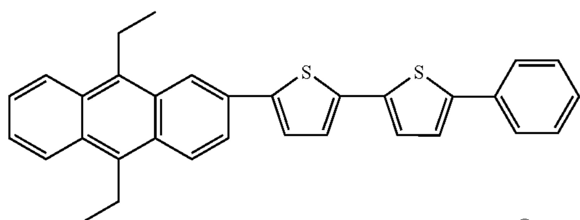
Compound 66
