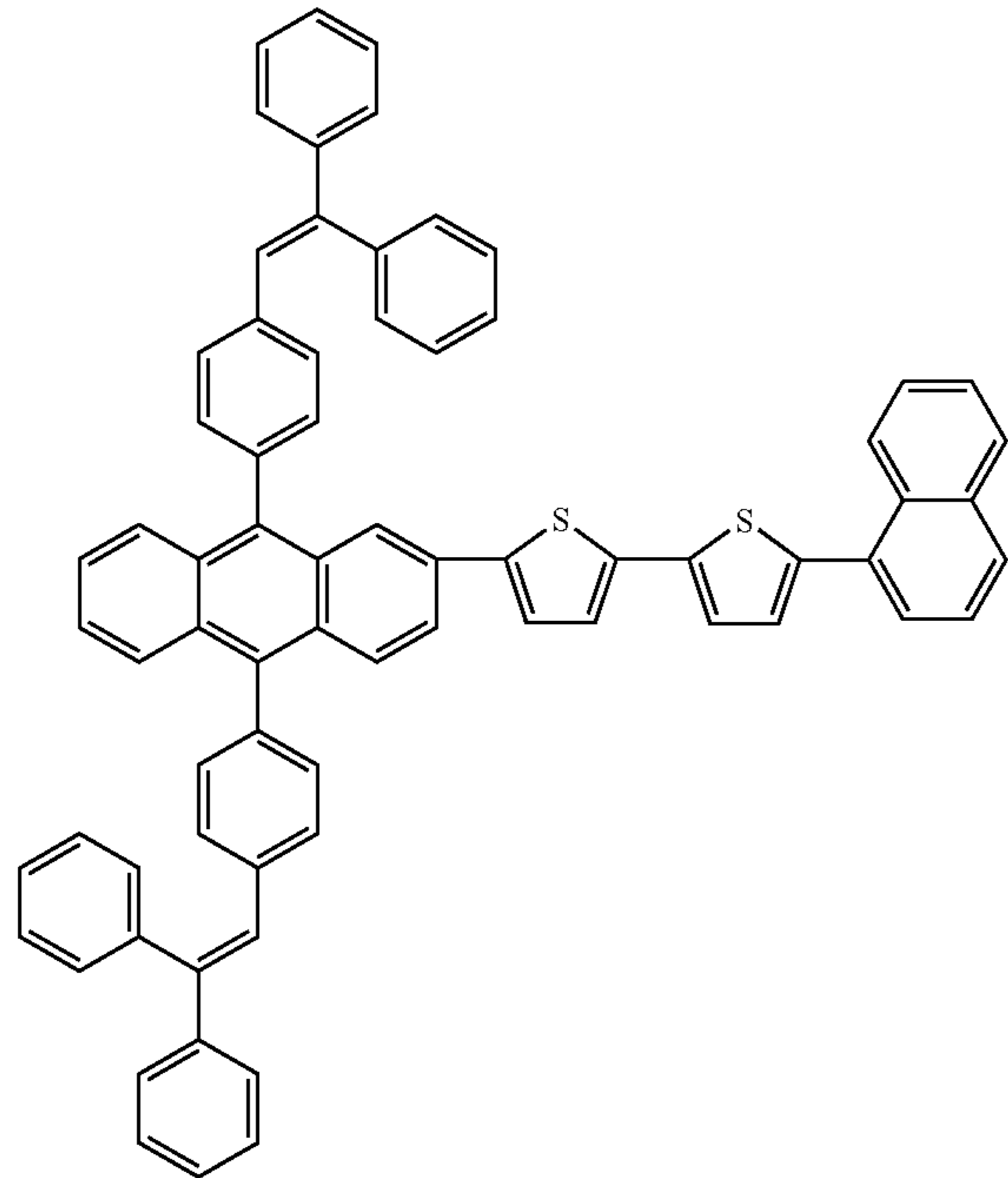
Compound 39
