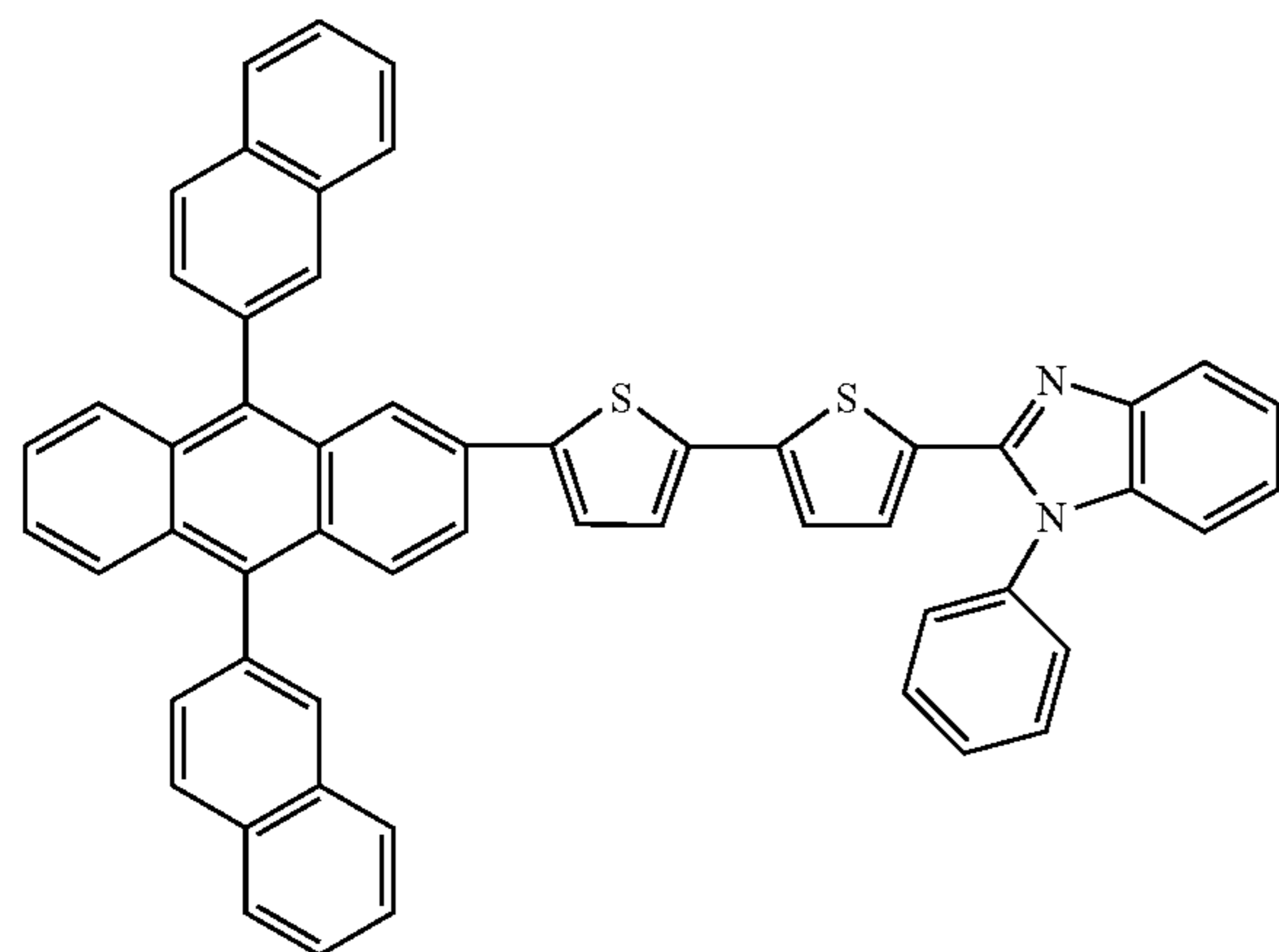
Compound 29
