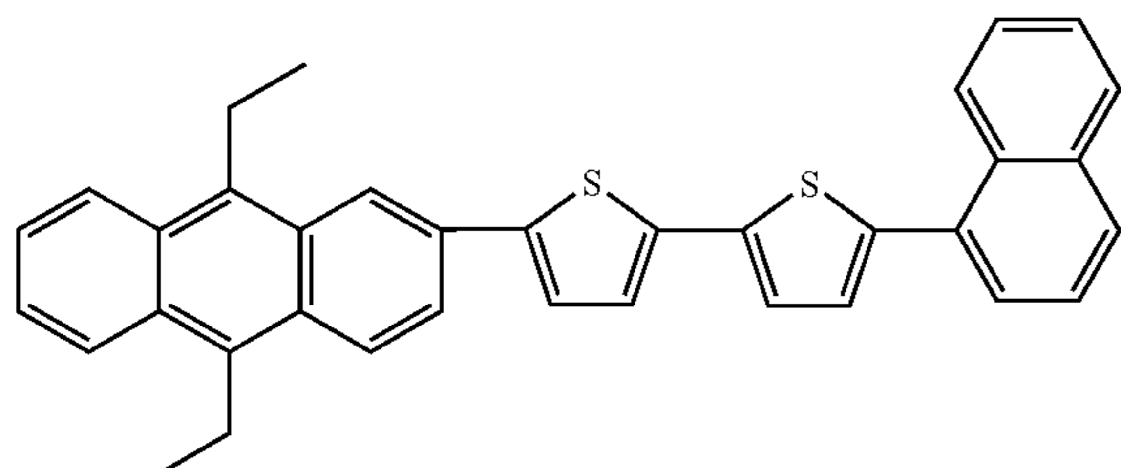
Compound 68
