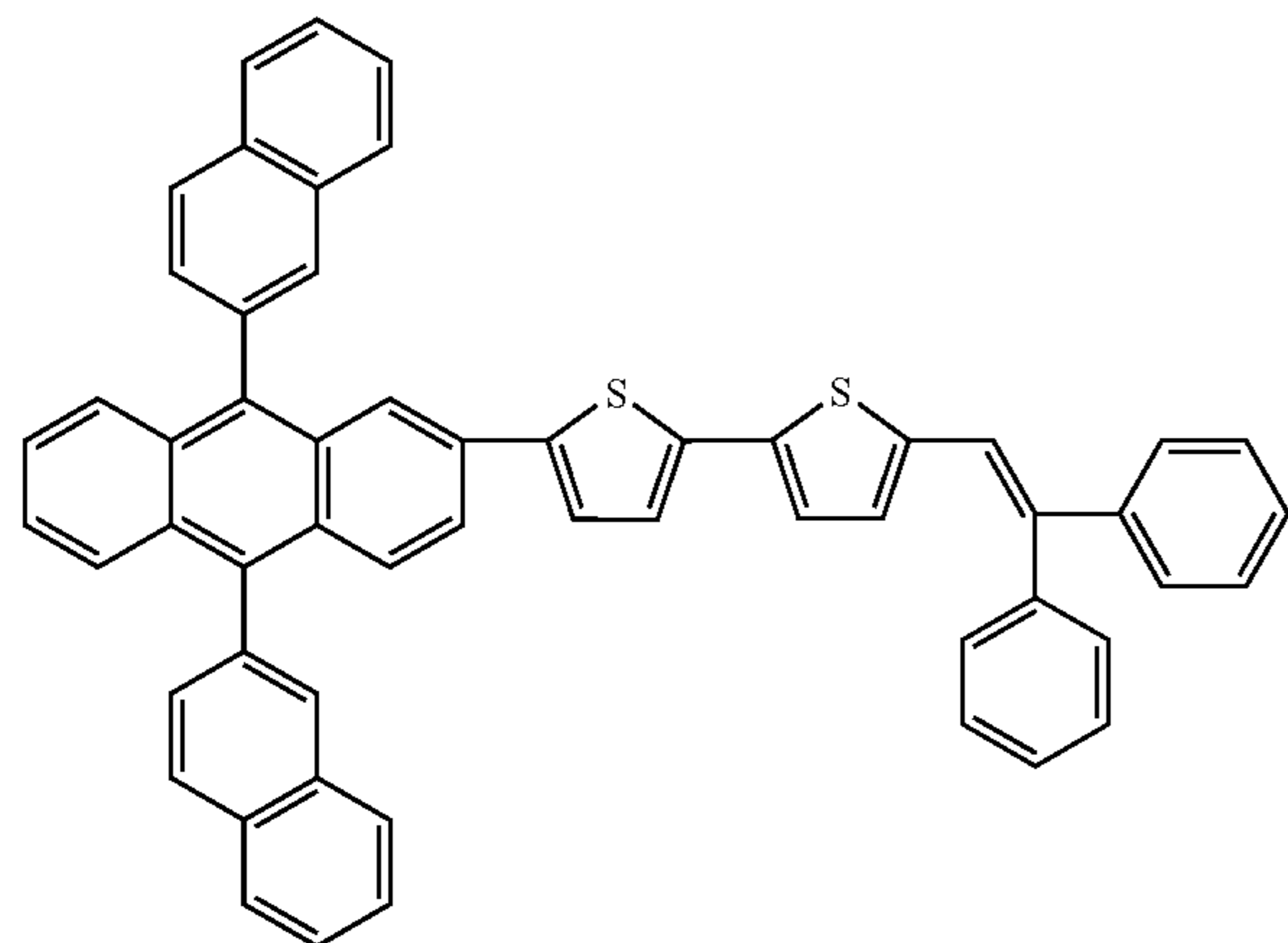
Compound 25
