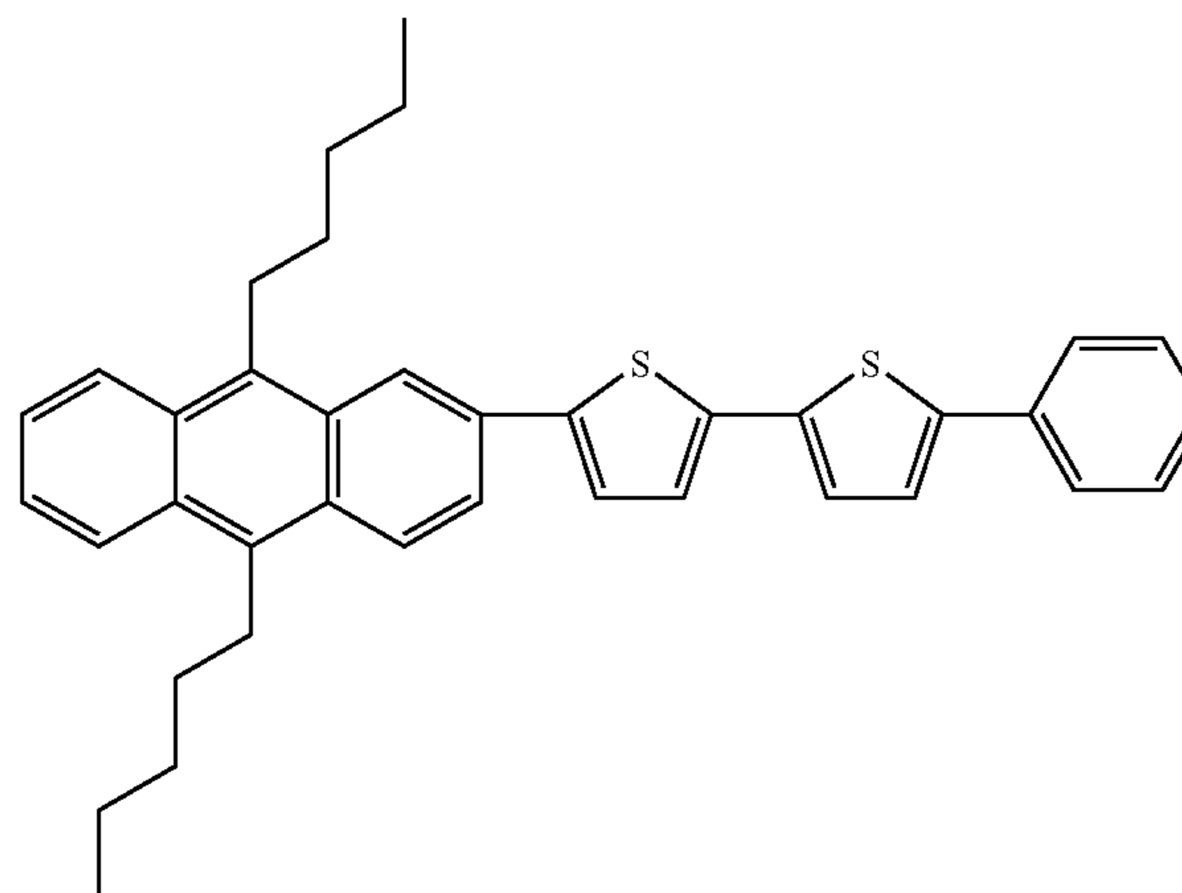
Compound 81
