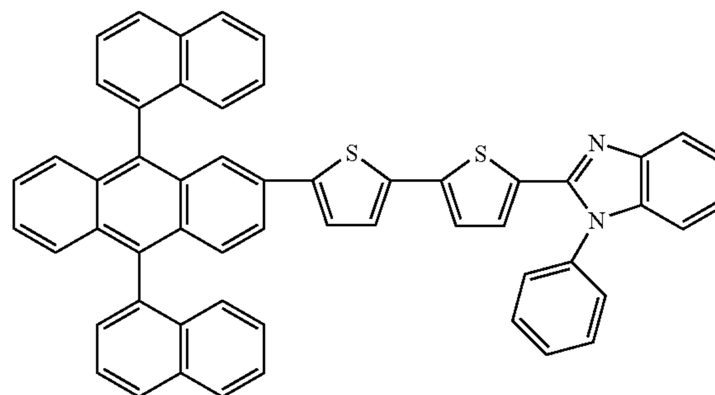
Compound 30
