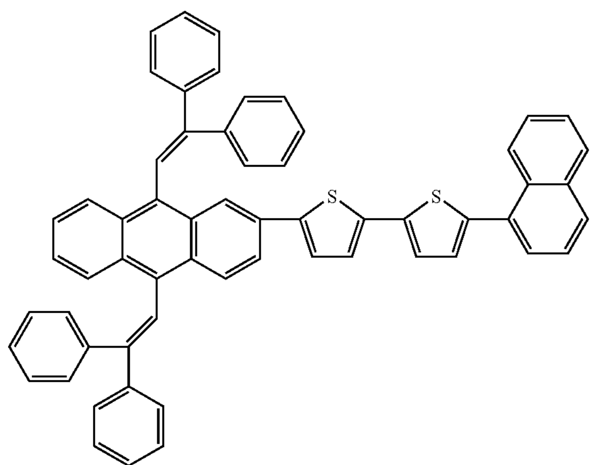
Compound 38
