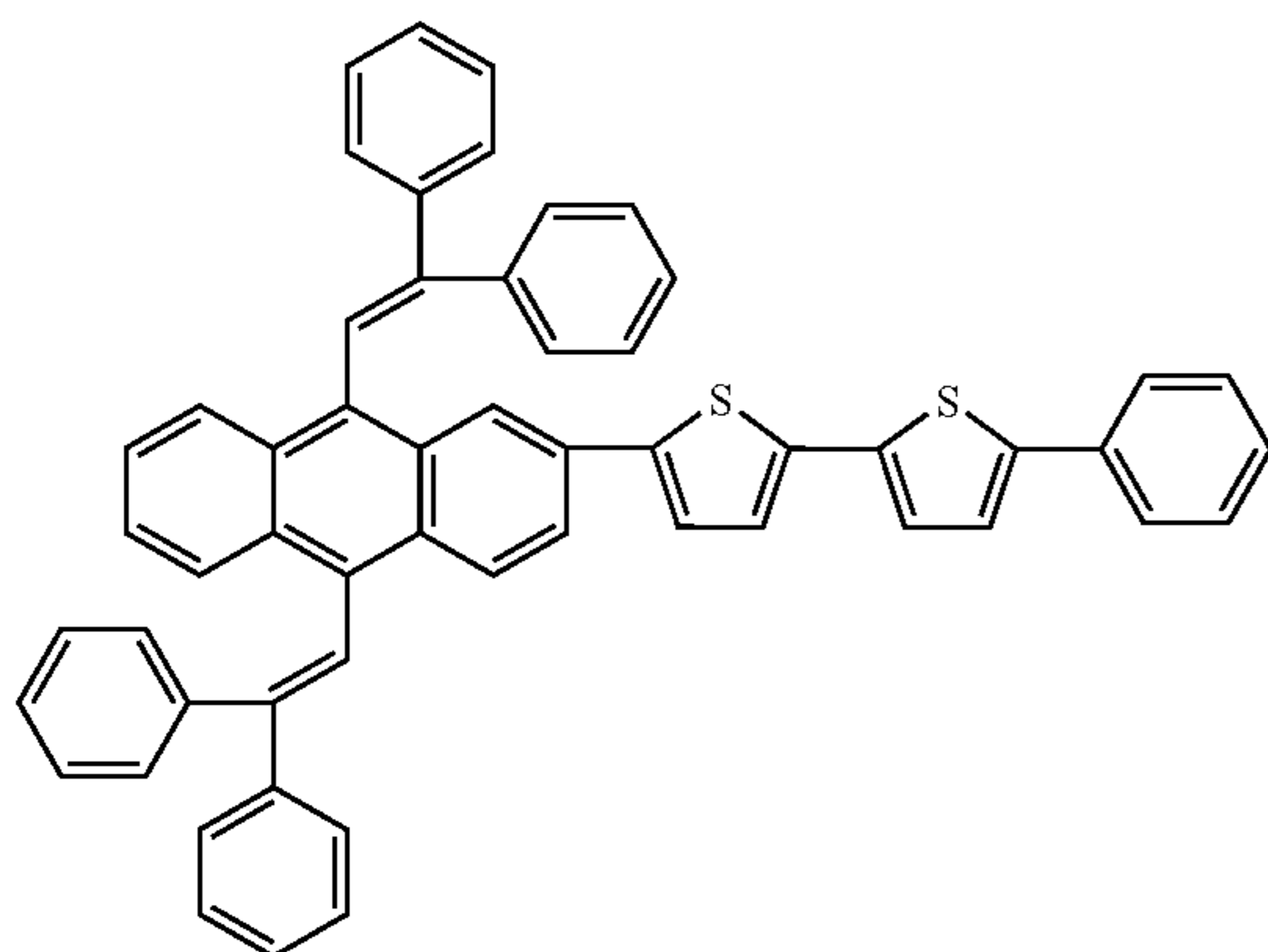
Compound 40
