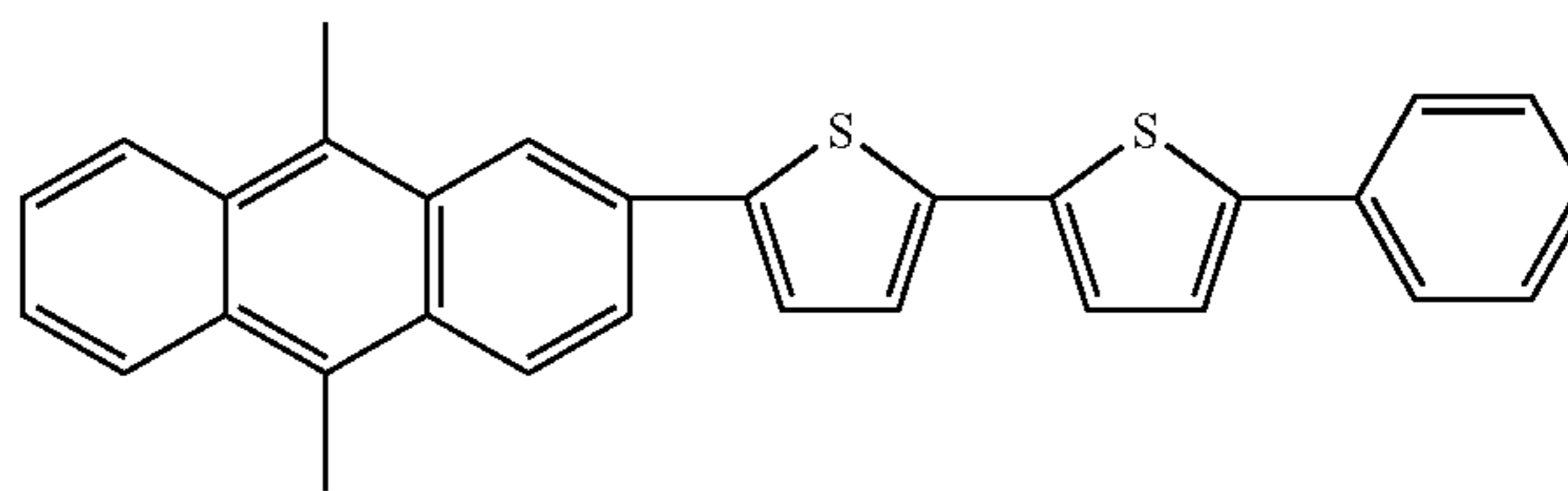
Compound 57
