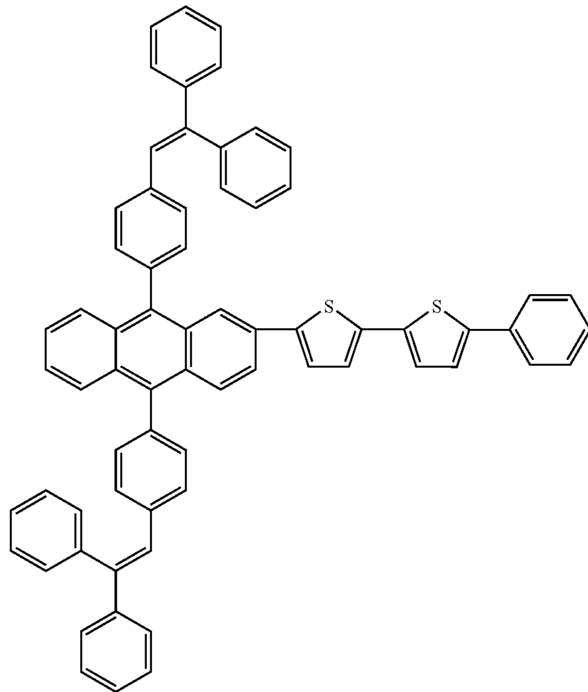
Compound 37
