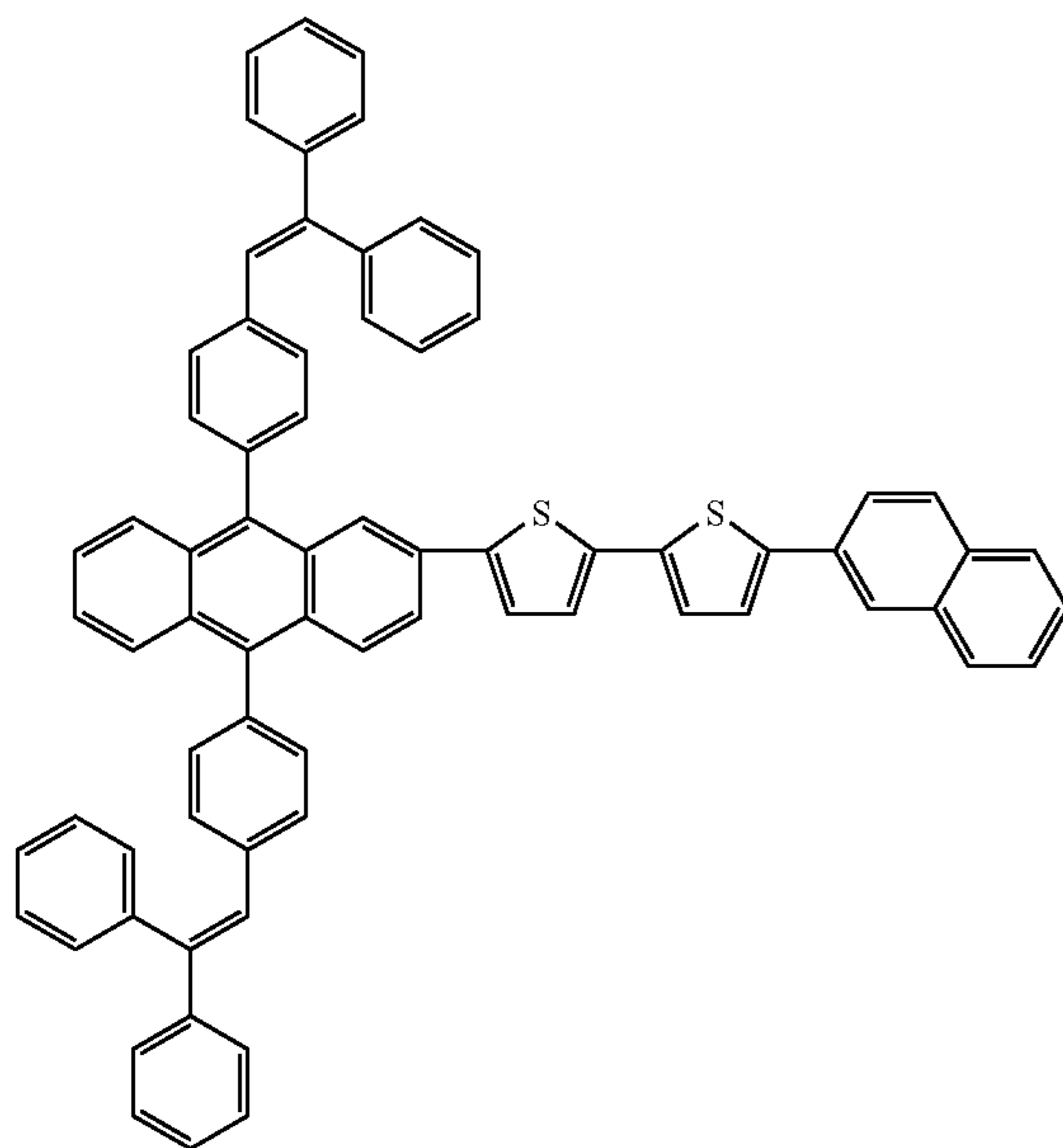
Compound 36
