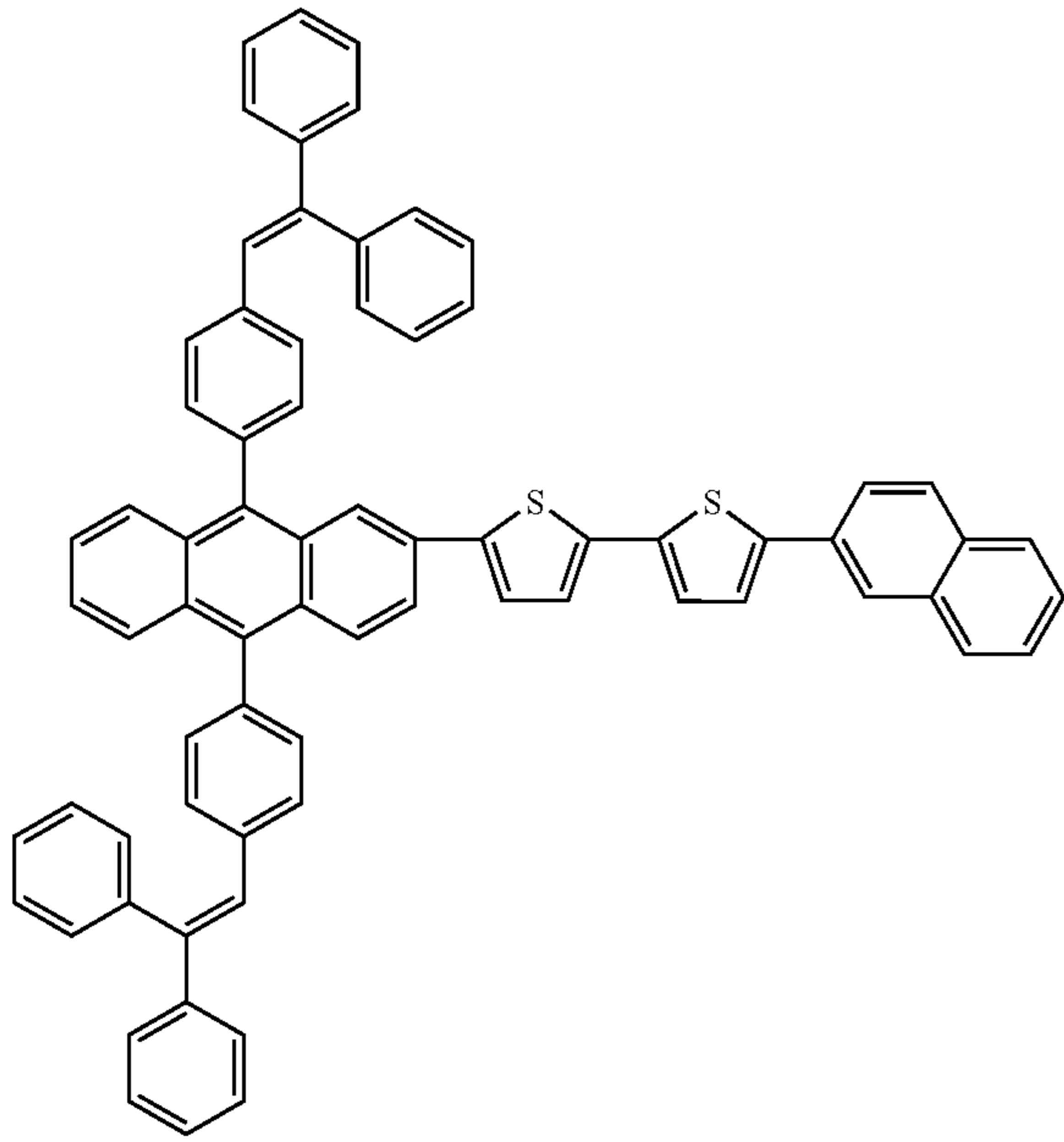
Compound 38
