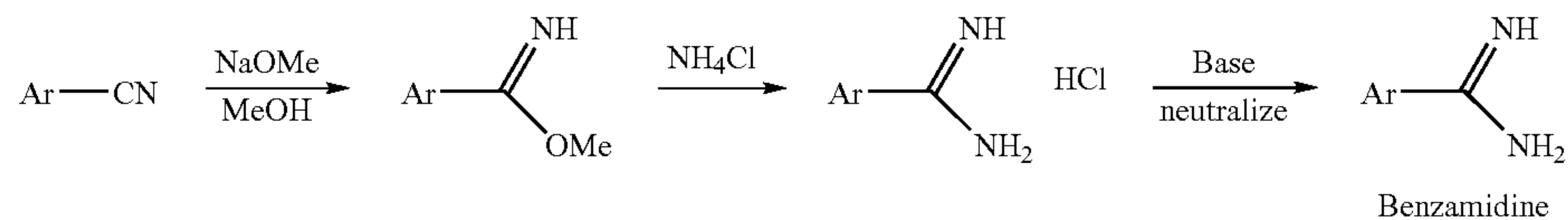
Scheme 8
