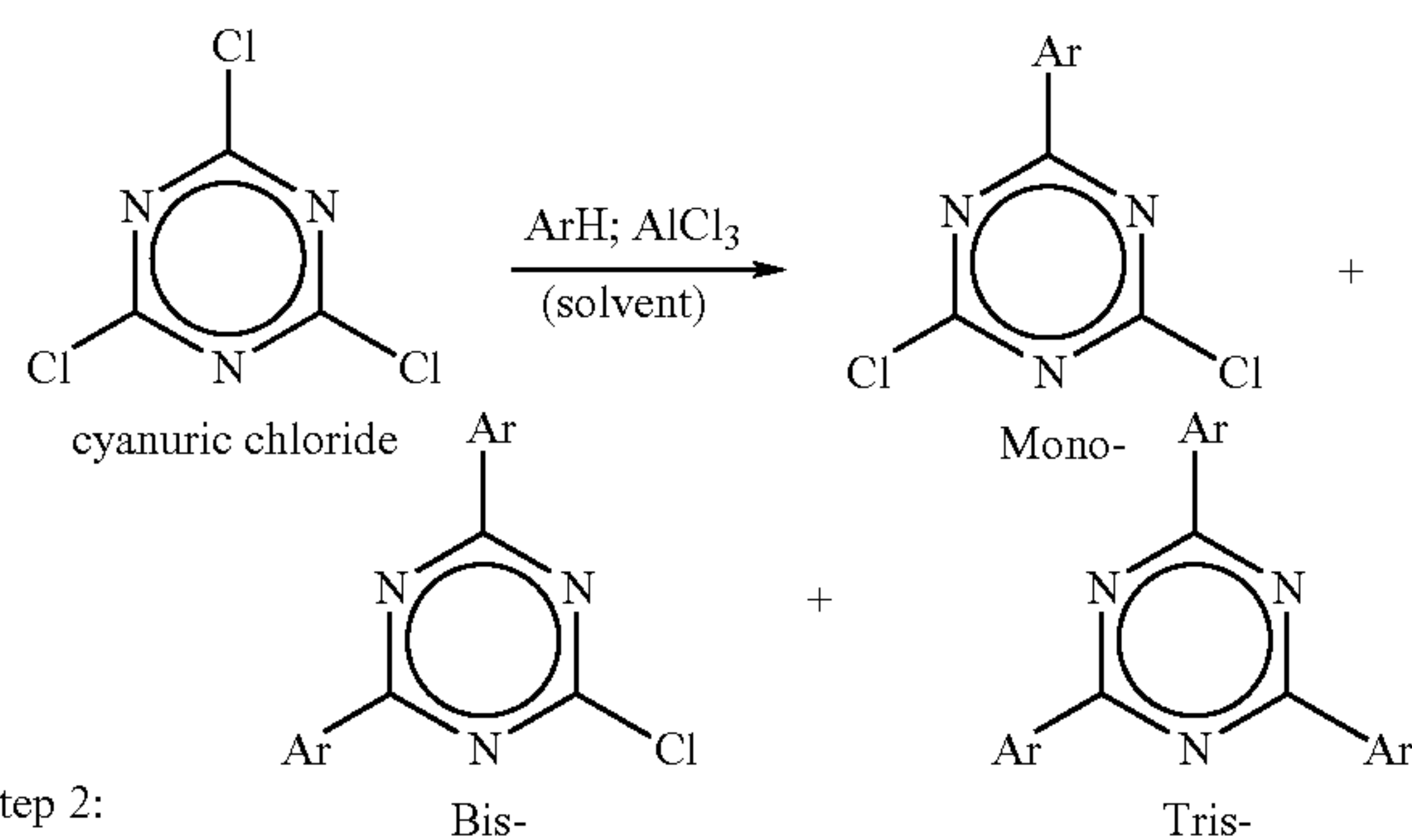
Scheme 1
