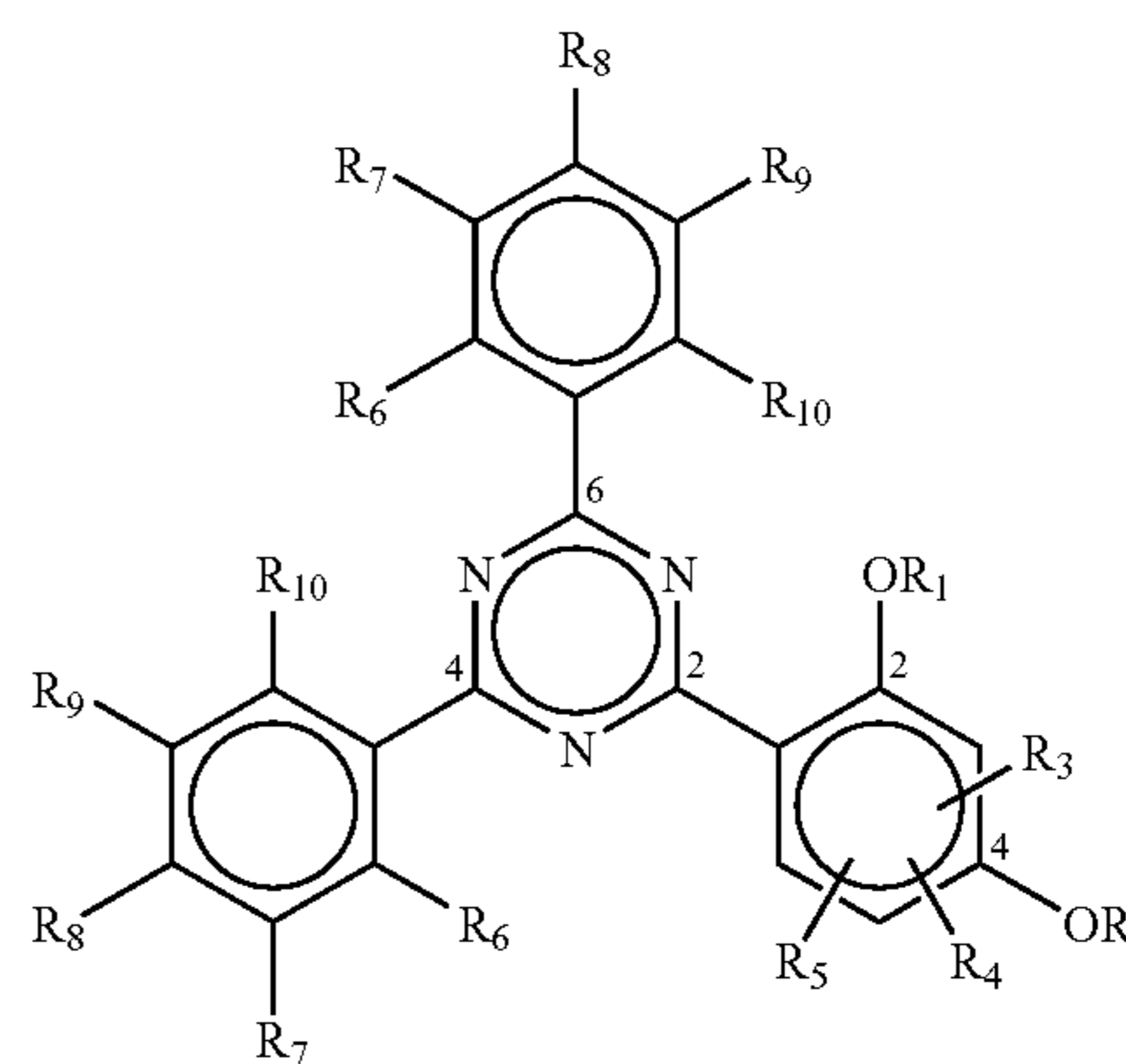
R_1 = \text{H} or a blocking group 2-(2-oxyaryl)-4,6-bisaryl-1,3,5-triazine UV absorbers
