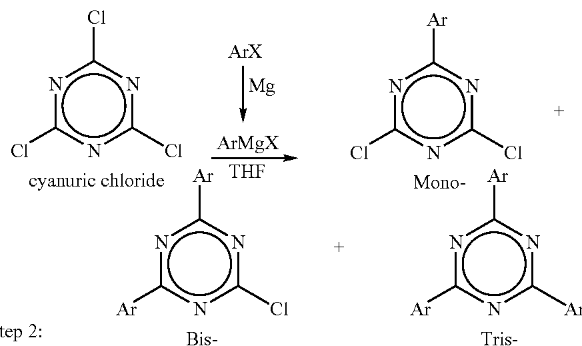
Scheme 2
