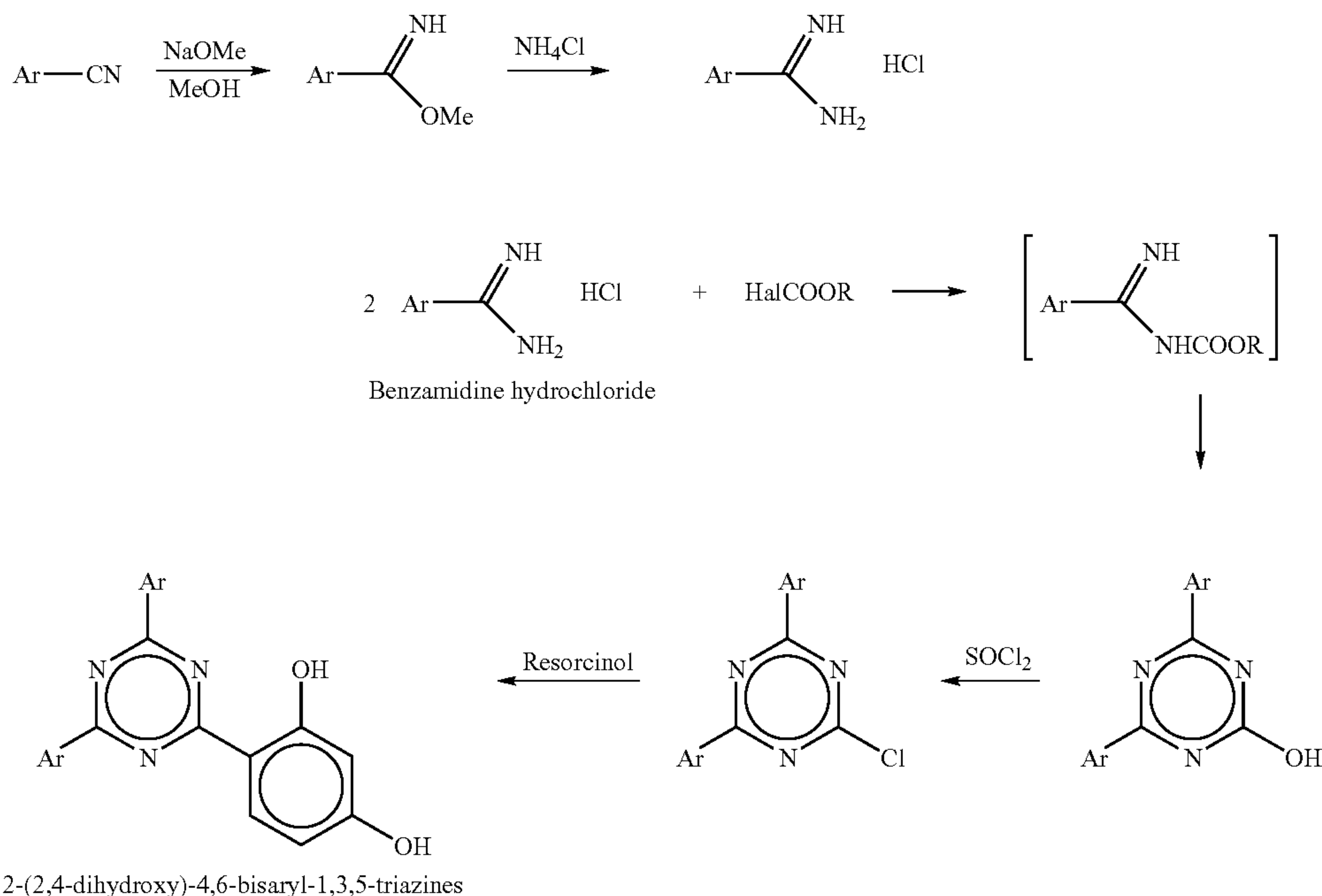
Scheme 5
