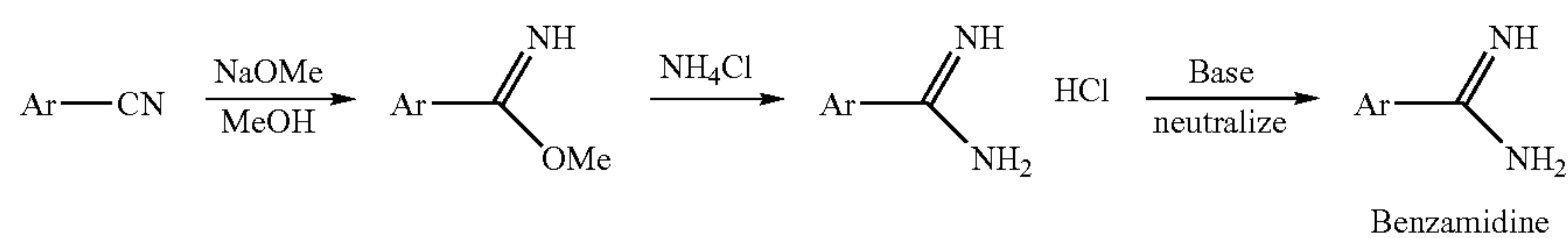
Scheme 6
