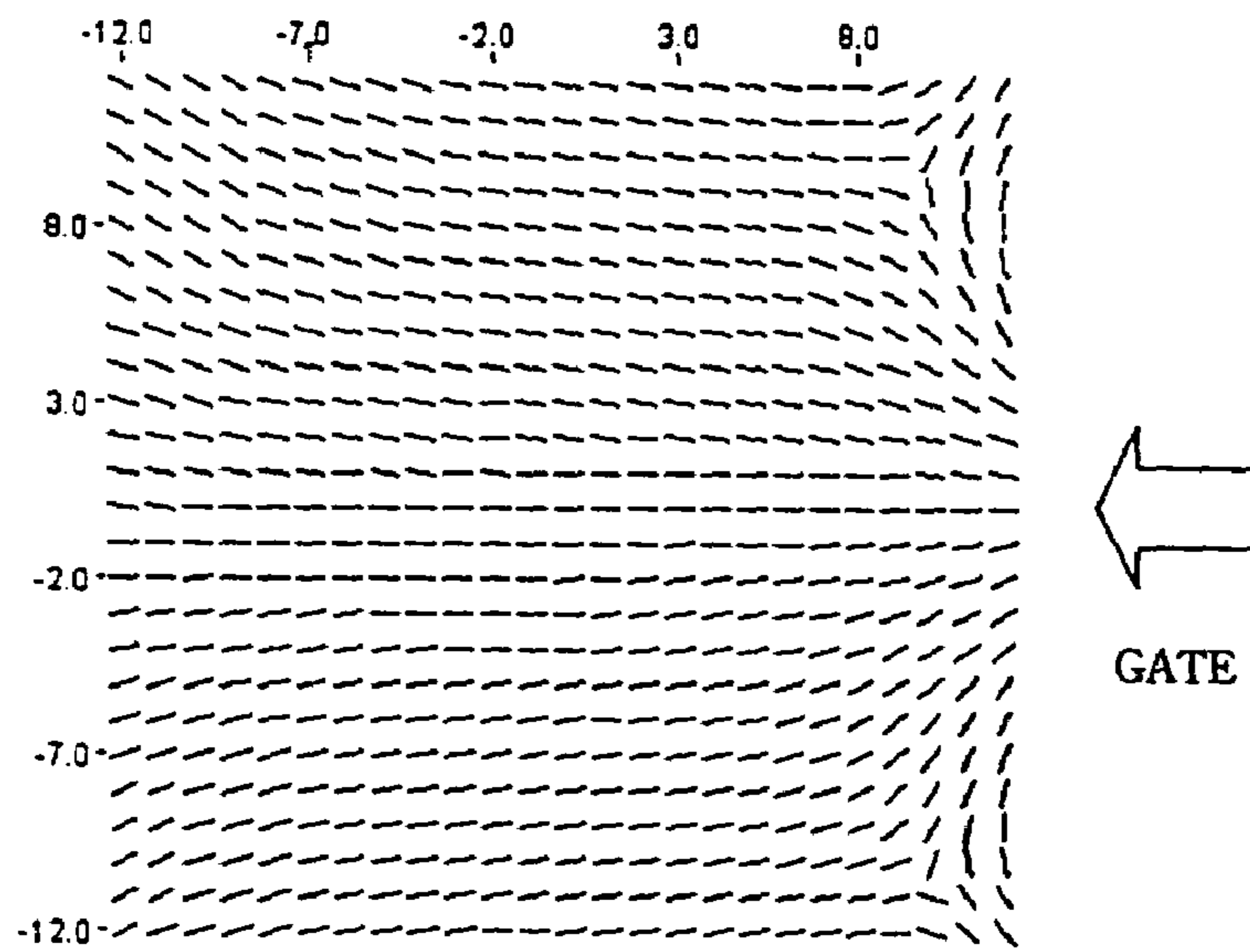
(a) POLYMETHYL METHACRYLATE
