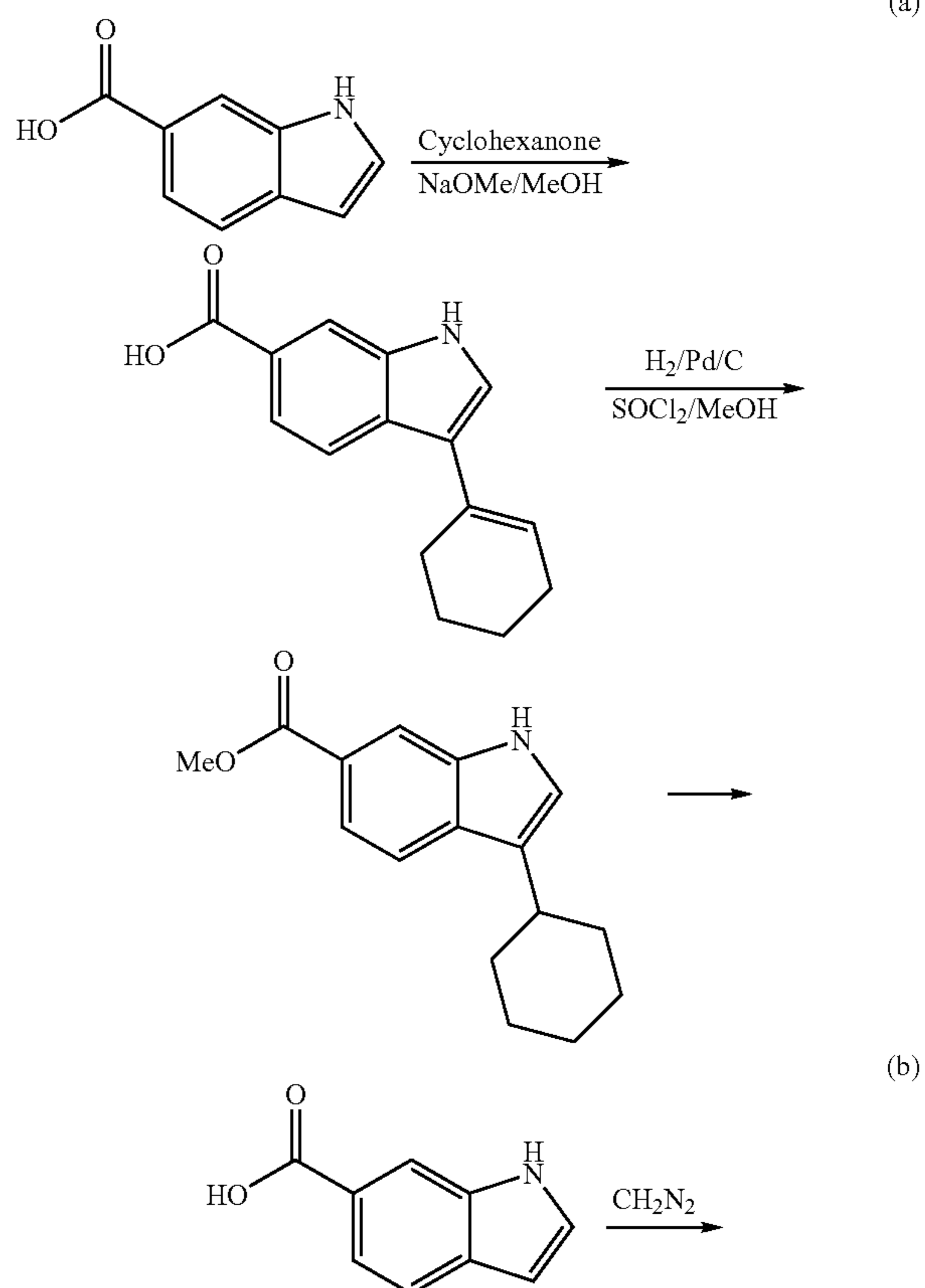
Scheme 1.
