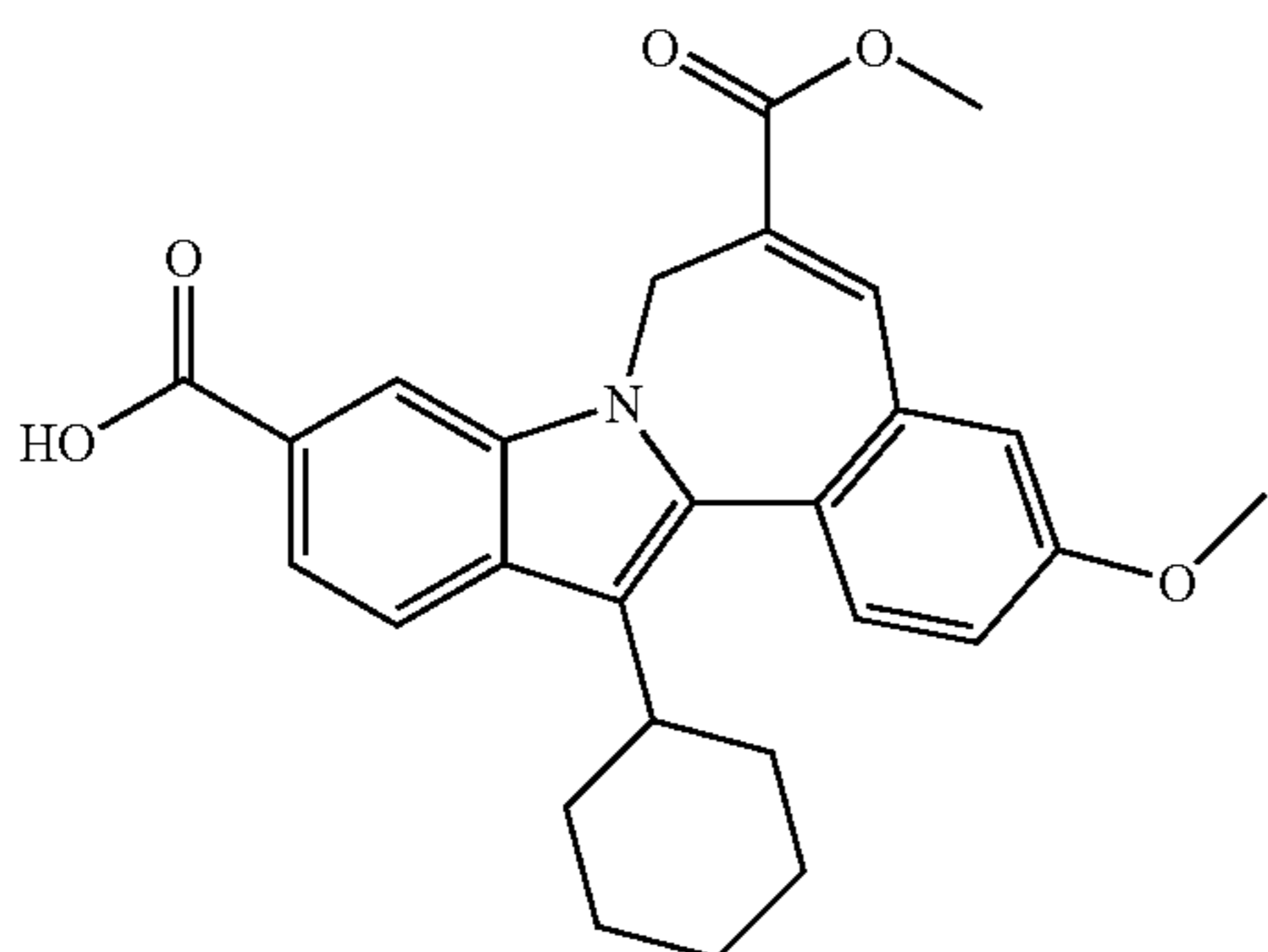
Intermediate 15
