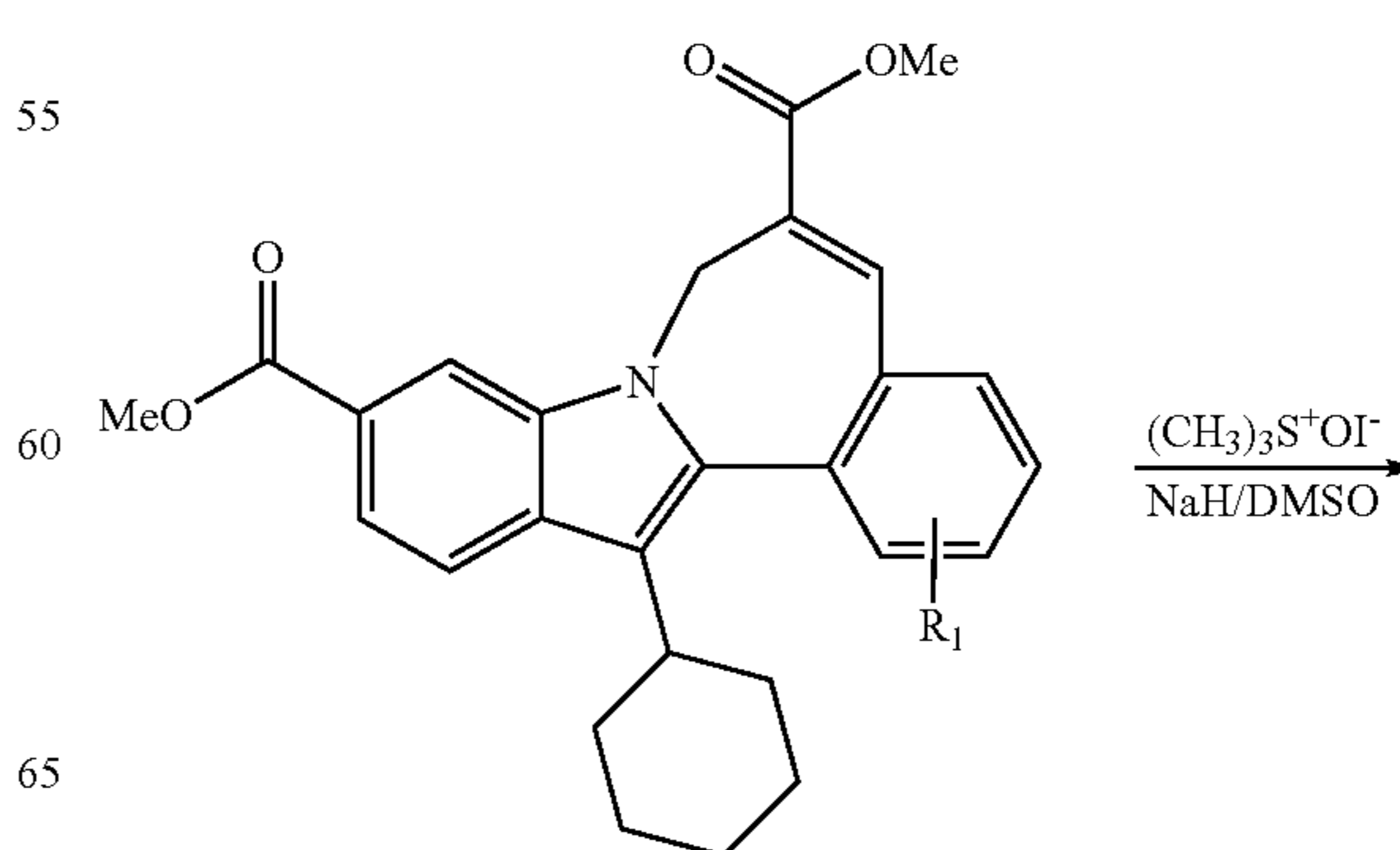
Scheme 2.
