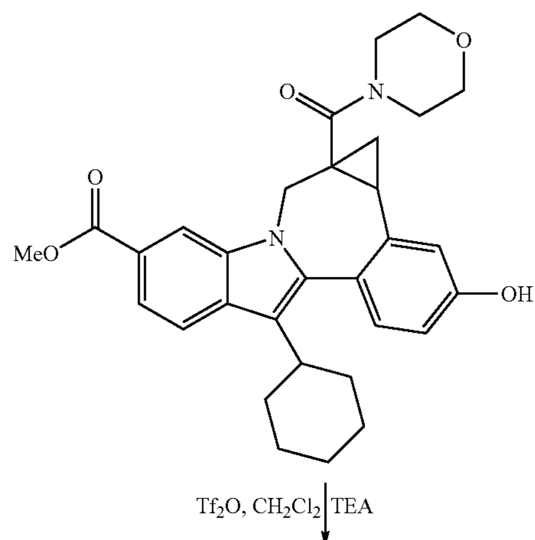
Scheme 10.
