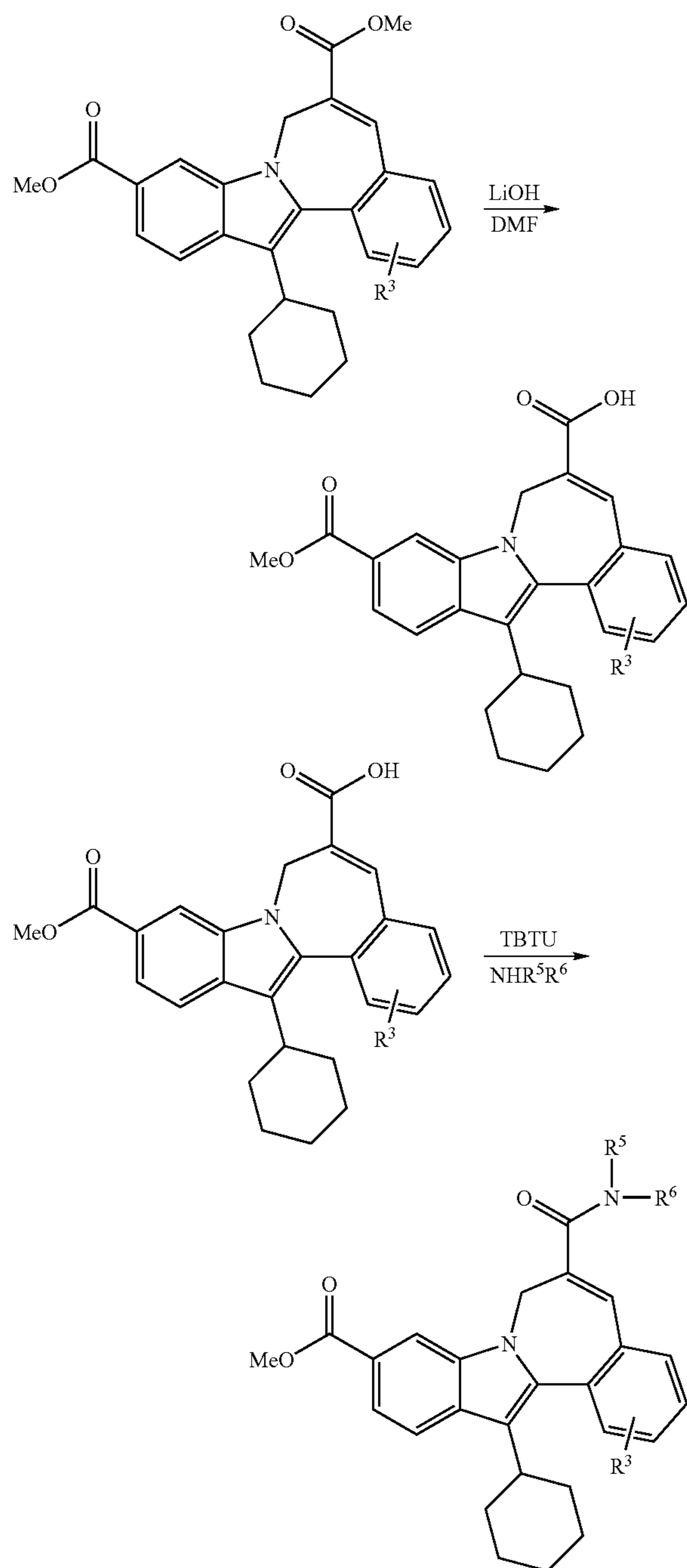
Scheme 3.
