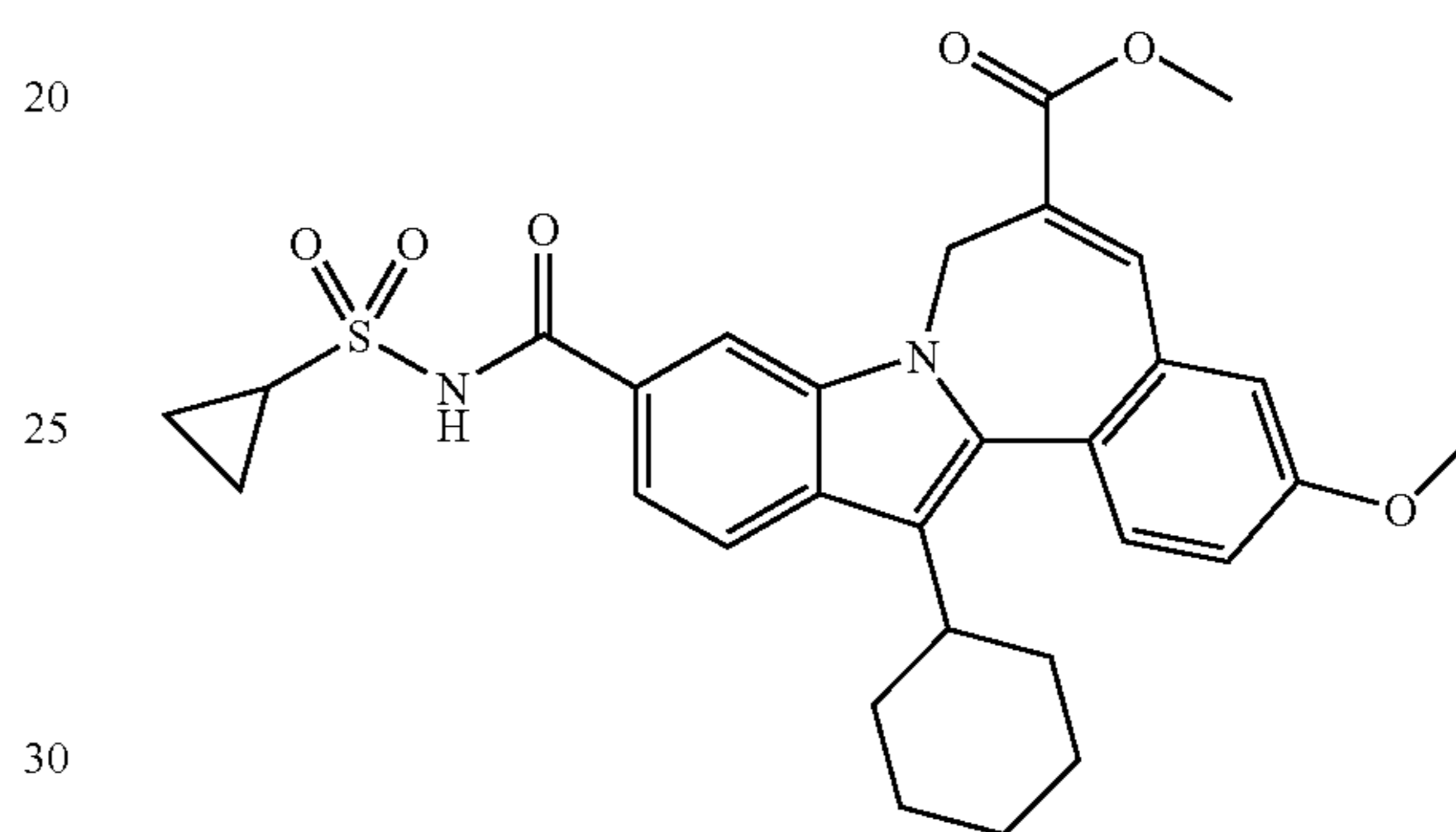
Intermediate 16
