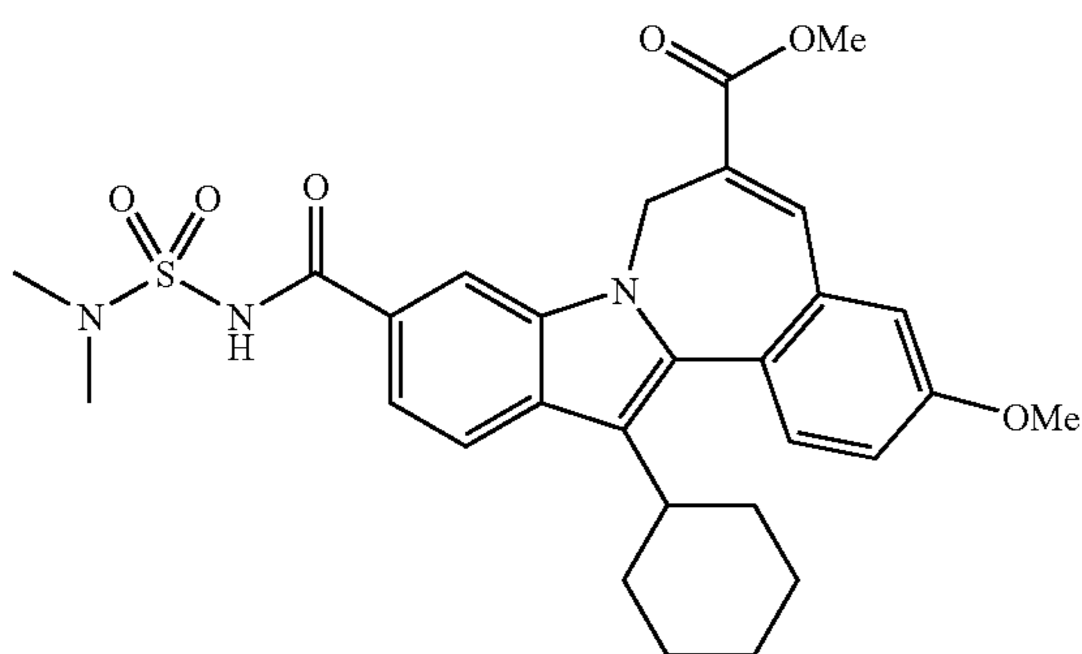
Intermediate 14
