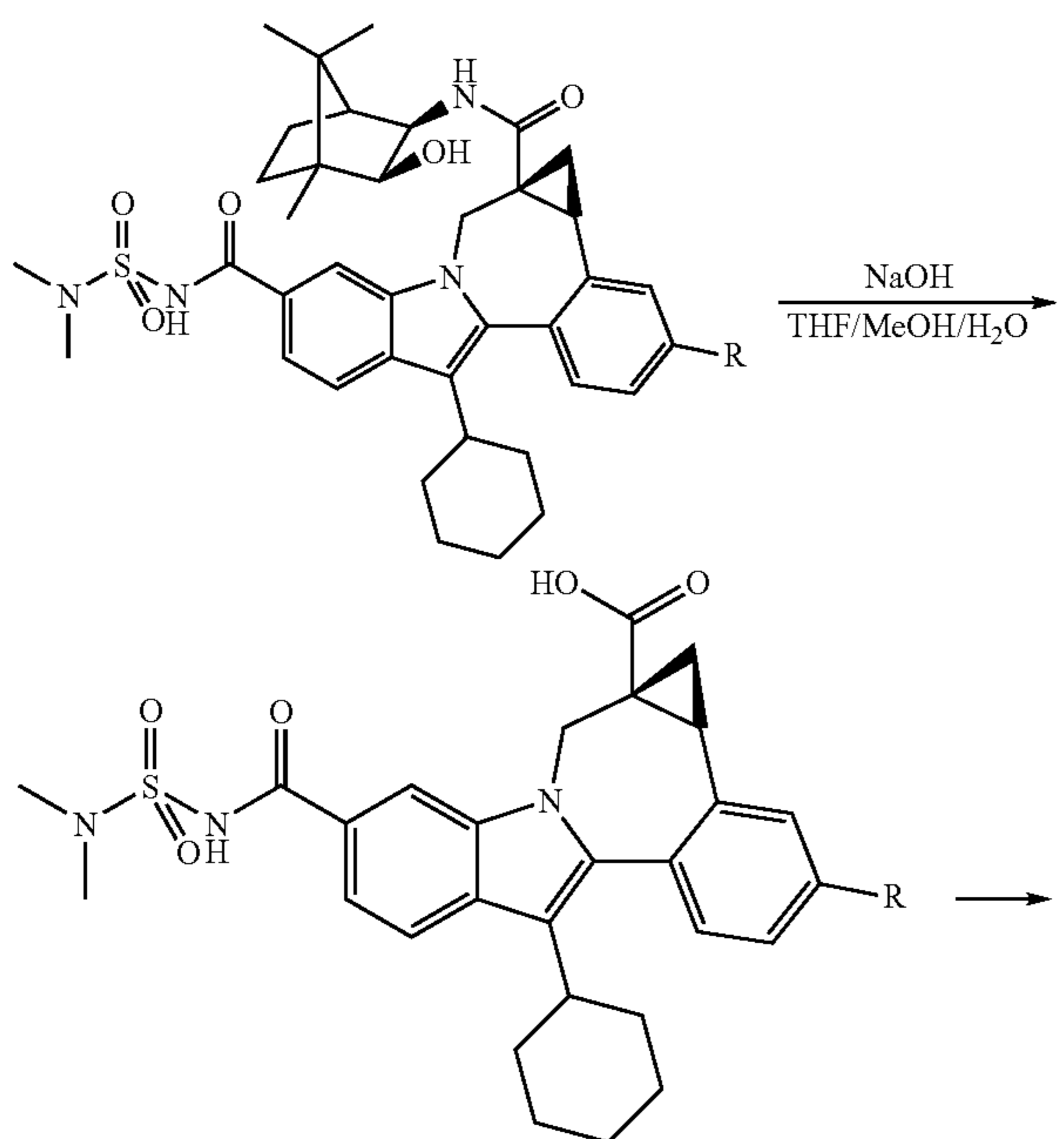
Scheme 8.
