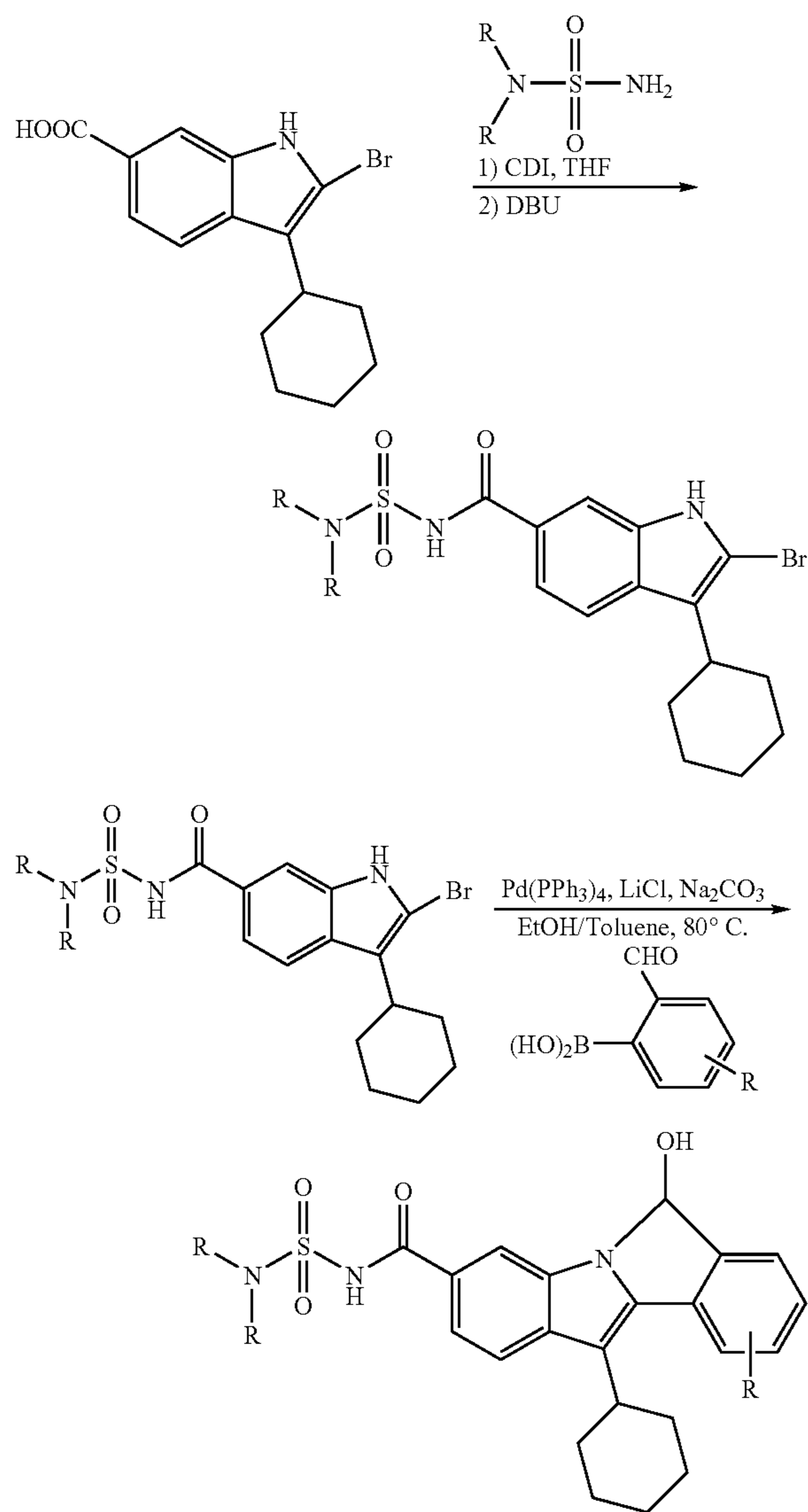
Scheme 4.
