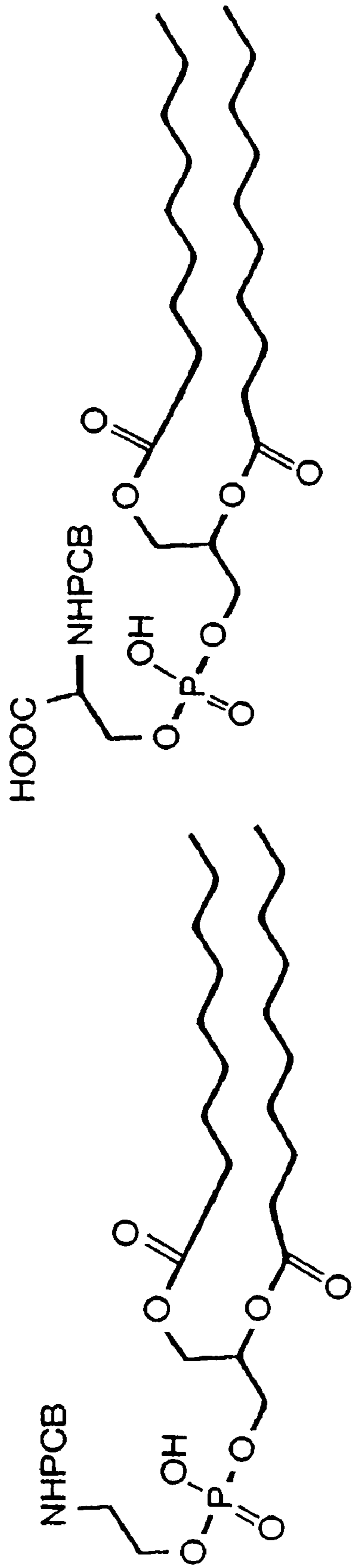
PCB-Phosphatidylethanoamine (PCB-PE)
