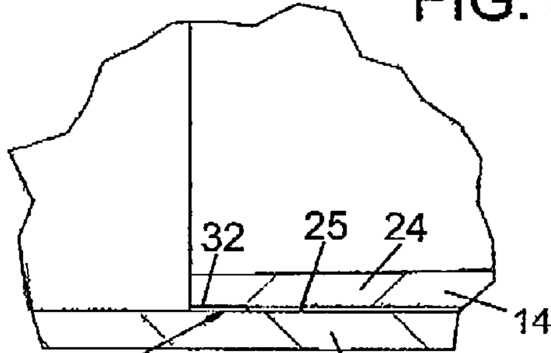
DETAIL C
