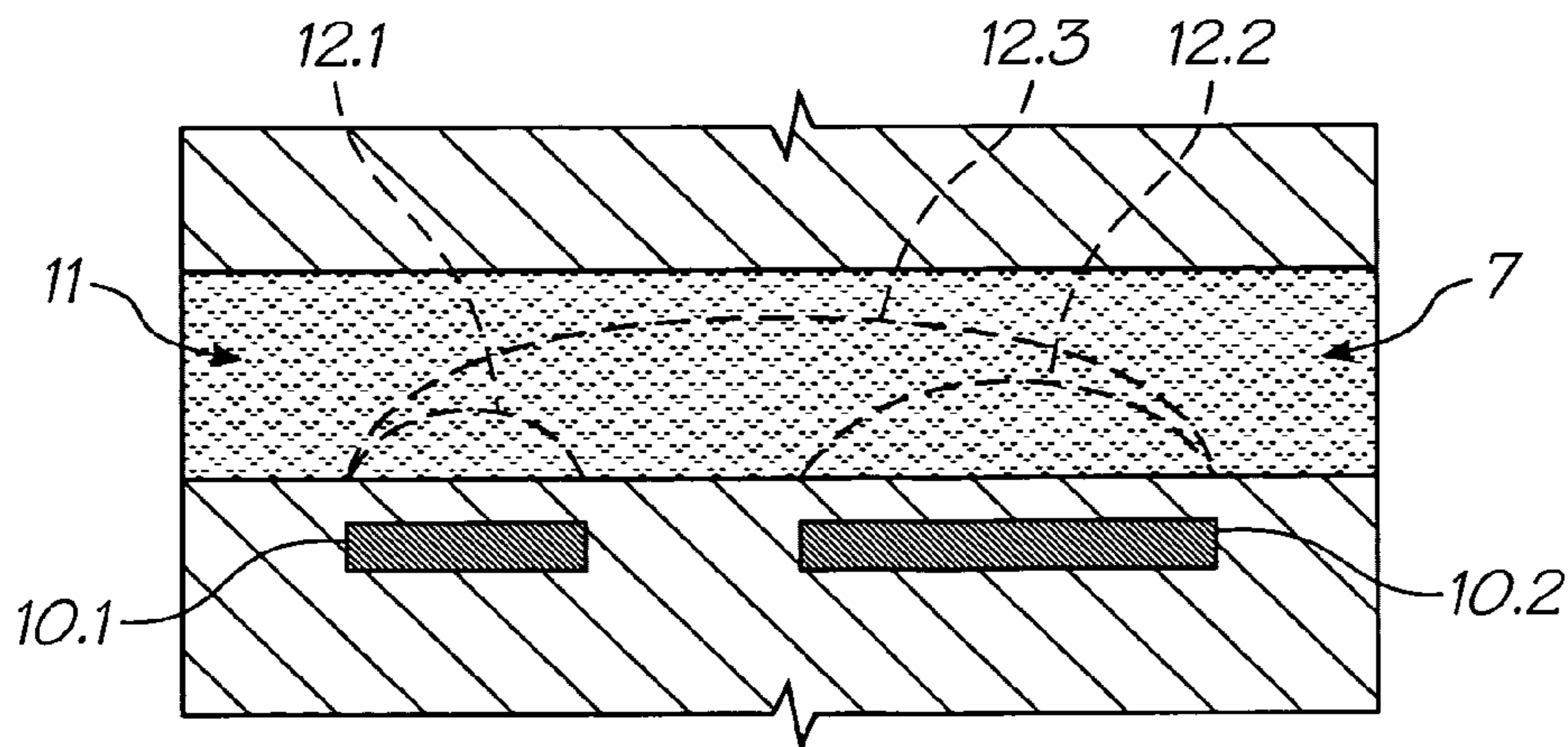
FIG. 52 (PRIOR ART)
