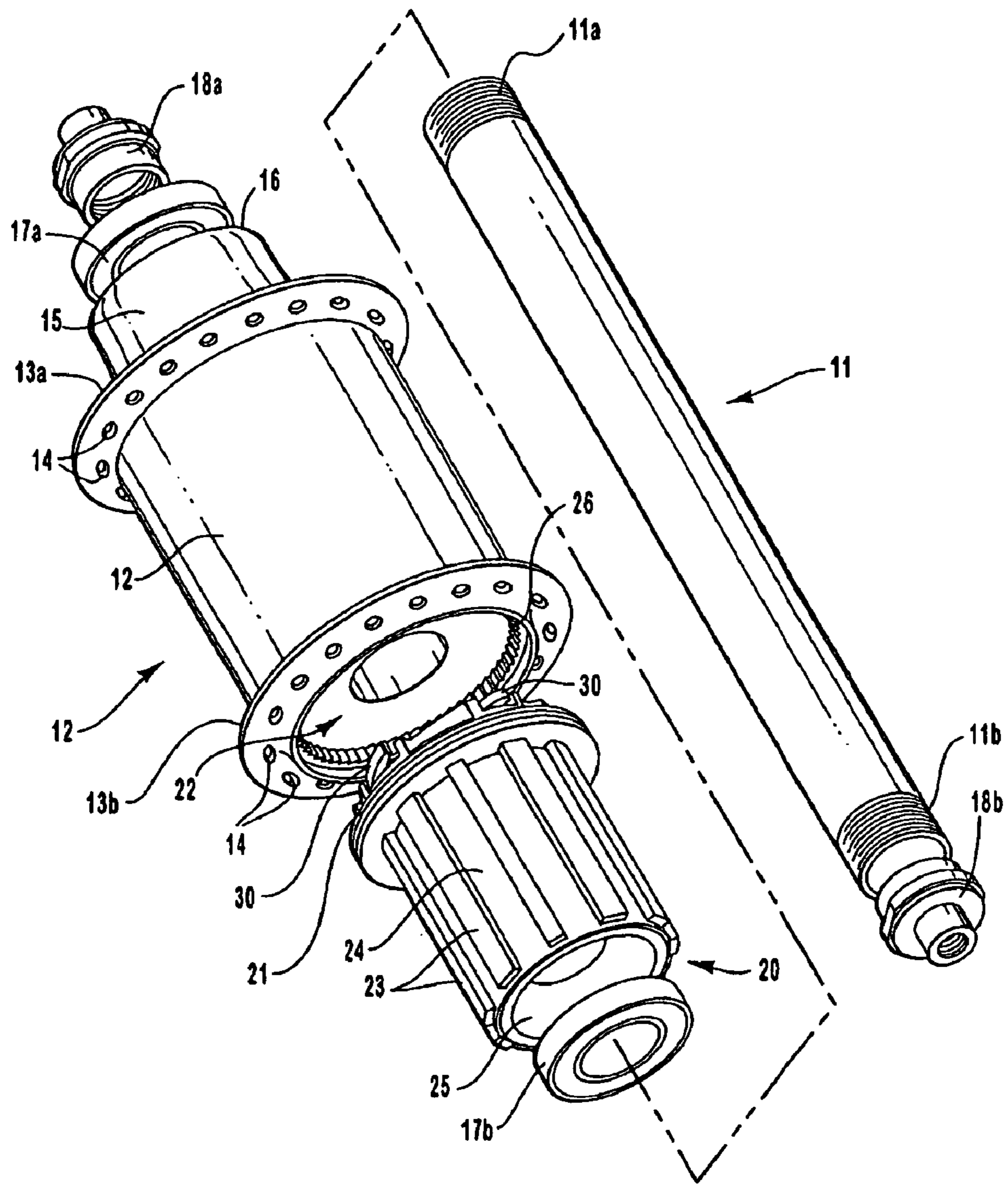
FIG. 1 (PRIOR ART)
