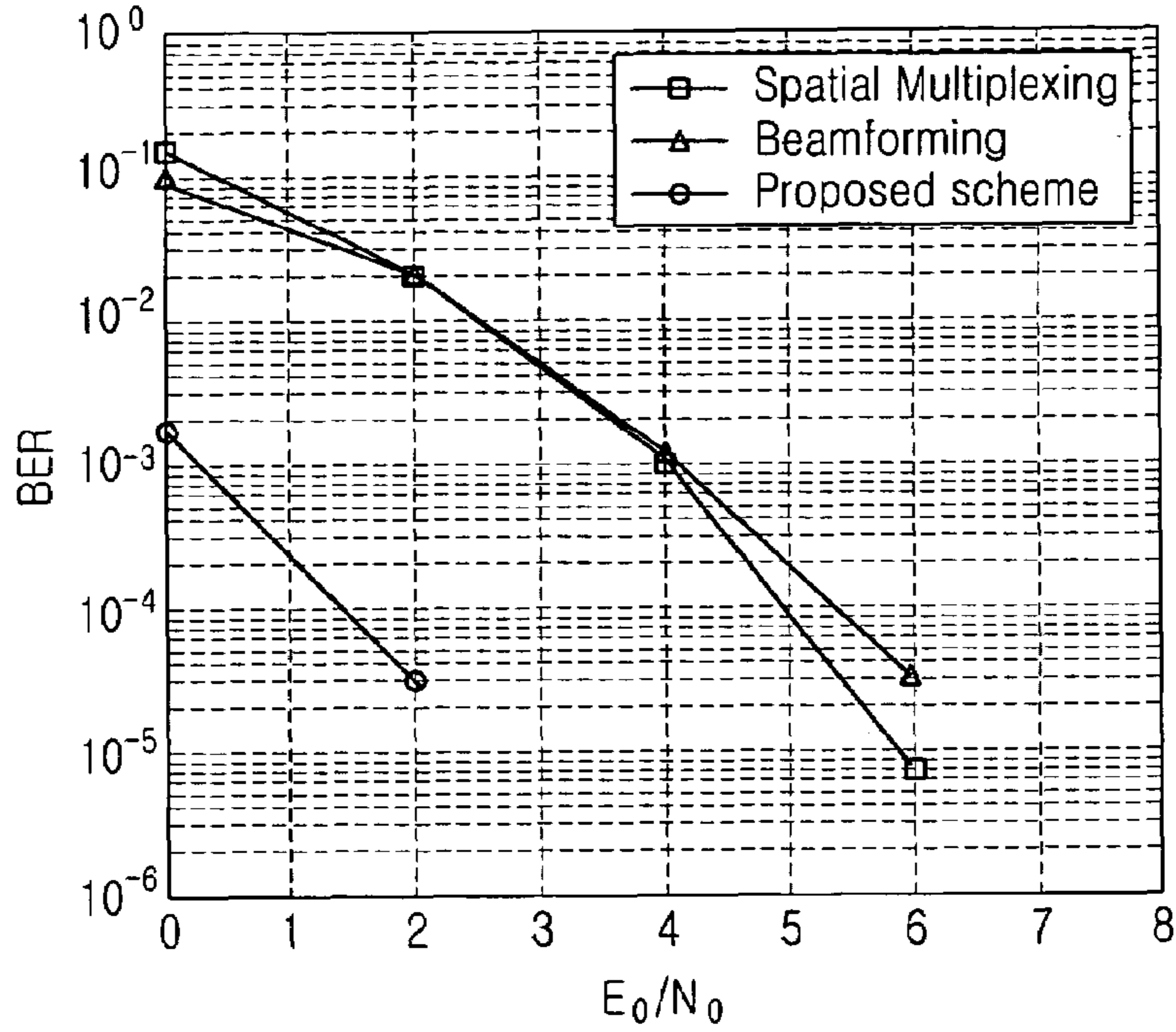
BER when the channels correlation coefficient is 0.5 (ML decoding)
