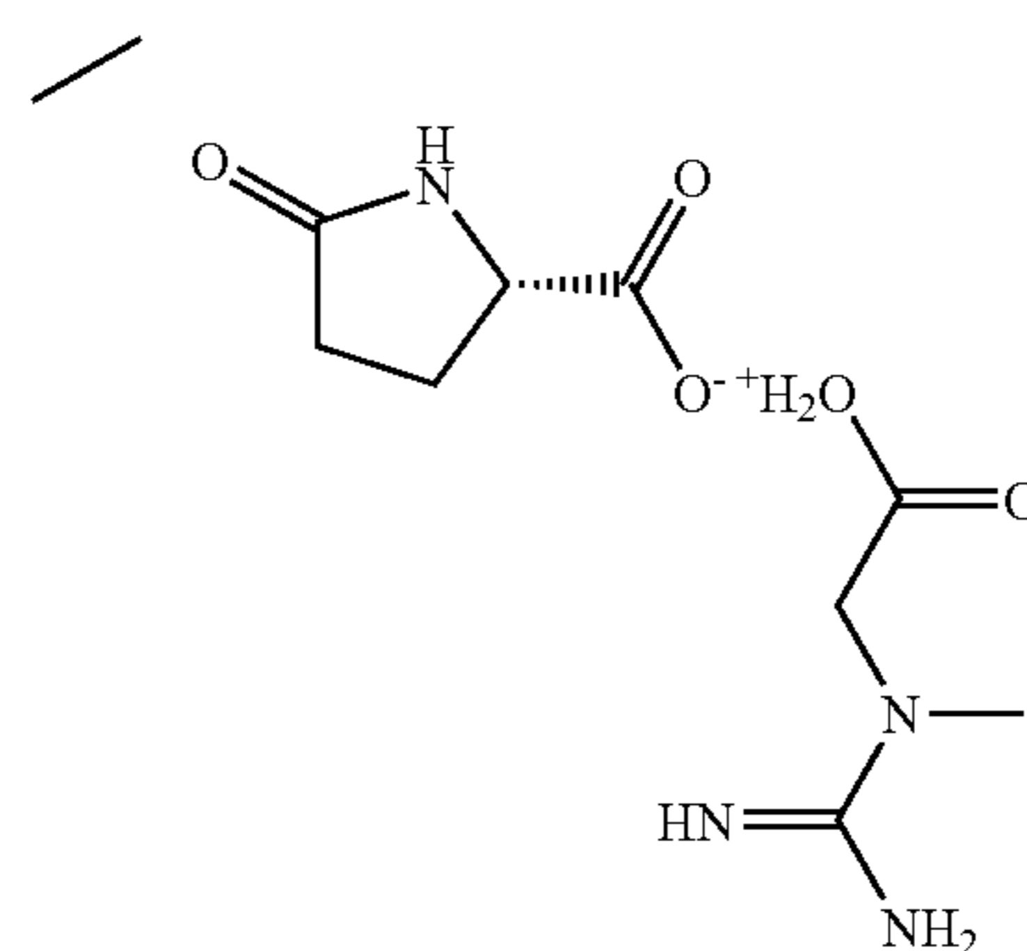
Fig.1. Schematic Representation of Creatine Pyroglutamate
