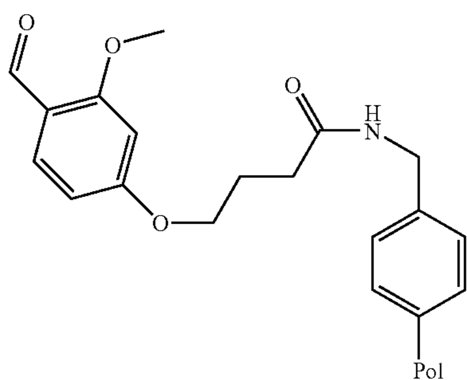
4-(4-formyl-3-methoxyphenoxy)butynyl polyethylene glycol grafted aminomethylpolystyrene-1% DVB
