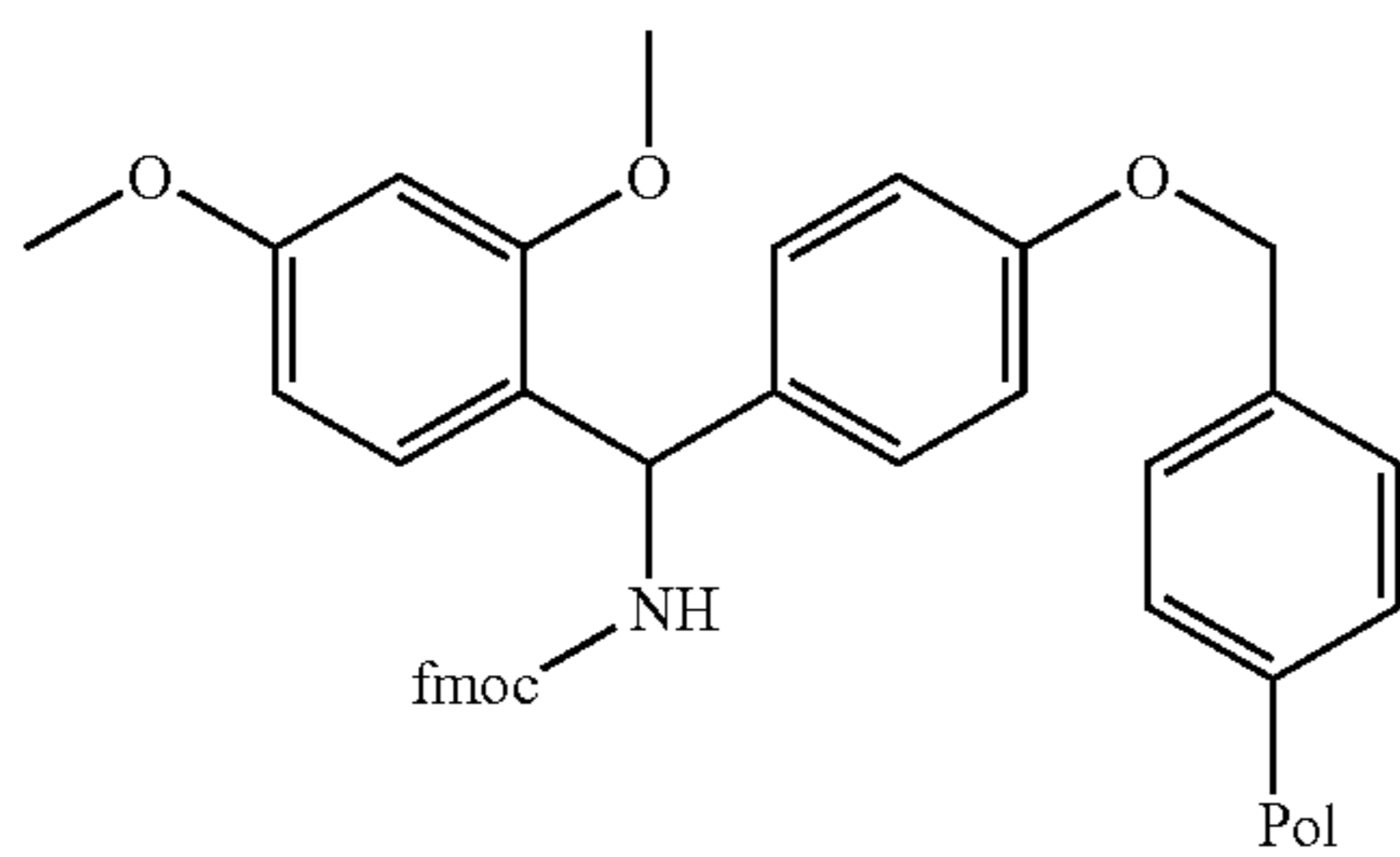
4-(2',4'-dimethoxyphenyl-fmoc-aminomethyl)phenoxy (copolystyrene-1% DVB)
