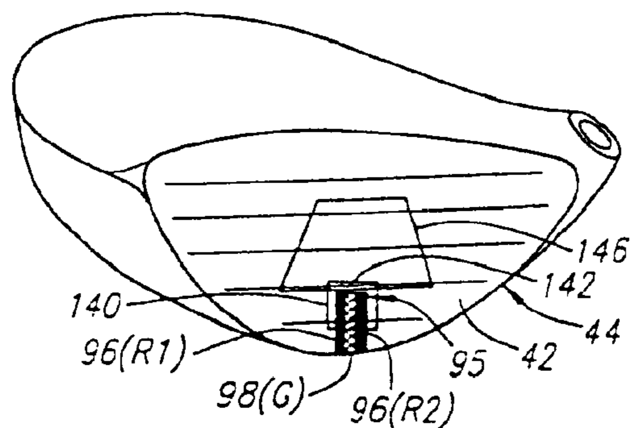
STRAIGHT-THROUGH FIG. 3B
