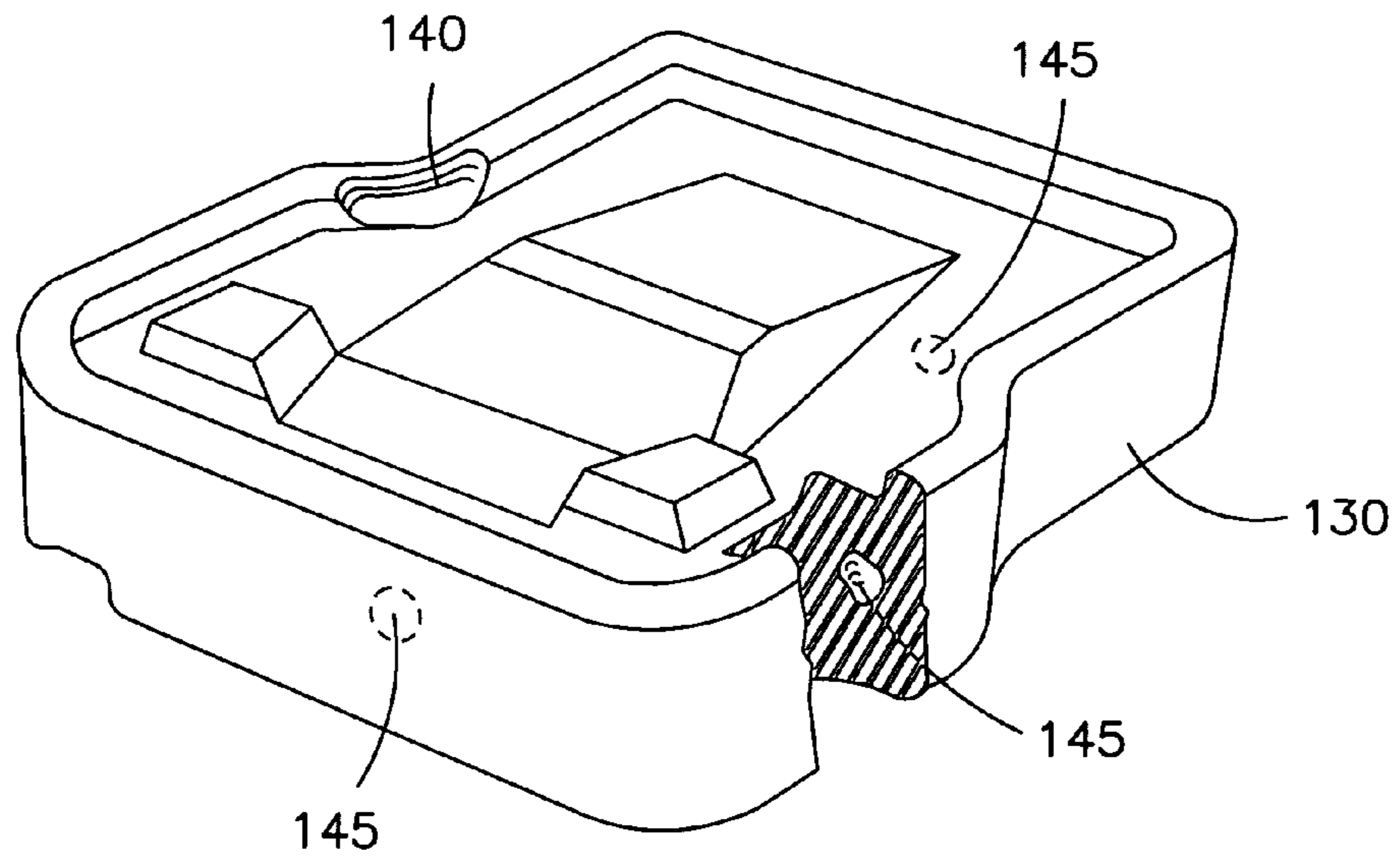
FIG. 7 PRIOR ART
