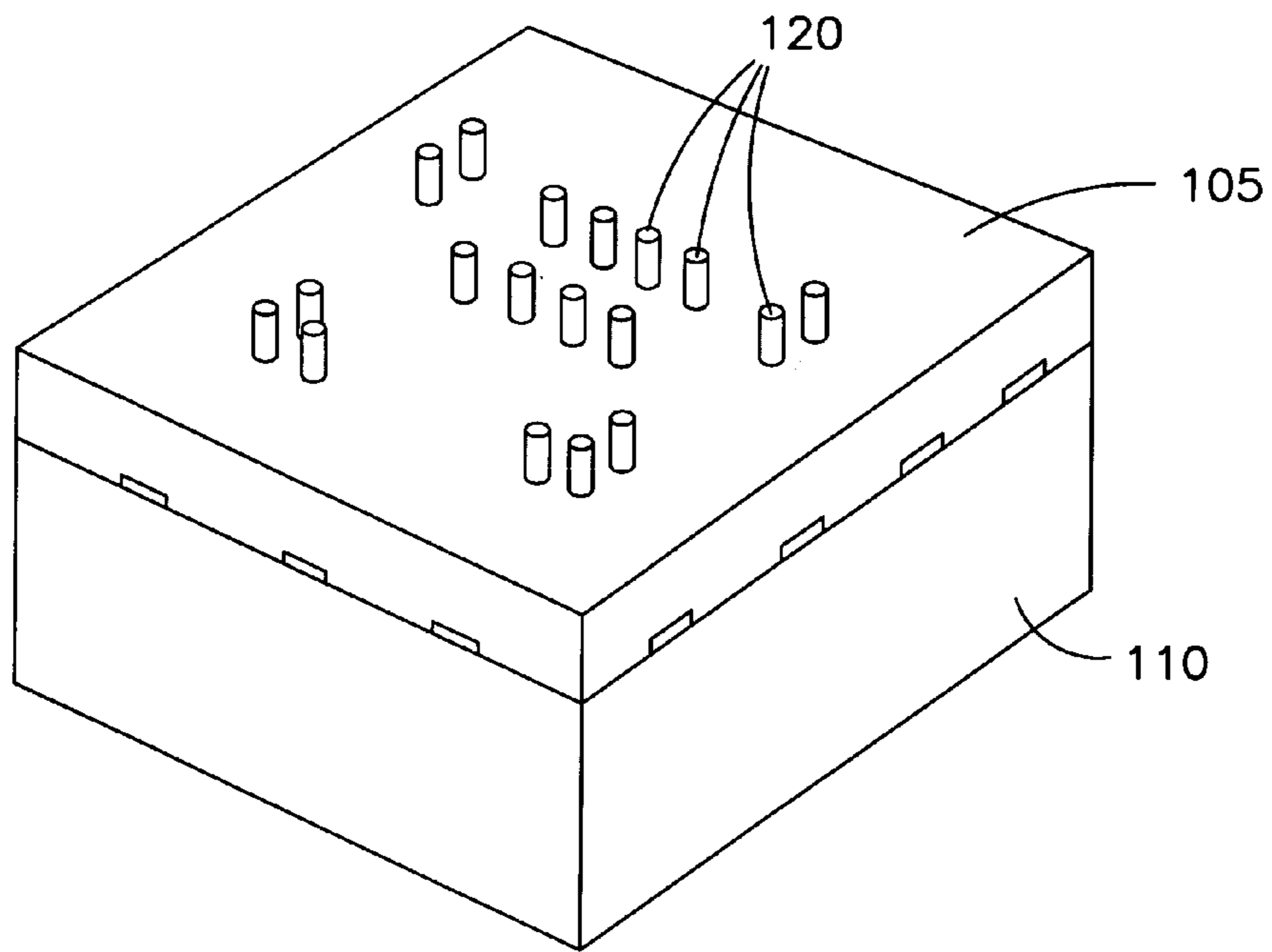
FIG. 6 PRIOR ART
