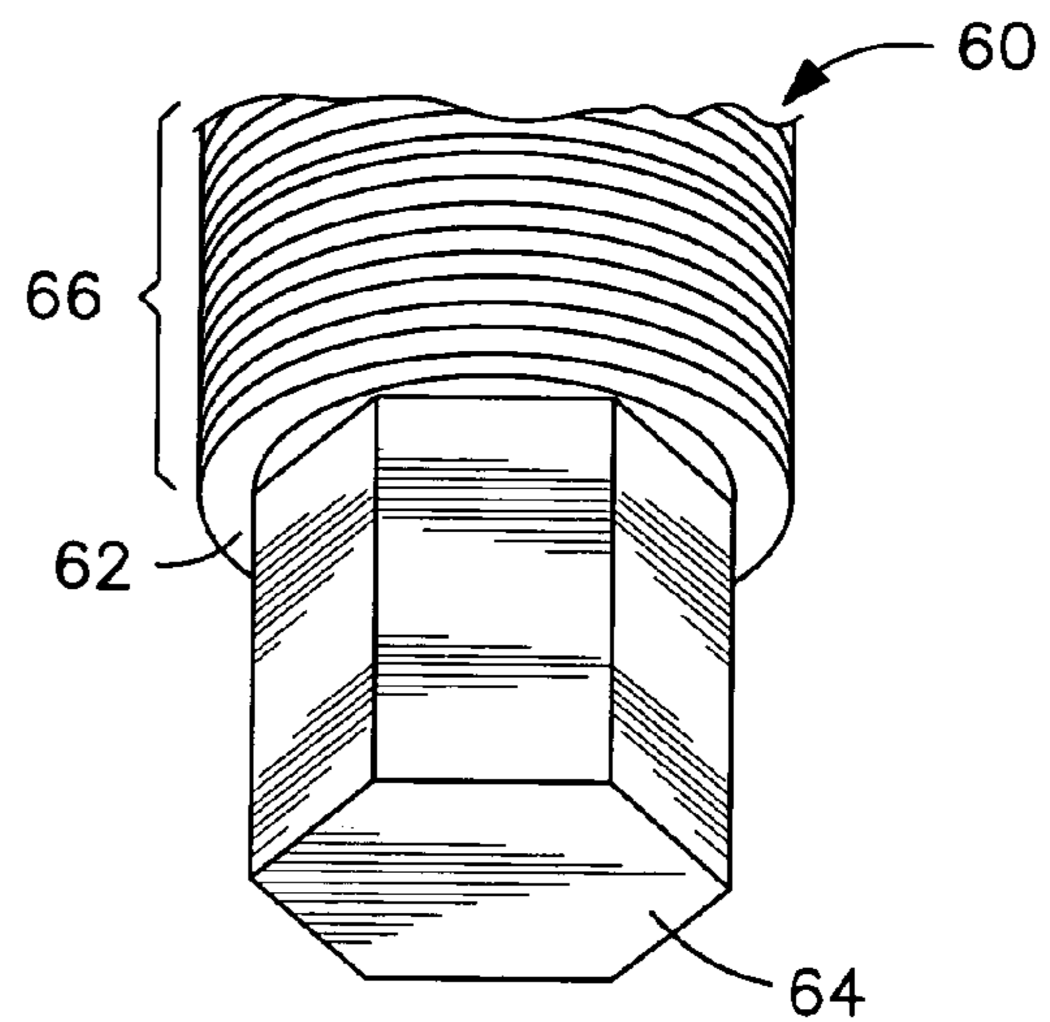
FIG. 4 PRIOR ART
