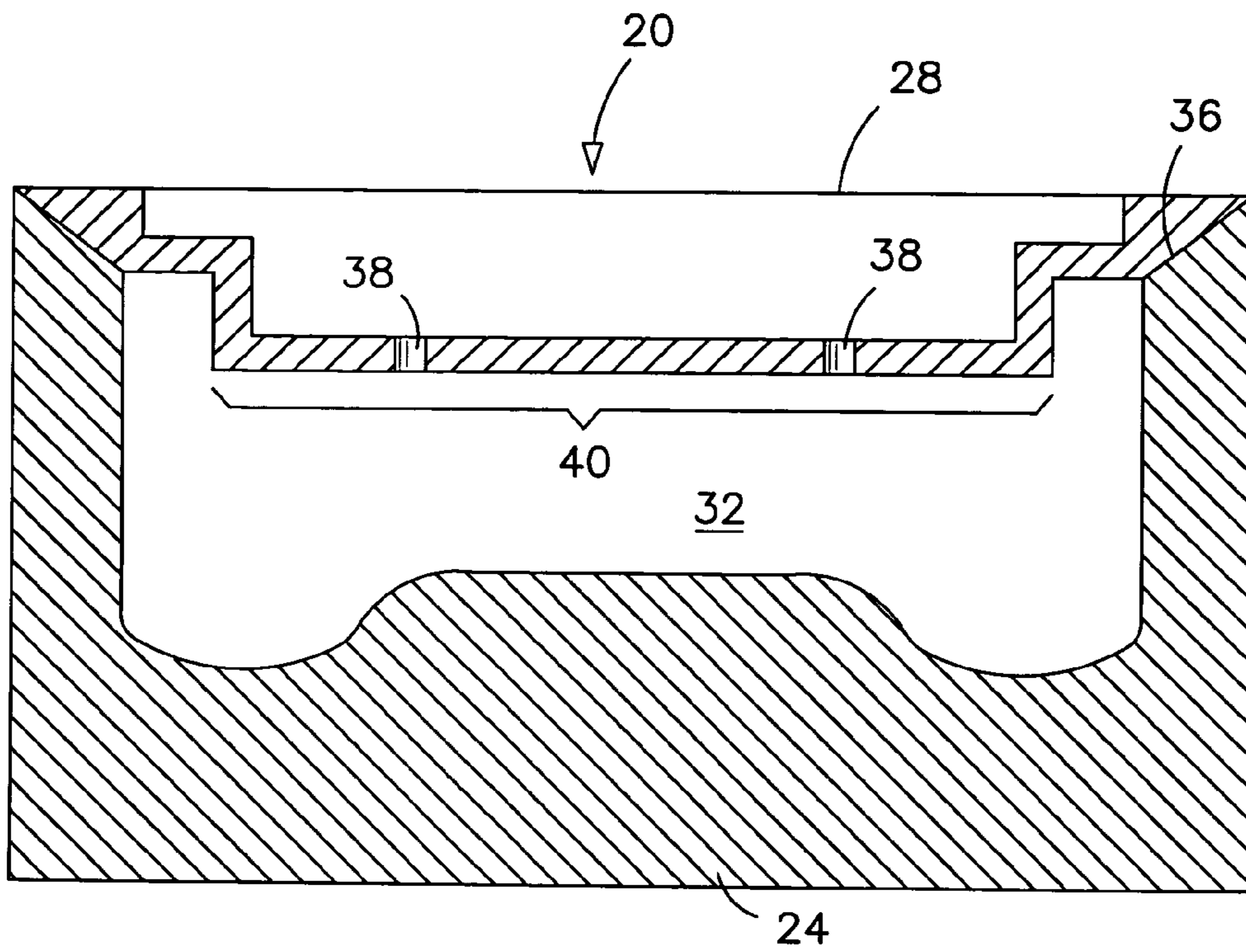
FIG. 1 PRIOR ART
