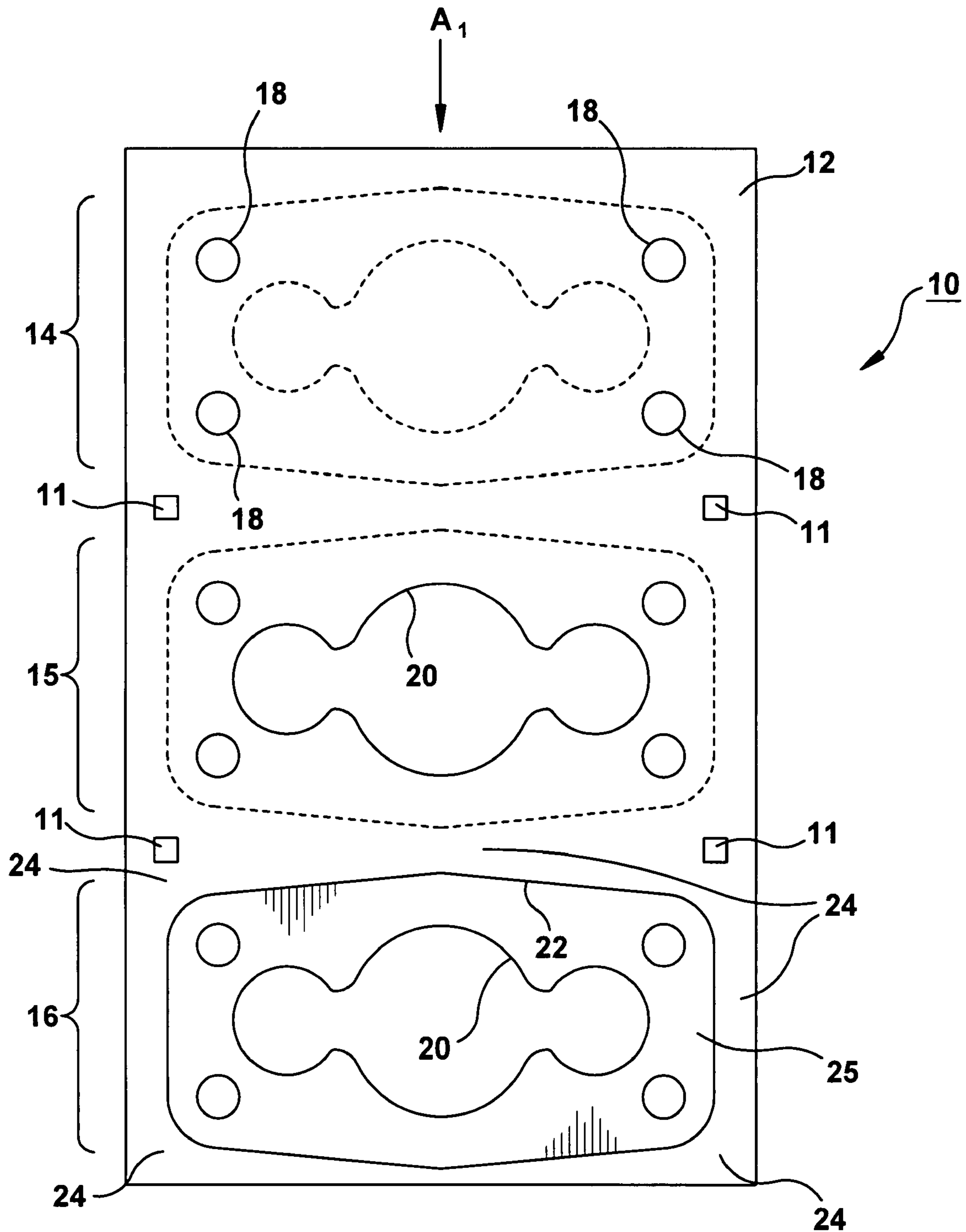
Fig. 1 (PRIOR ART)
