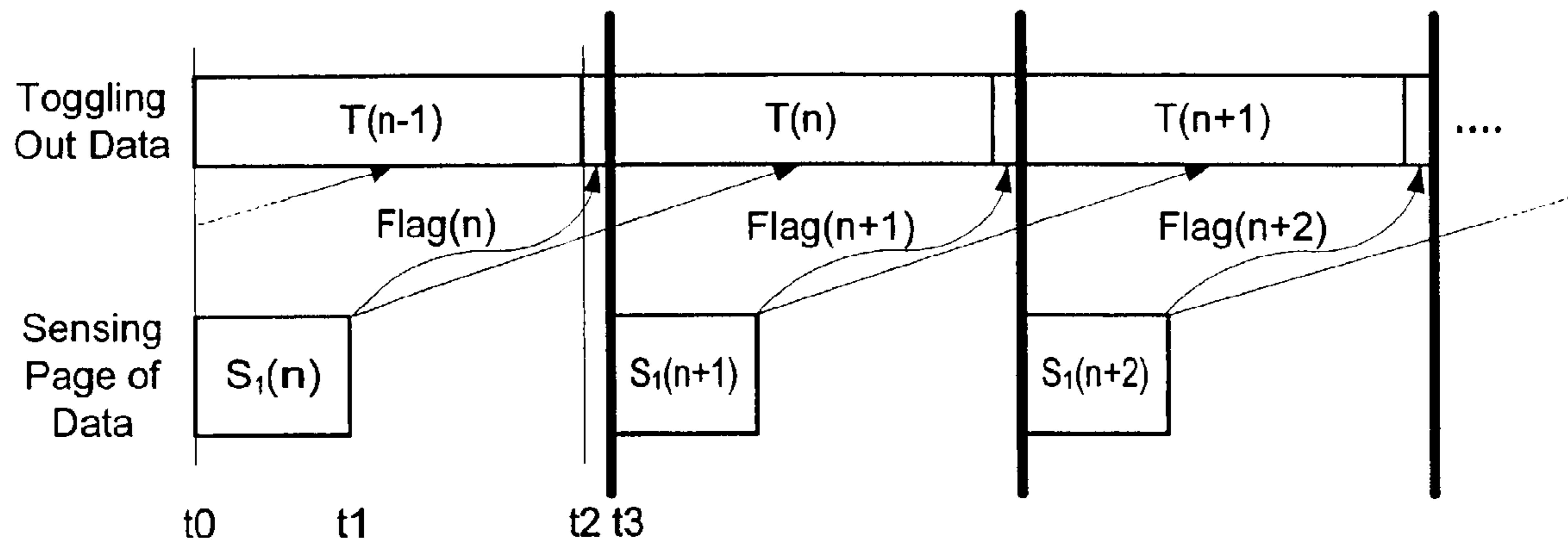
Read Caching with LM Coding
