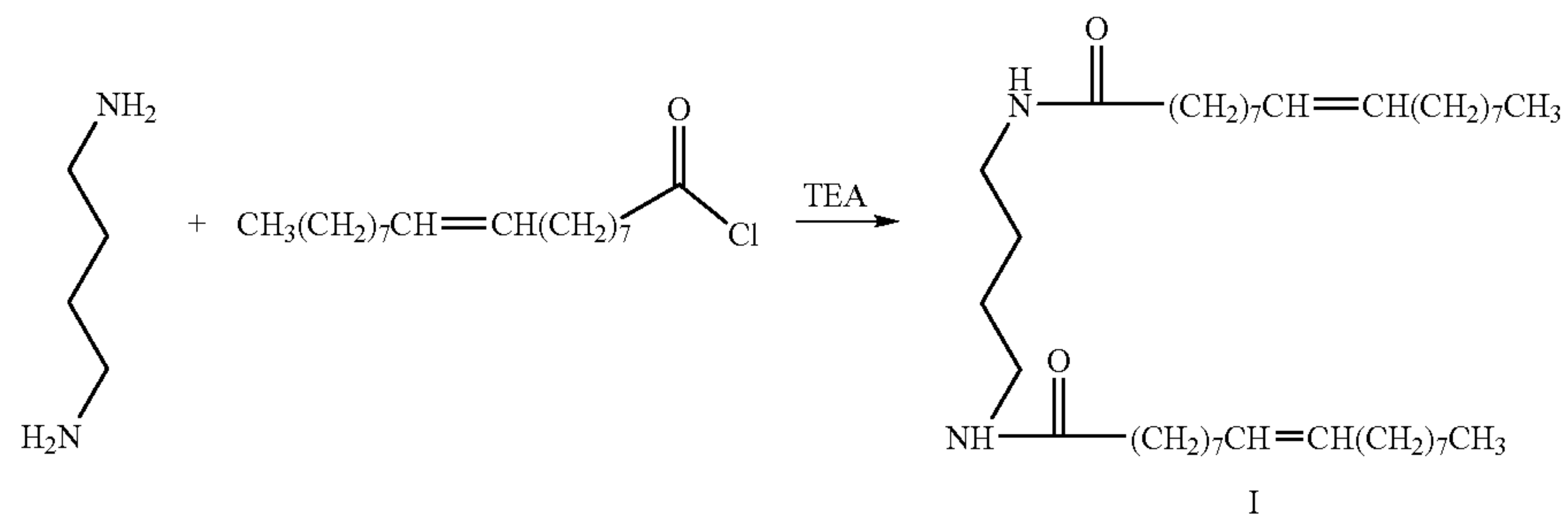
Synthesis of dihydroxy-dioleyl-dispermincarboxamido spermine and analogs (Scheme 1)
