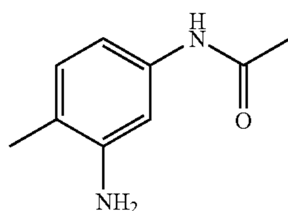
N-(3-Amino-4-methyl-phenyl)-acetamide
