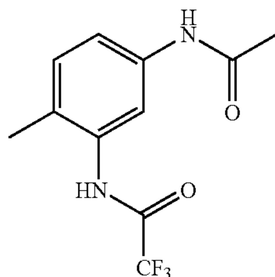
N-(5-Acetylamino-2-methyl-phenyl)-2,2,2-trifluoro-acetamide
