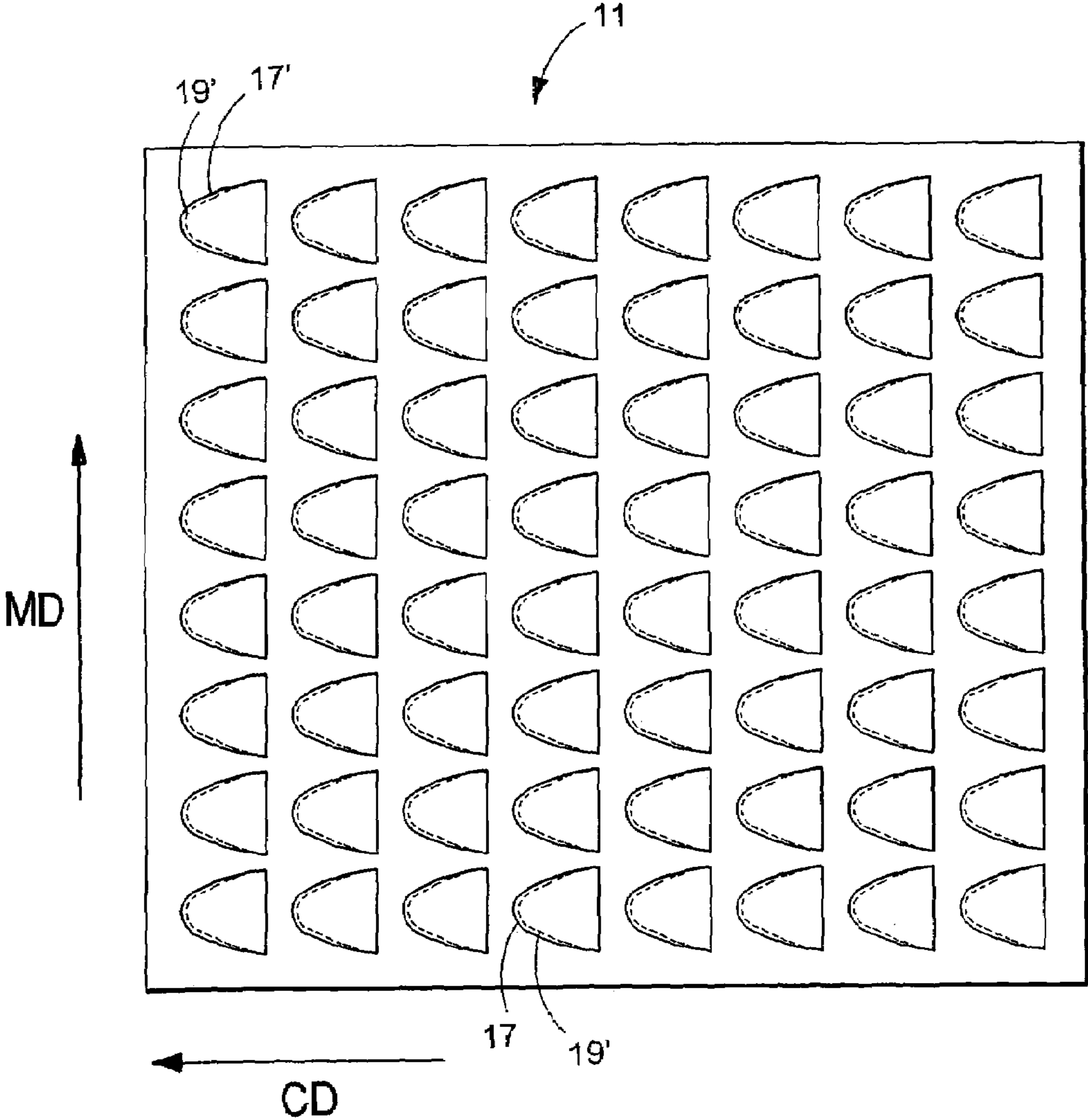
FIG. 1D
