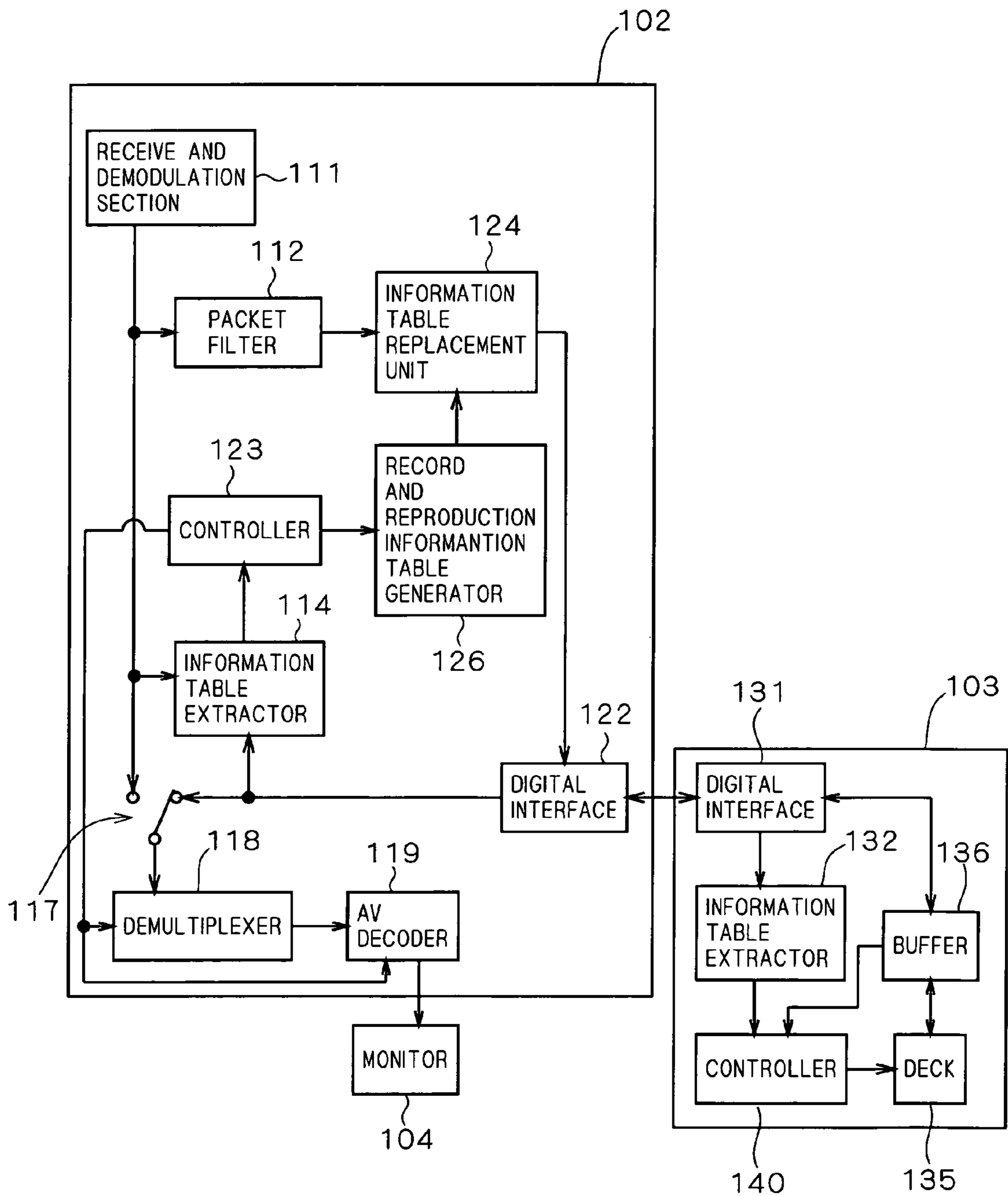
FIG. 22 (PRIOR ART)
