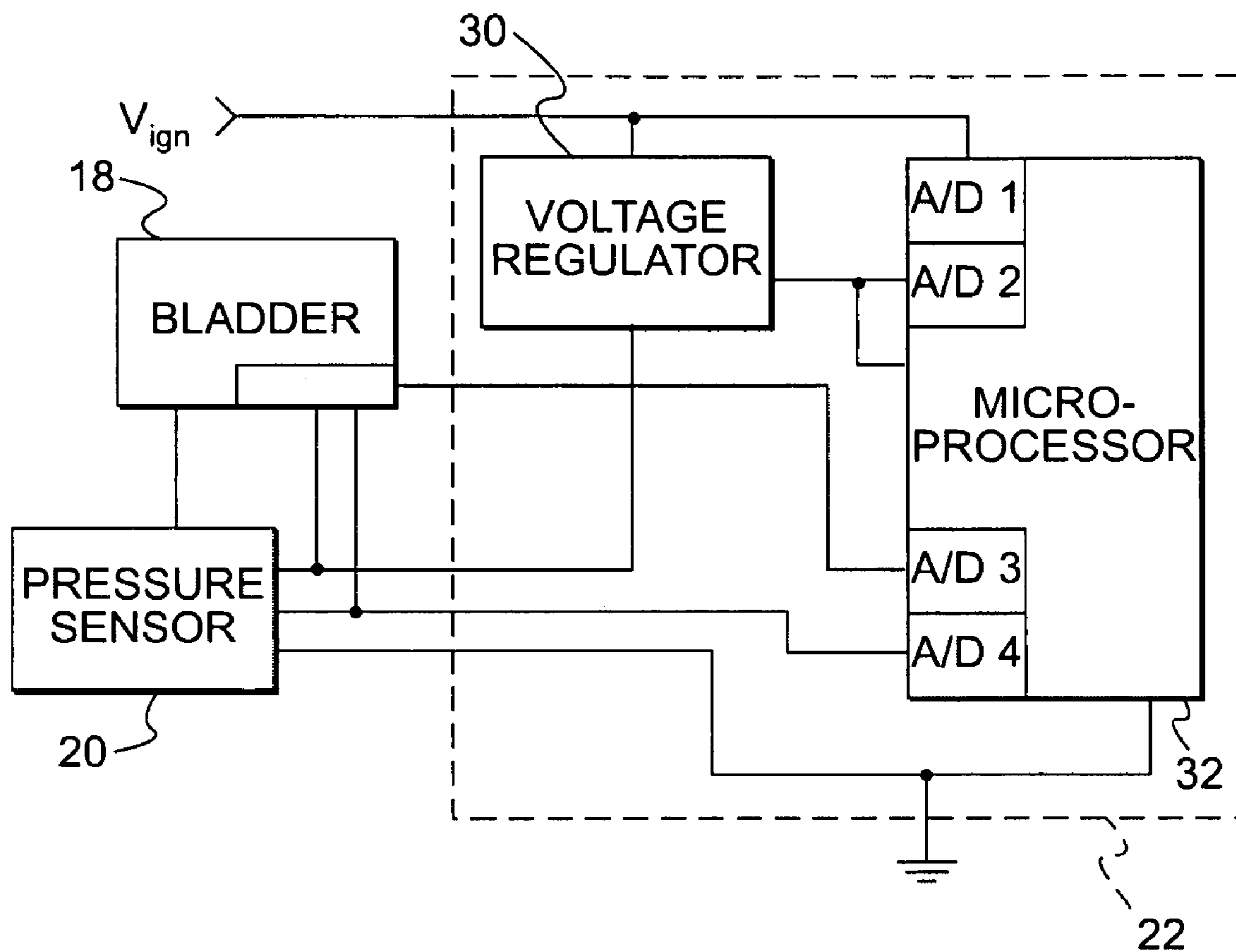
FIG. 3 PRIOR ART
