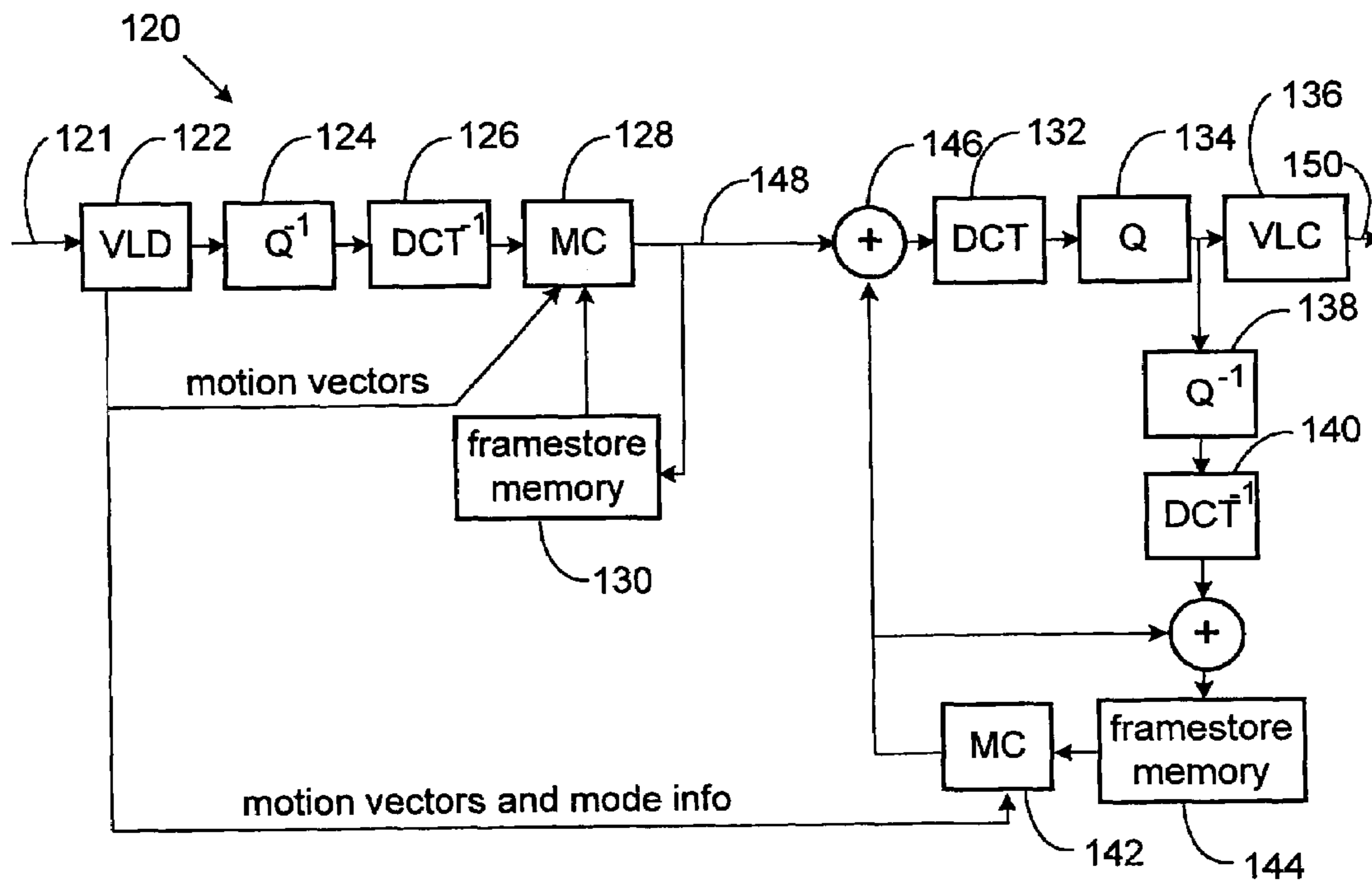
Figure 4B (PRIOR ART)
