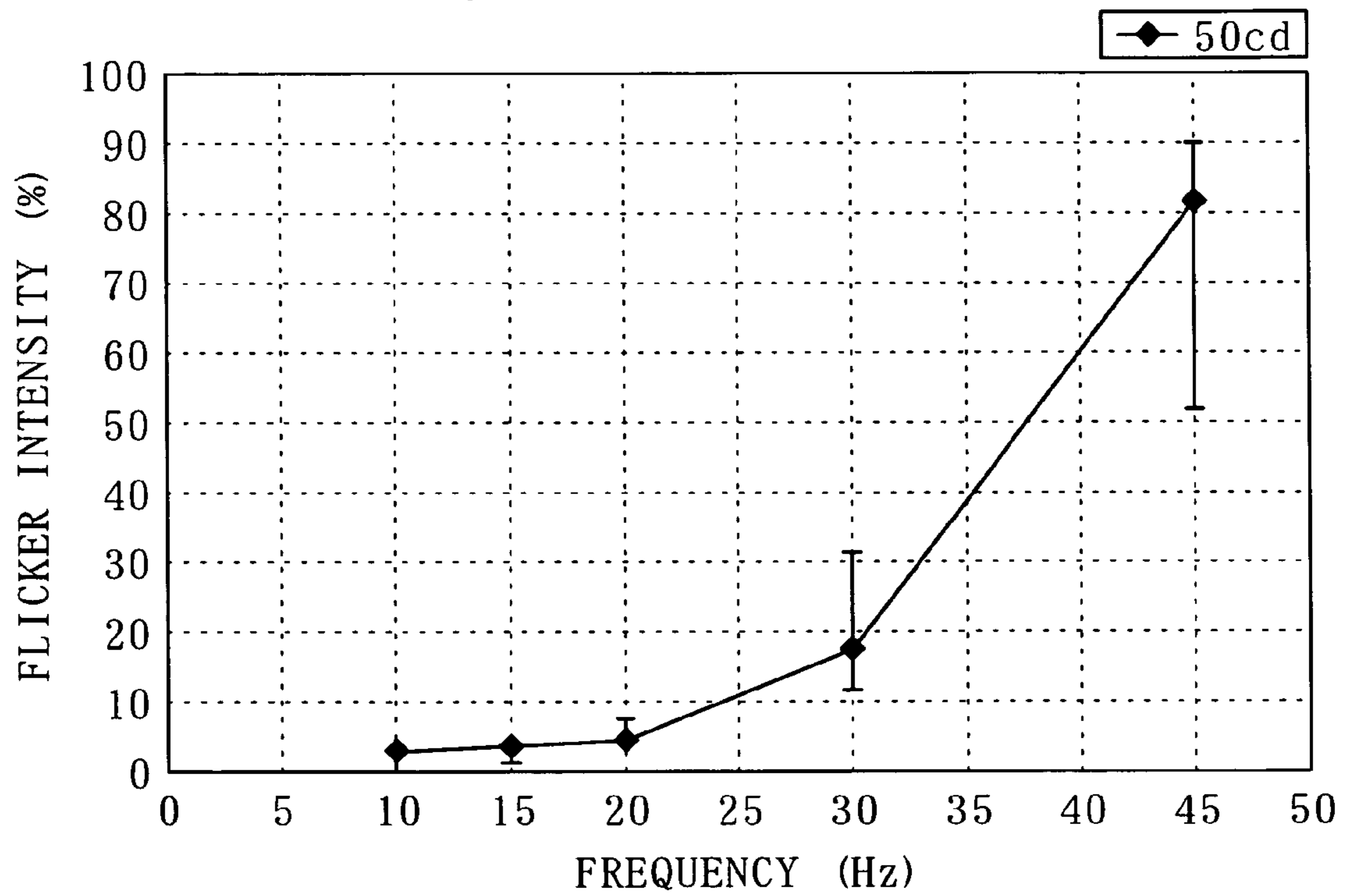
DEPENDENCE OF DETECTION THRESHOLD ON FREQUENCY
