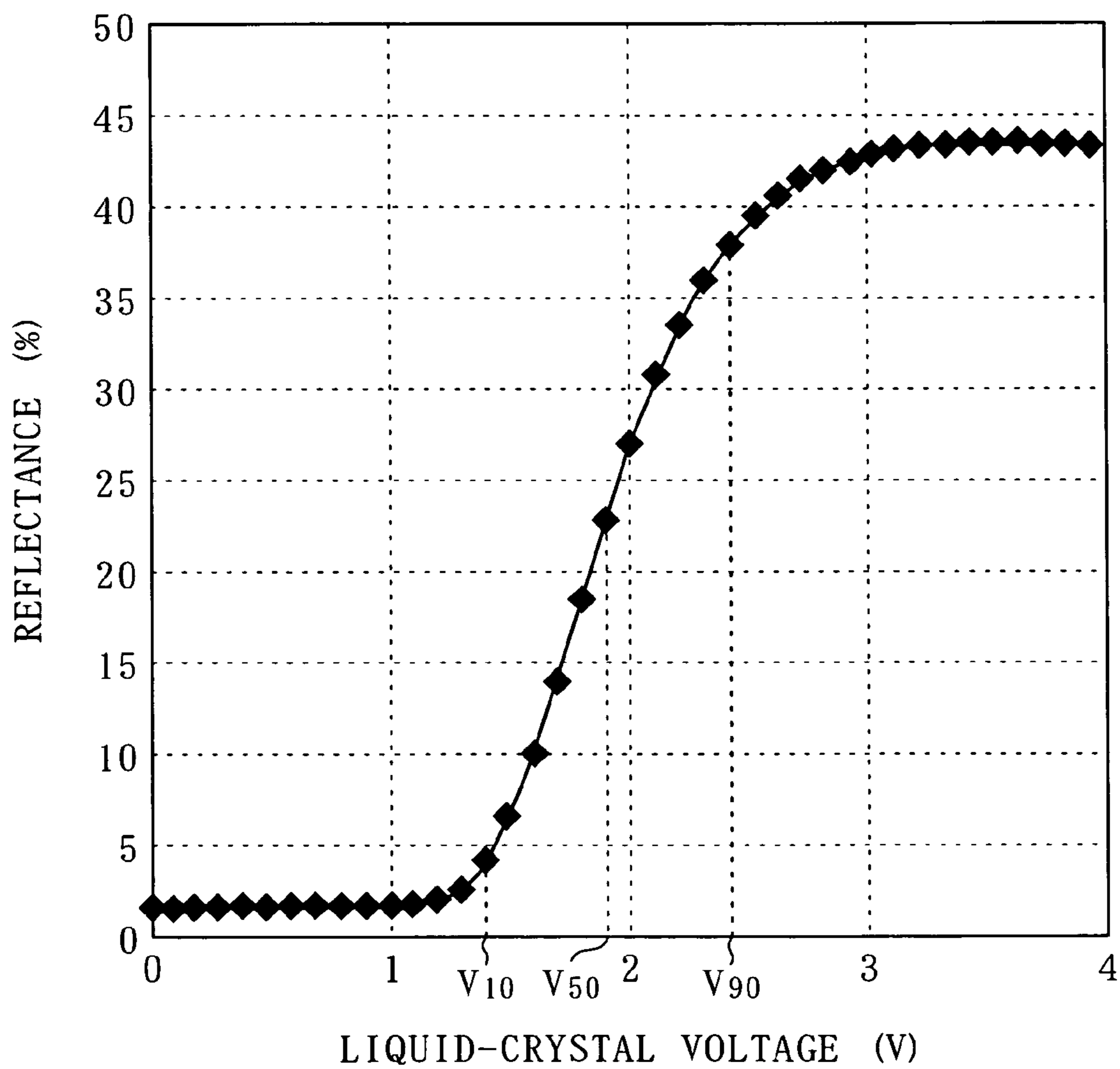
REFLECTANCE (%) VERSUS LIQUID-CRYSTAL VOLTAGE (V)
