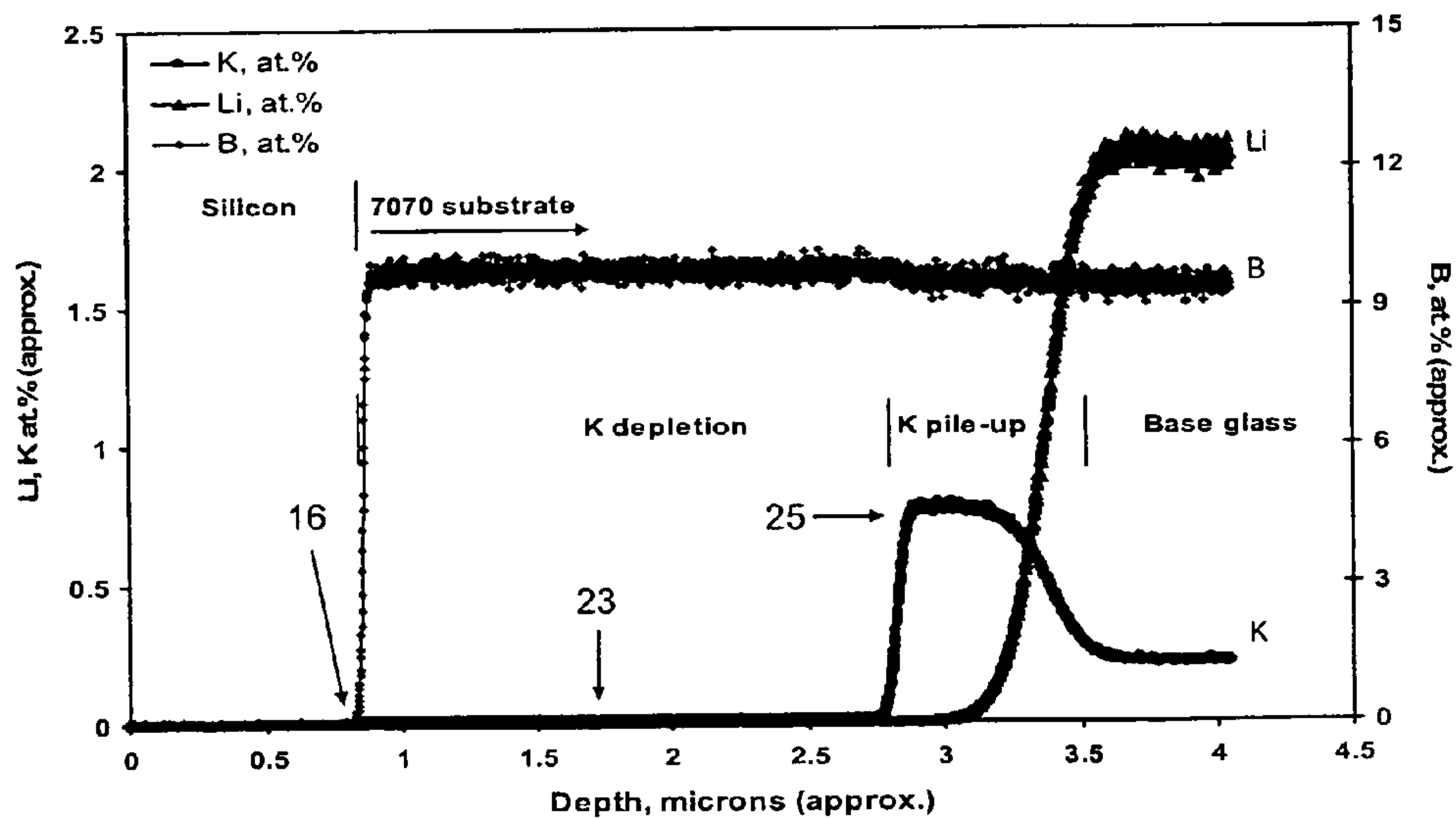
ToF-SIMS DEPTH PROFILE OF Si/7070 (RE-FIRED)
