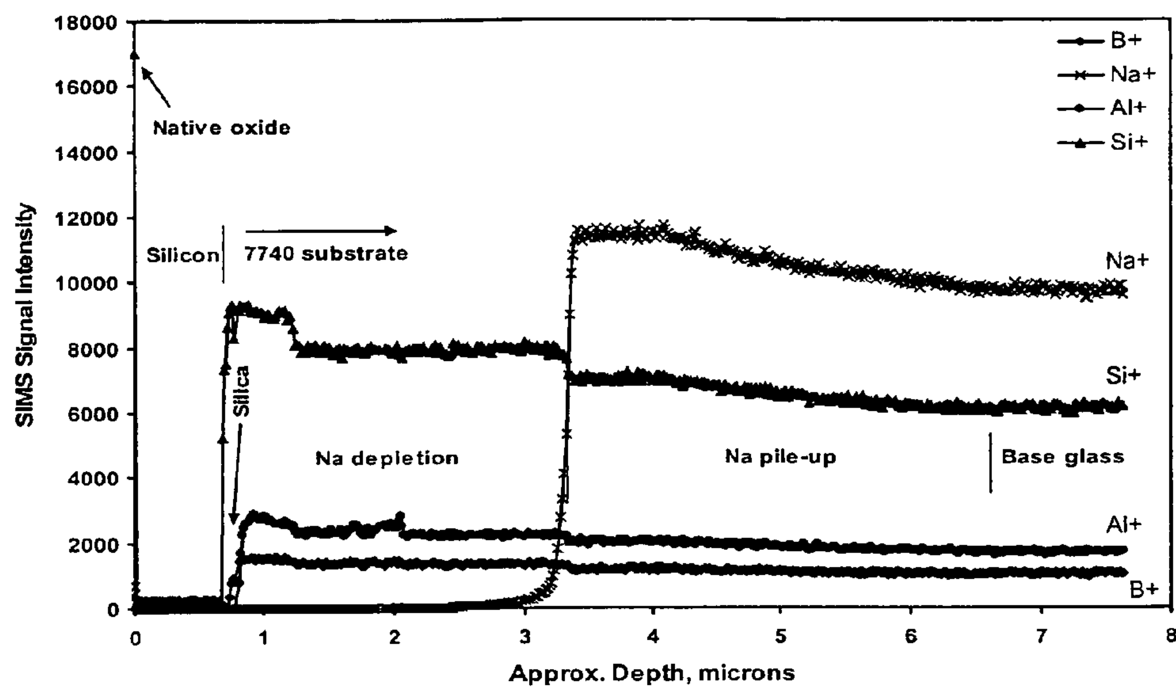
ToF-SIMS DEPTH PROFILE OF Si/7740 (RE-FIRED)
