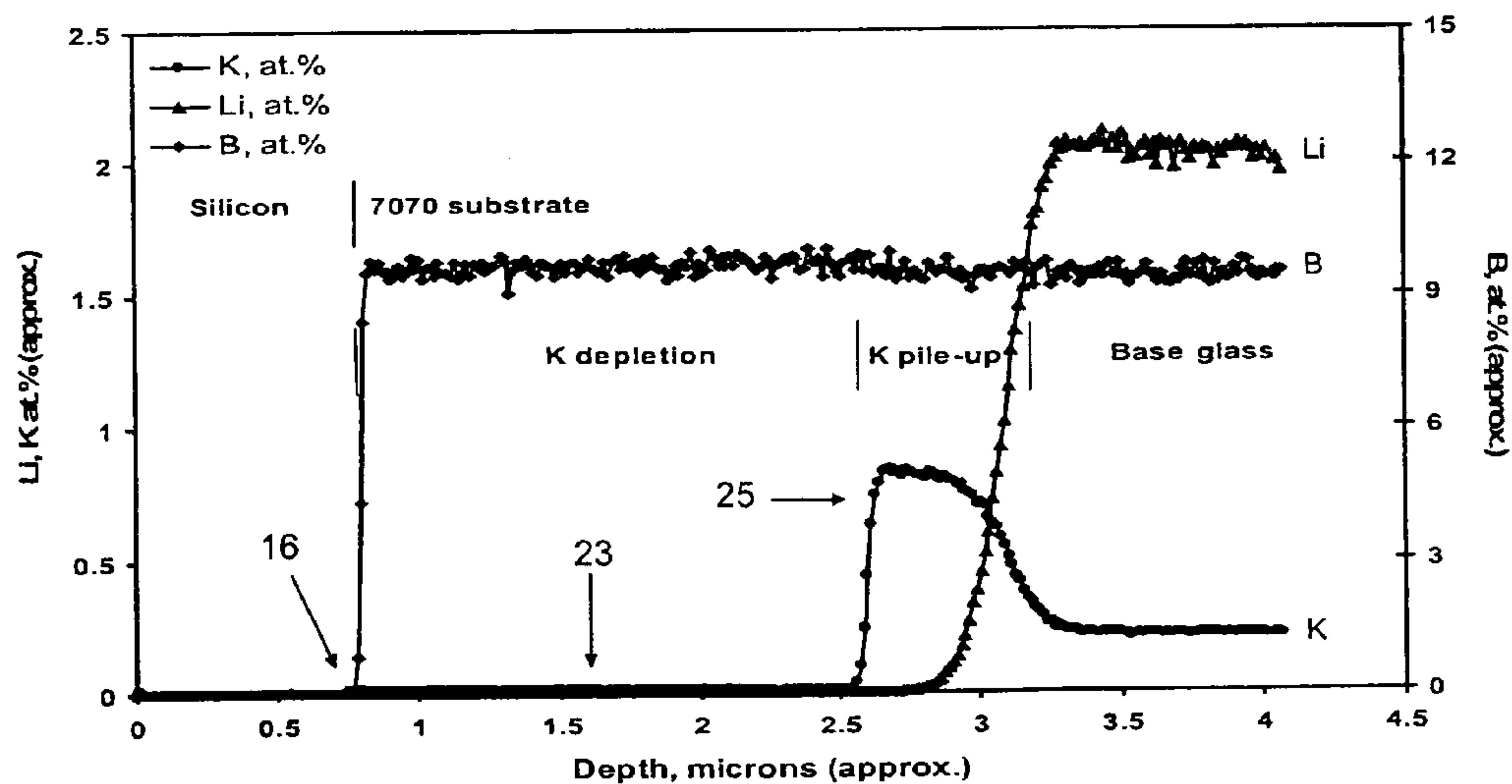
ToF-SIMS DEPTH PROFILE OF Si/7070 (AS BONDED)
