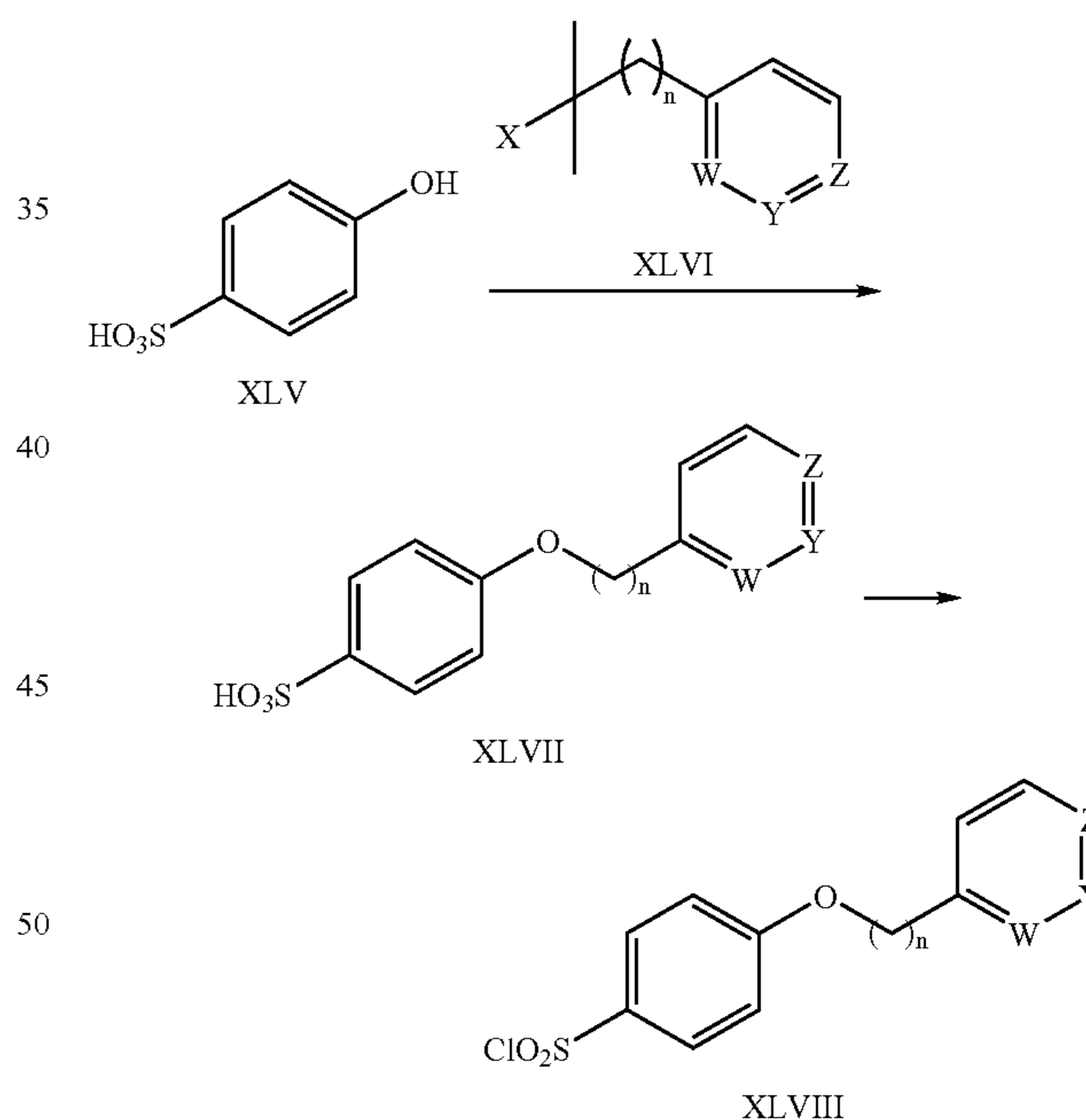
Scheme 23a-Preparation of sulfonyl chloride XLVIII:
