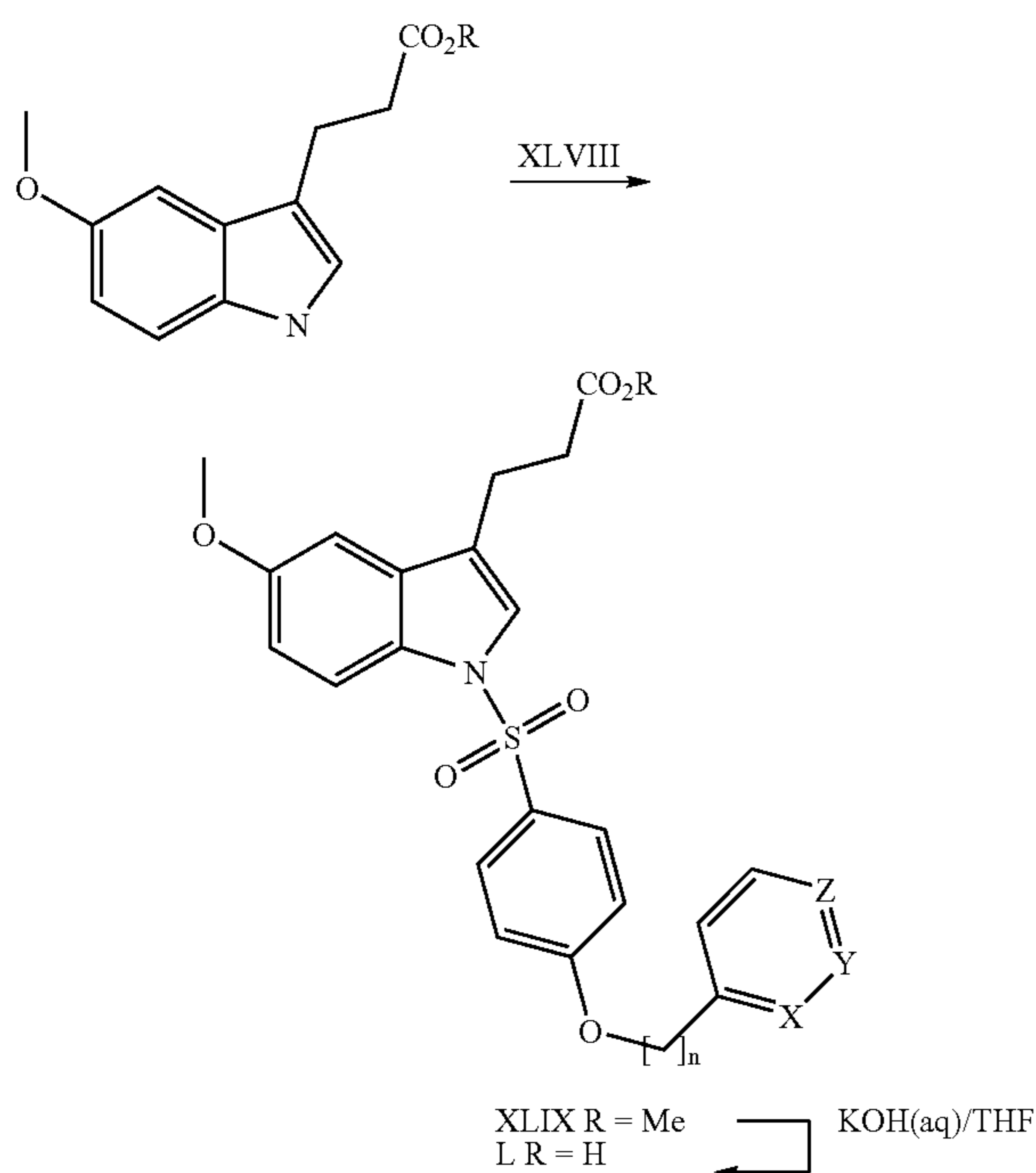
Scheme 23b-Preparation of Compound of Formula L
