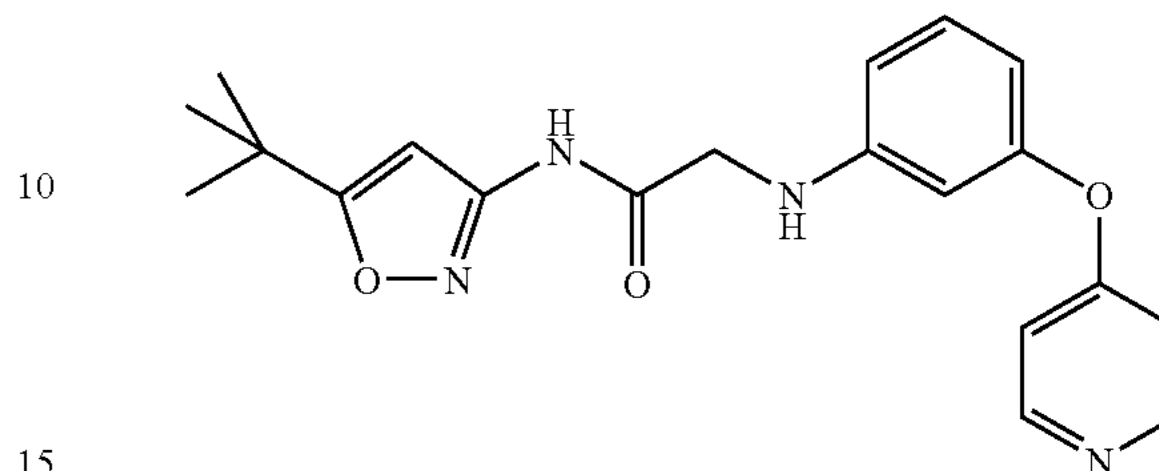
(4): N-(4-Chloro-3-trifluoromethyl-phenyl)-2-[3-(pyridin-3-yloxy)-phenylamino]-acetamide
