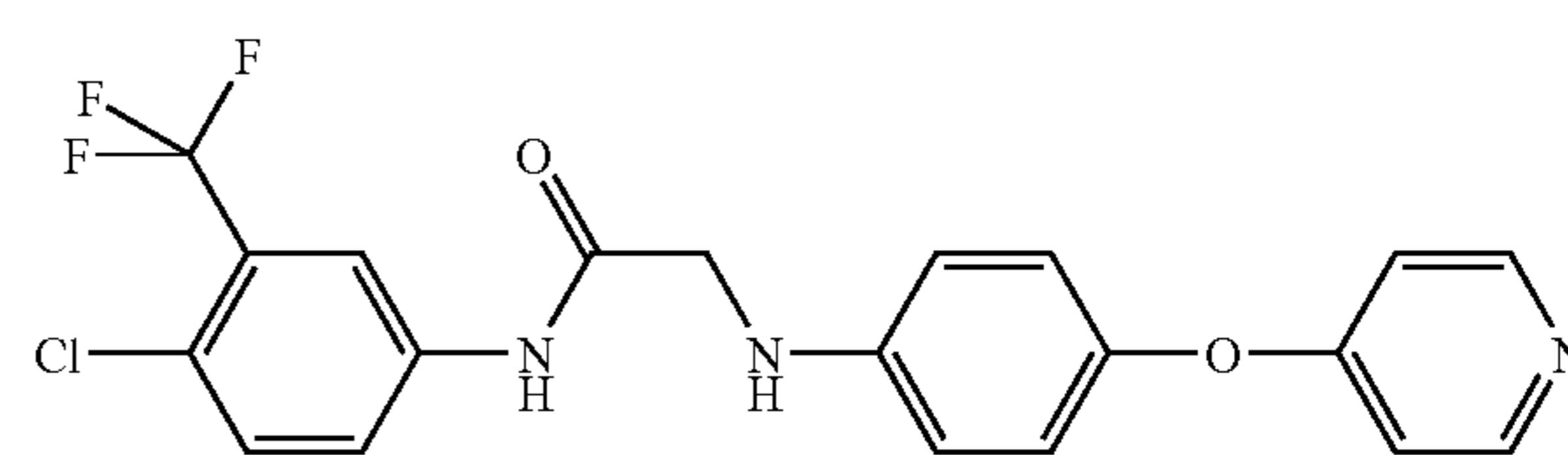
(1): N-(4-Chloro-3-trifluoromethyl-phenyl)-2-[4-(pyridin-4-yloxy)-phenylamino]-acetamide
