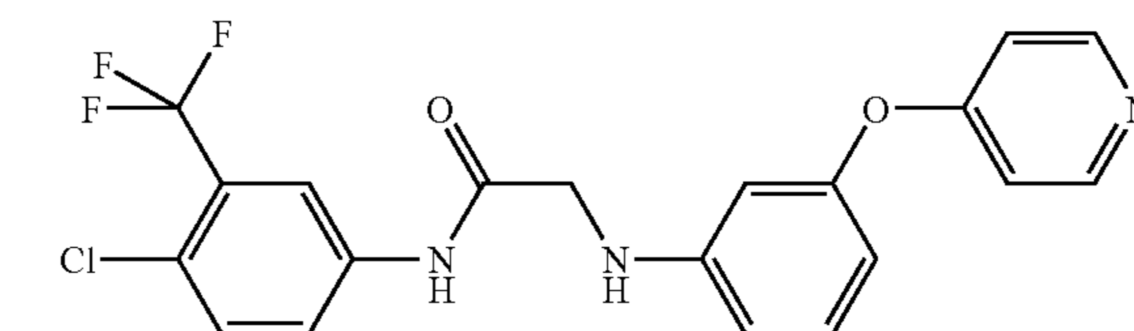
(2): N-(4-Chloro-3-trifluoromethyl-phenyl)-2-[3-(pyridin-4-yloxy)-phenylamino]-acetamide
