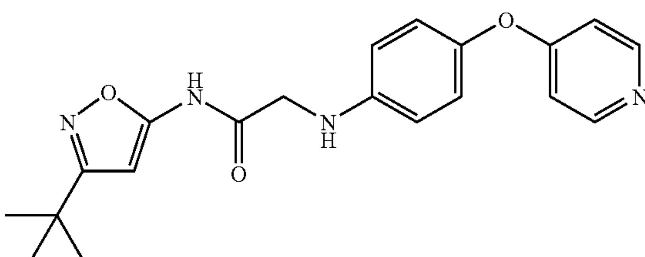
(8): N-(5-tert.-Butyl-isoxazol-3-yl)-2-[4-(pyridin-4-yloxy)-phenylamino]-acetamide
