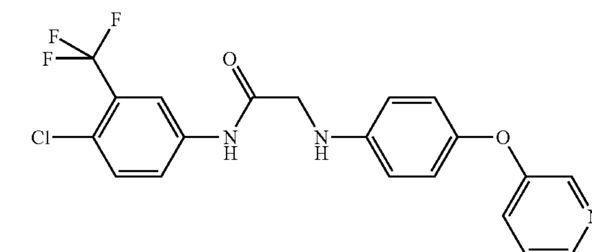
(3): N-(4-Chloro-3-trifluoromethyl-phenyl)-2-[4-(pyridin-3-yloxy)-phenylamino]-acetamide
