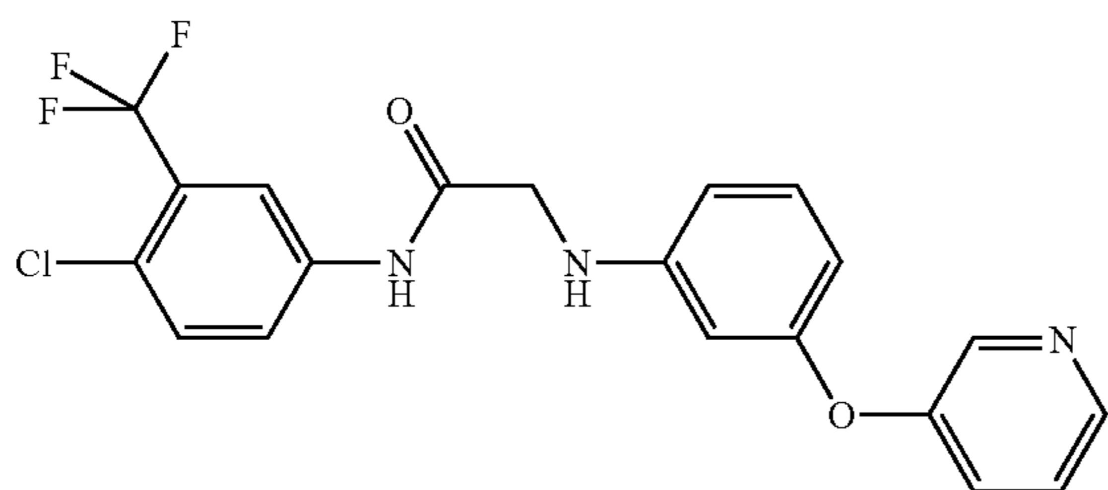
(4): N-(4-Chloro-3-trifluoromethyl-phenyl)-2-[3-(pyridin-3-yloxy)-phenylamino]-acetamide
