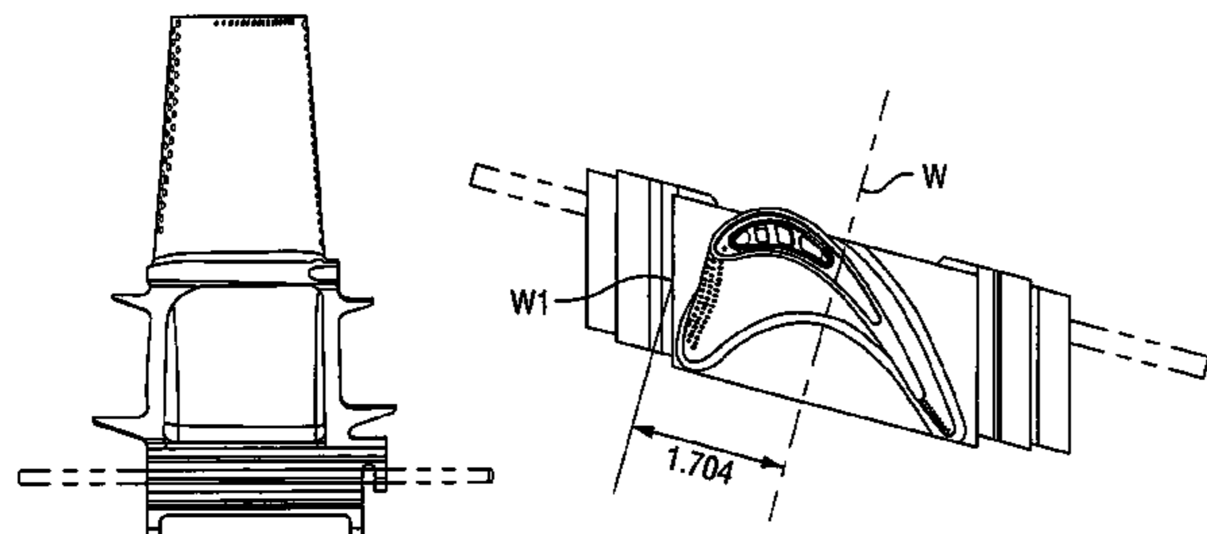
The plane containing Datum W is located 1.704 inches from Pt. W1 as measured along Datum S (centerline of the dovetail axis). Pt. W1 is in the fwd face of the dovetail.
