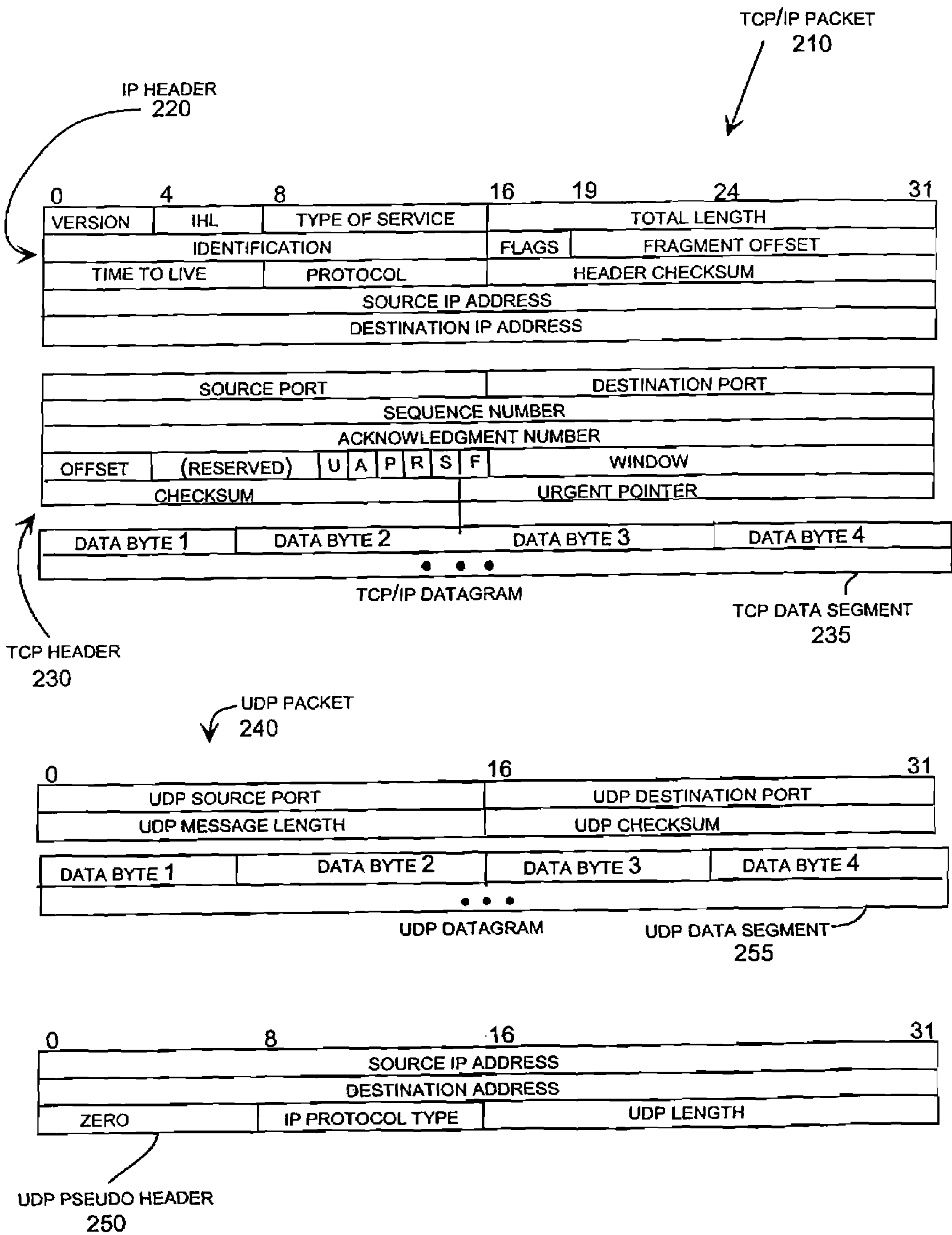
PACKET HEADERS FIG. 2
