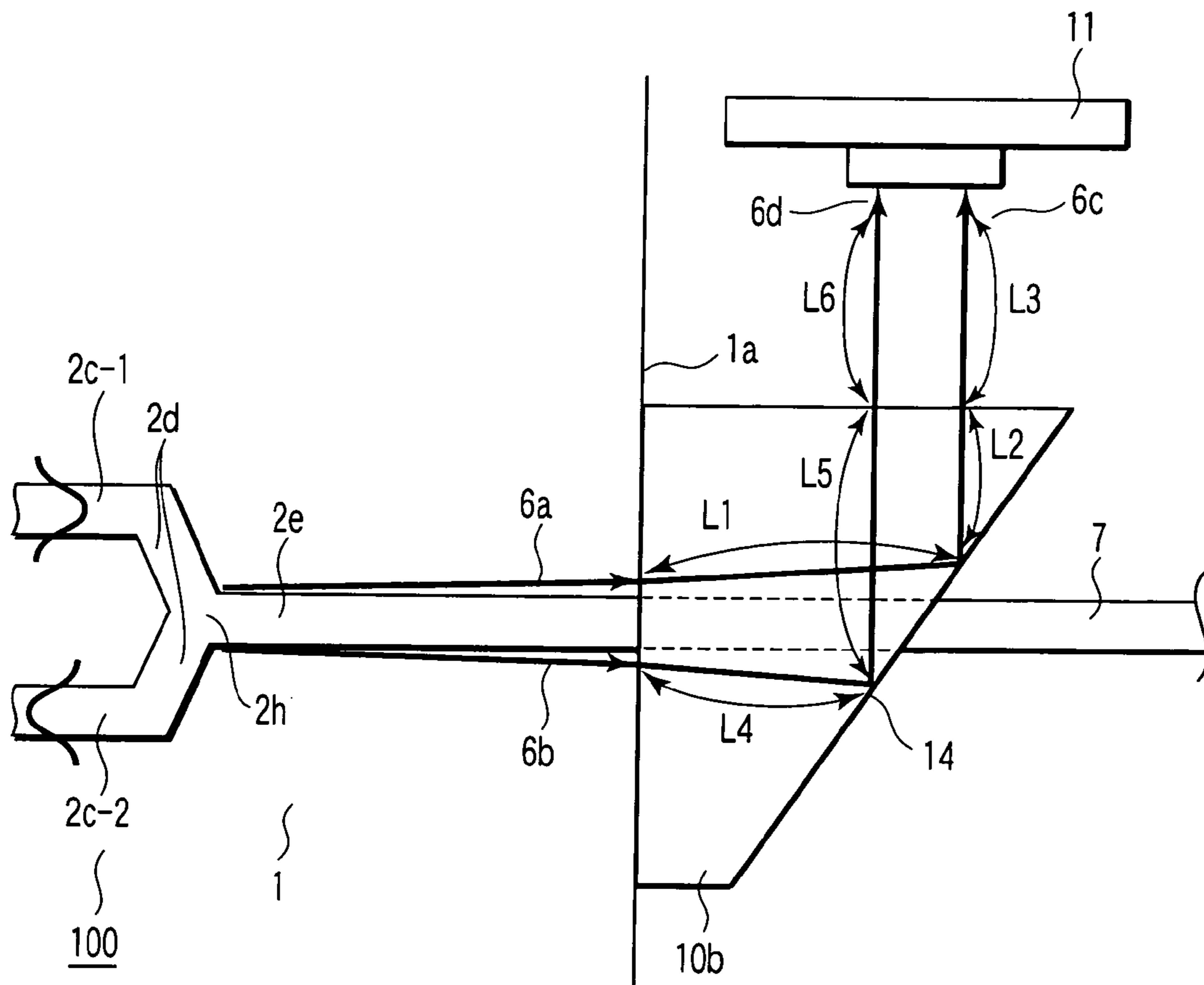
FIG. 17 (PRIOR ART)
