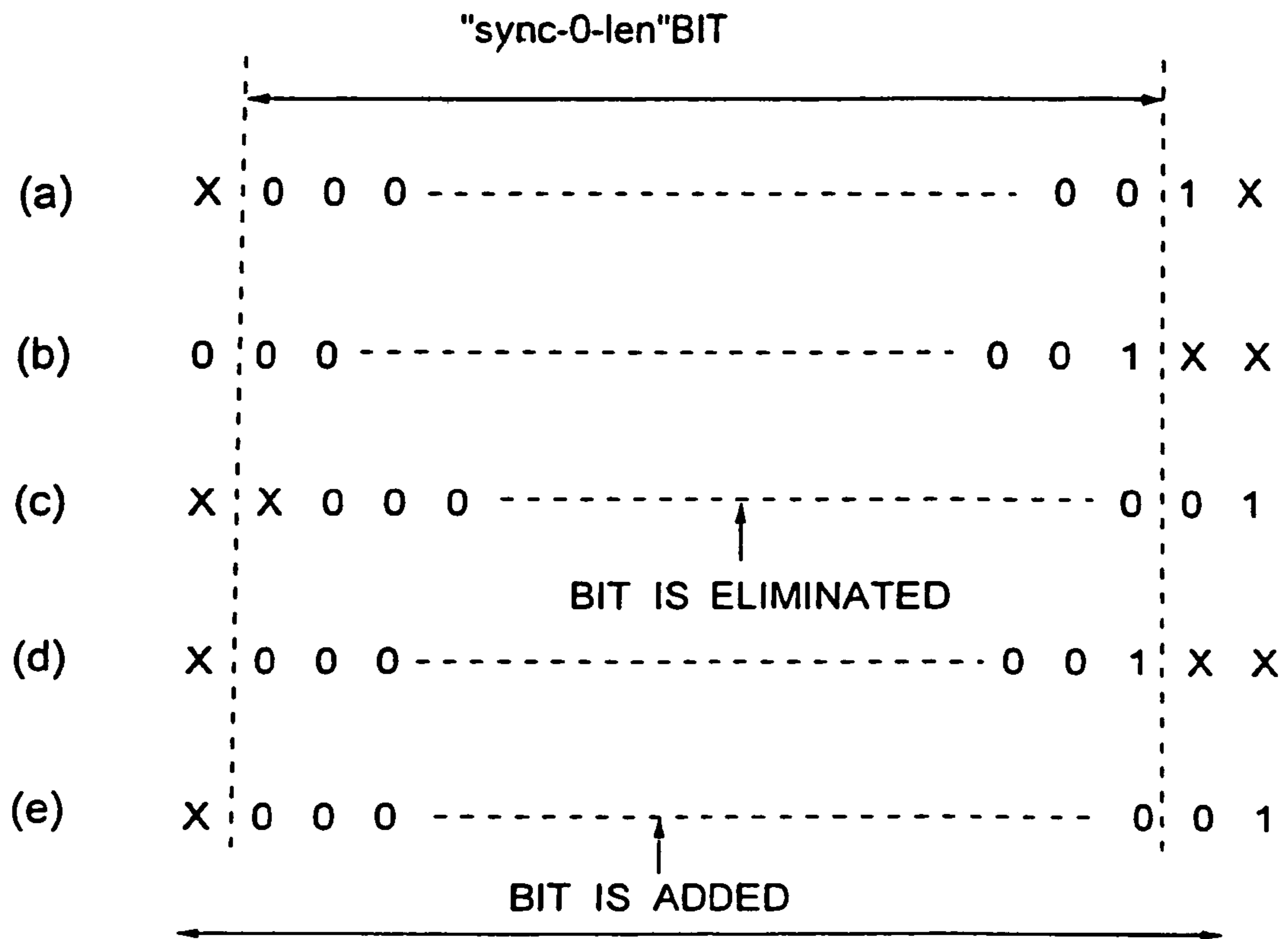
SYNCHRONIZATION CODE DETECTION WINDOW OF "sync-0-len+2"BIT
