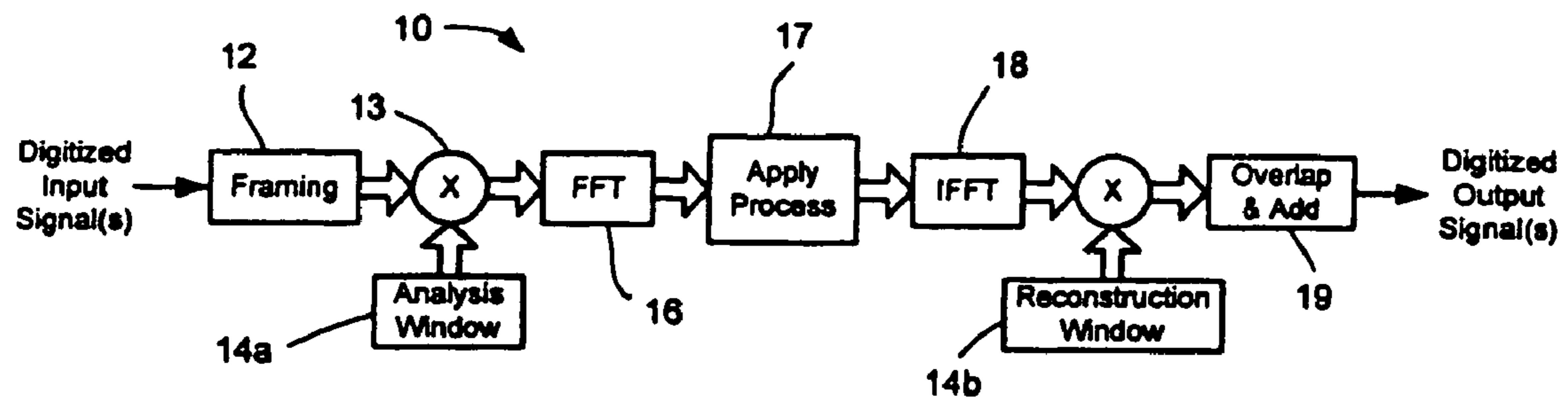
FIG. 1 PRIOR ART
