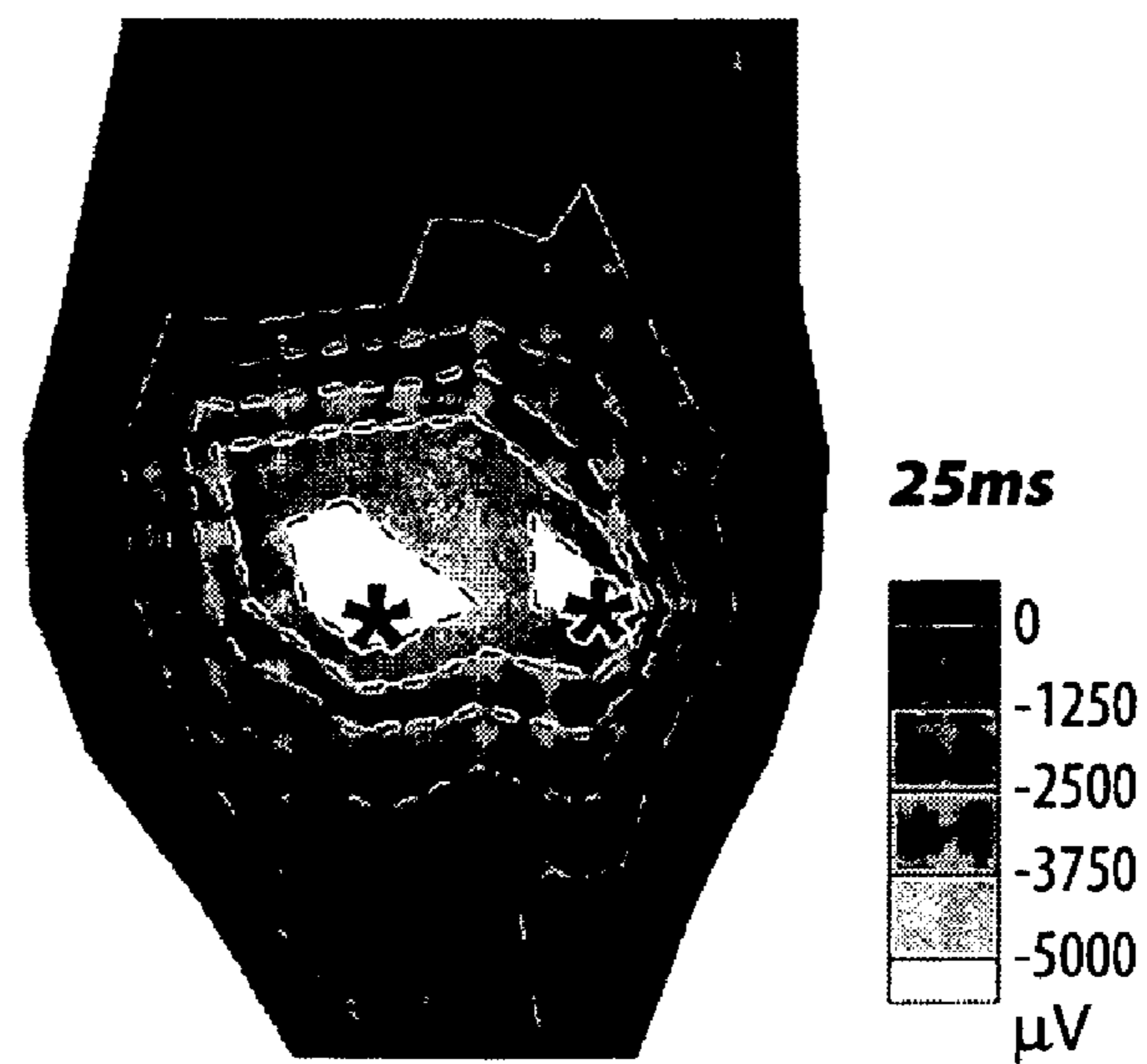
Tikhonov - GMRes
