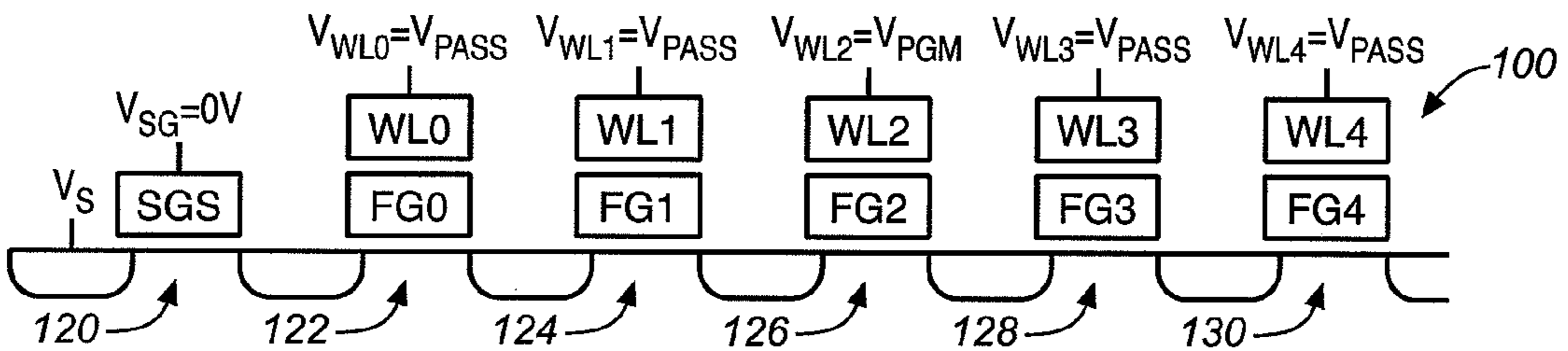
FIG. 4C (PRIOR ART)
