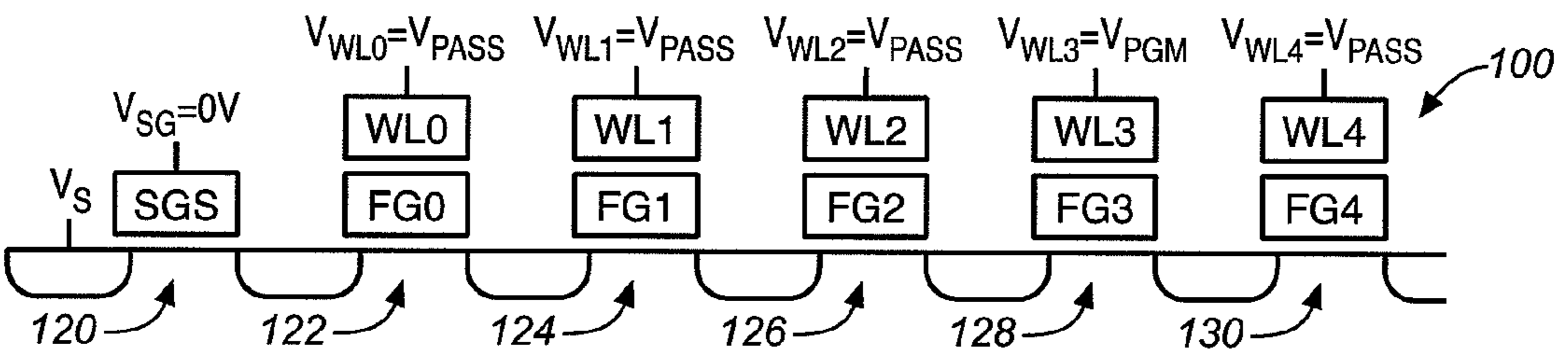
FIG. 4D (PRIOR ART)
