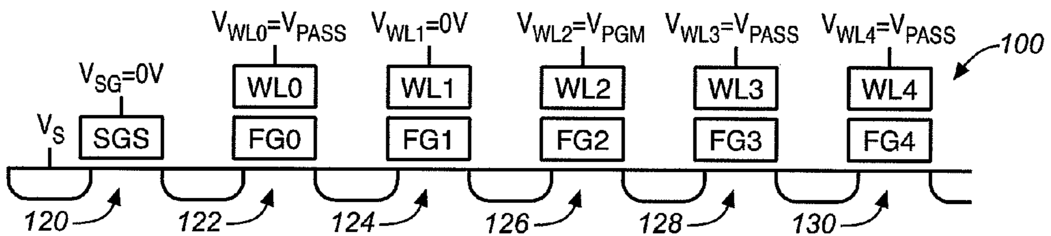
FIG. 6C (PRIOR ART)
