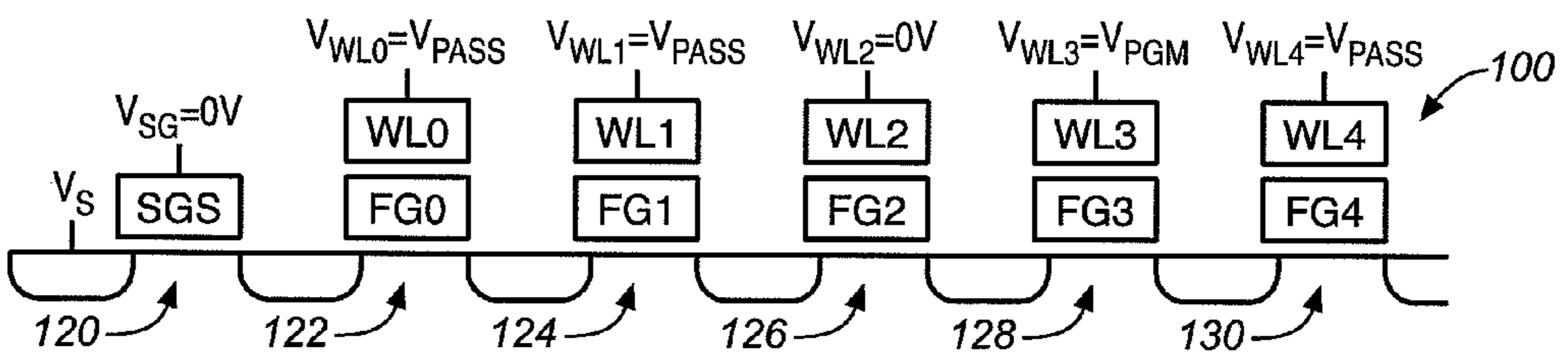
FIG. 6D (PRIOR ART)
