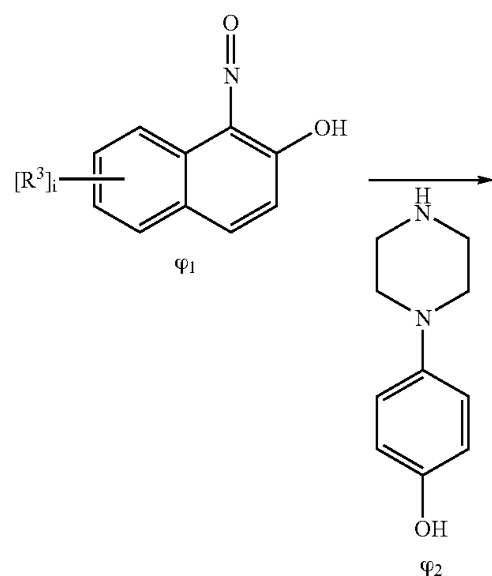
Reaction Sequence J
