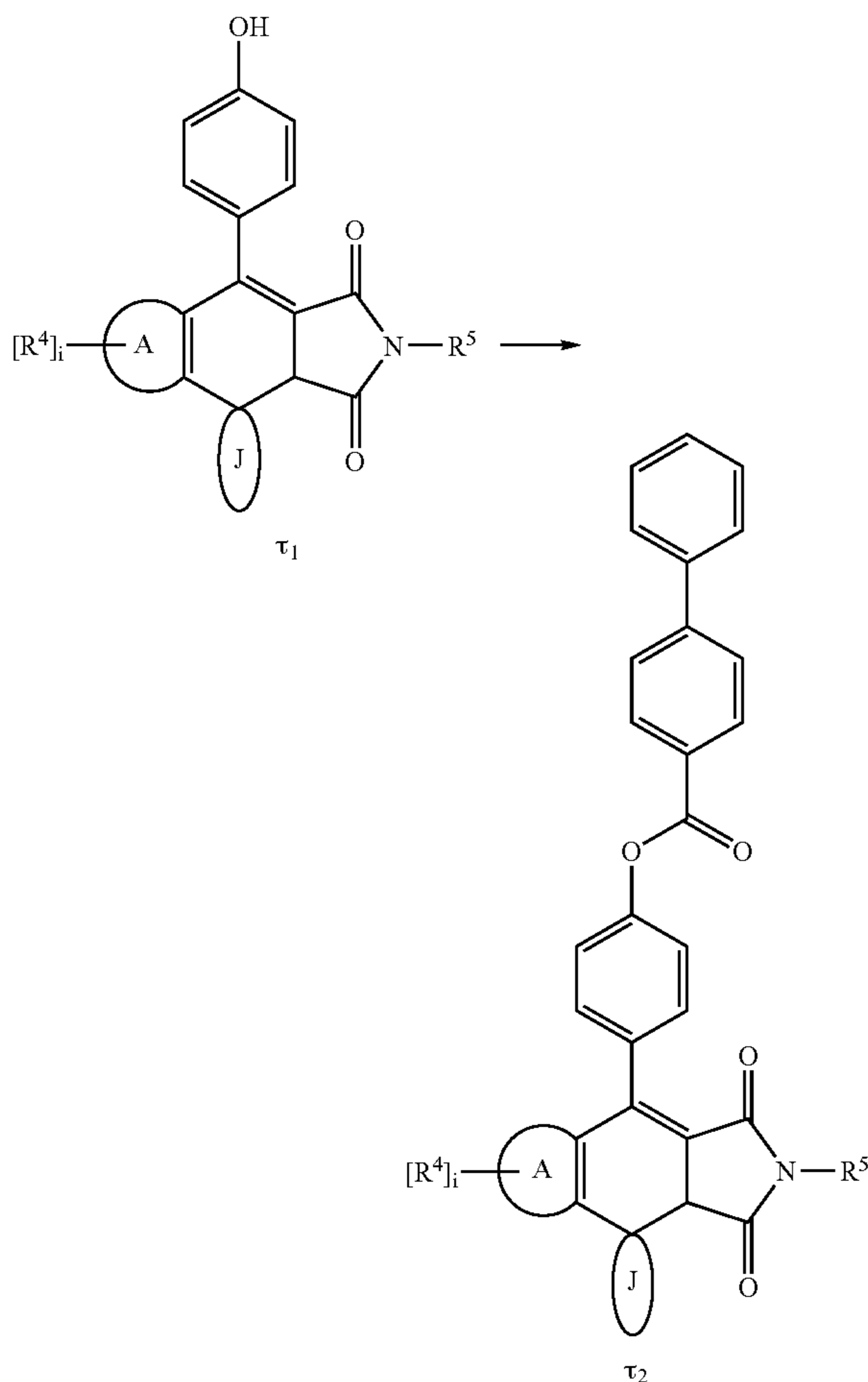
Reaction Scheme T
