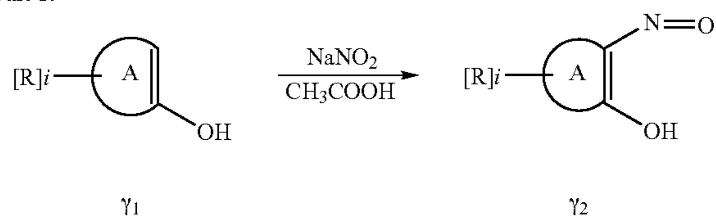
Reaction Sequence G
