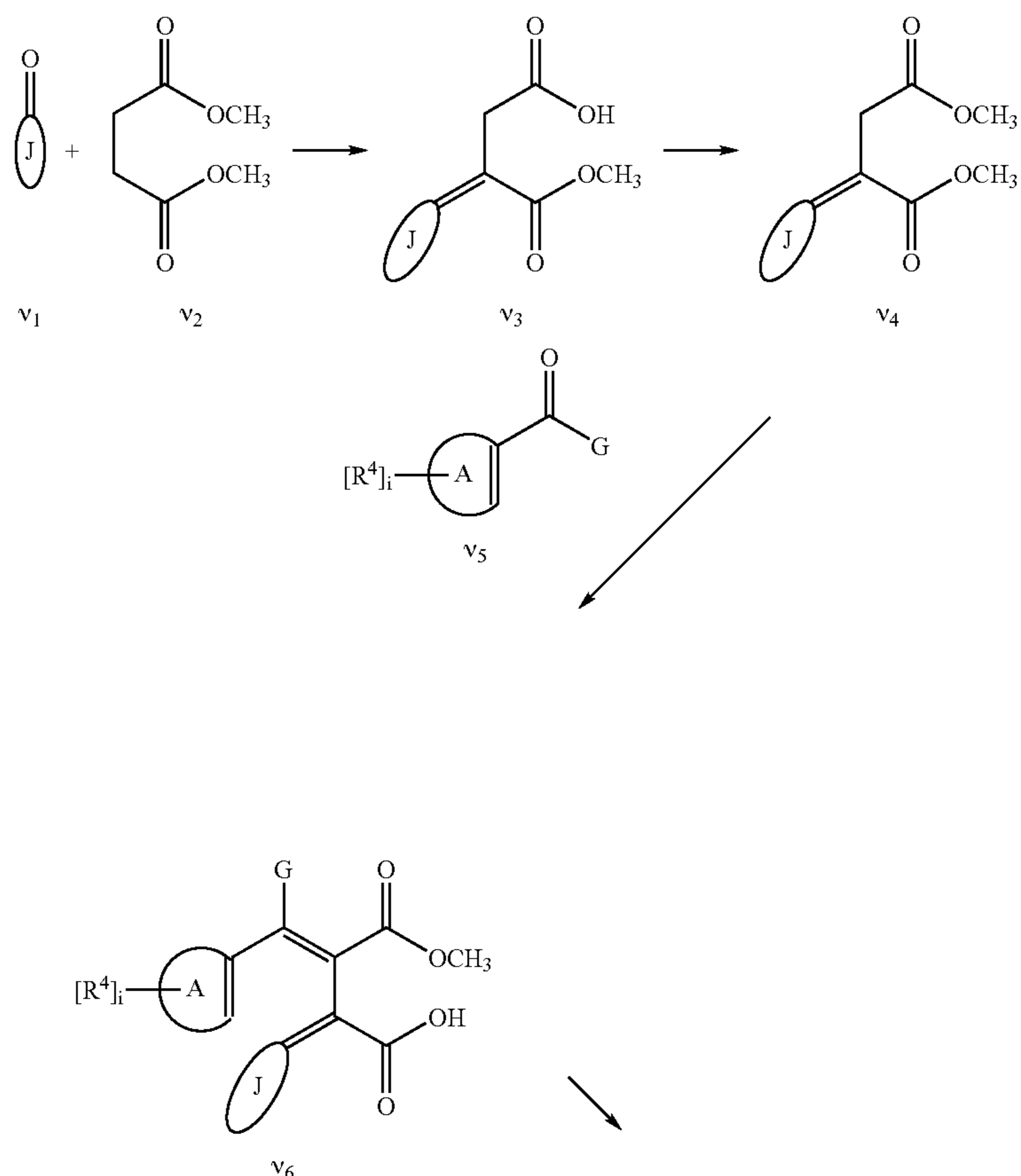
Reaction Sequence N
