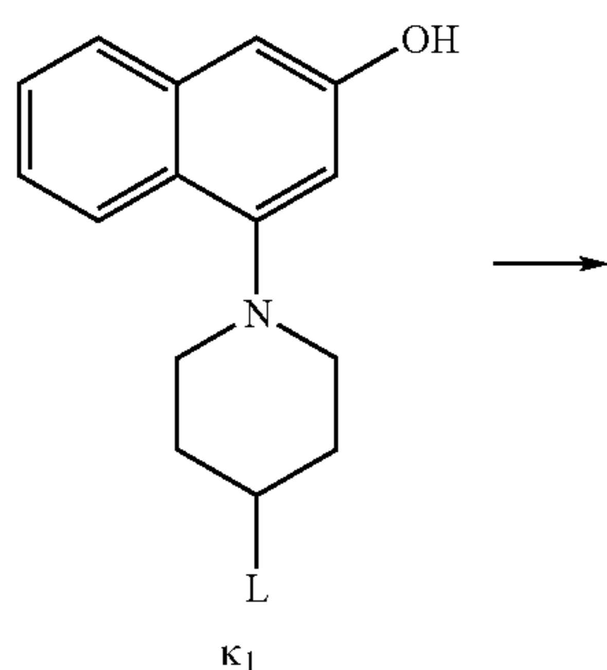
Reaction Sequence K
