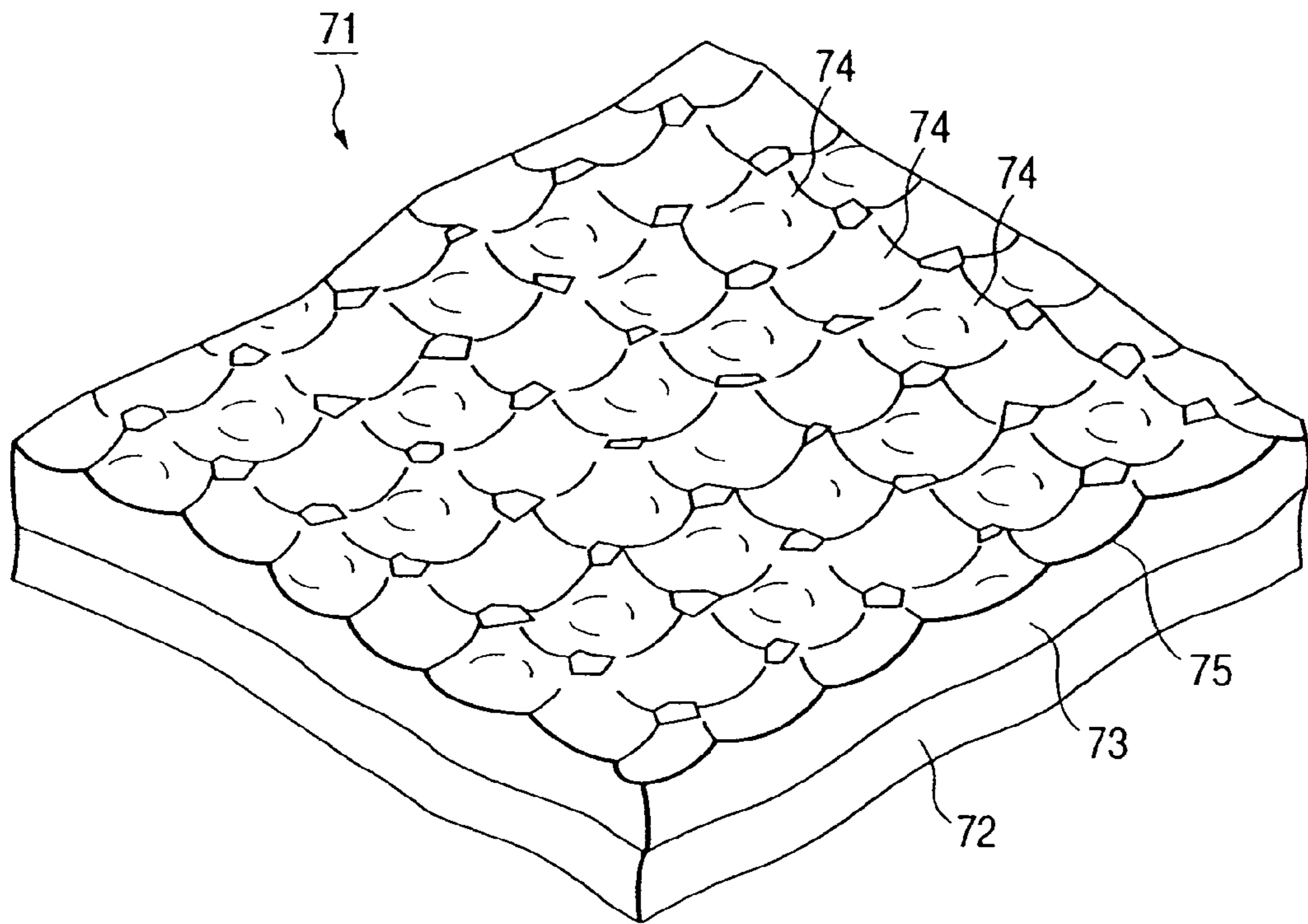
FIG. 15 PRIOR ART
