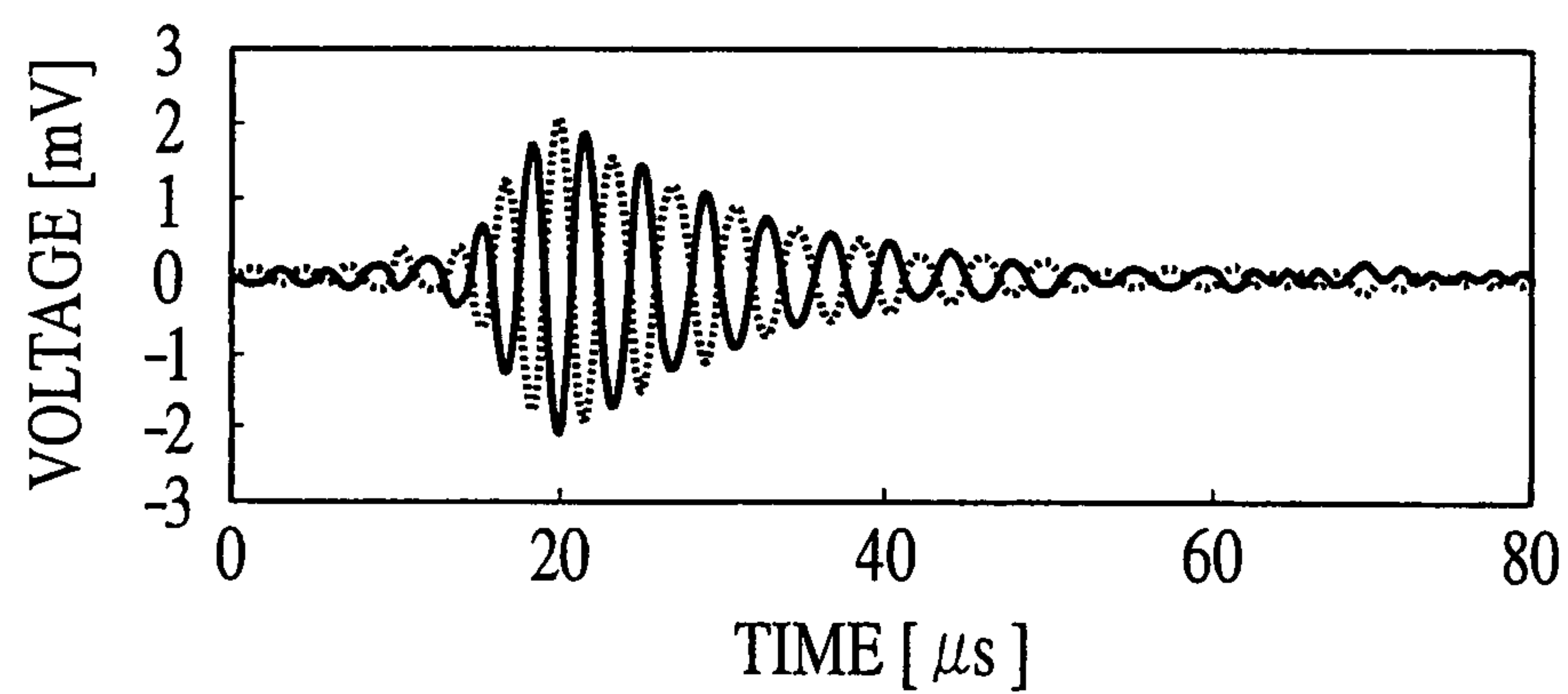
FIG. 9A \theta = 0^\circ (AXIS DIRECTION)
