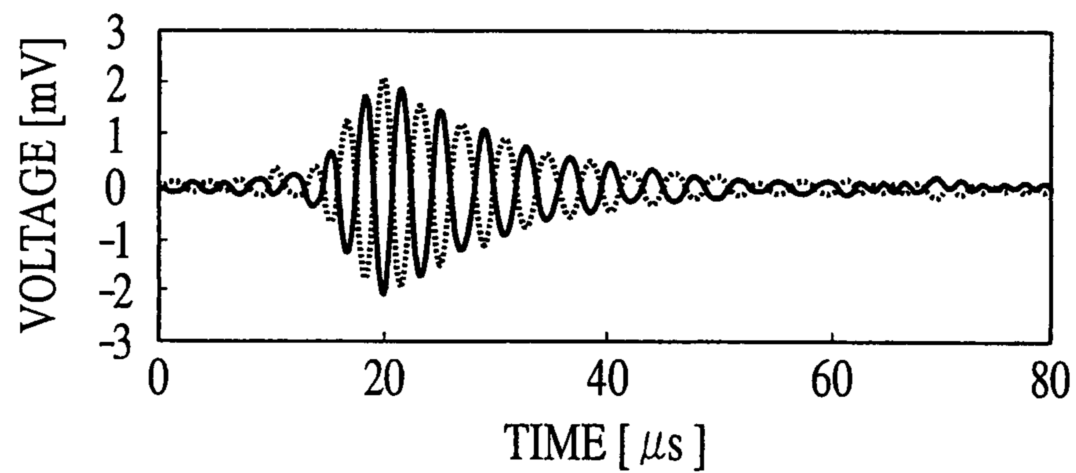
FIG.9A \theta = 0^\circ (AXIS DIRECTION)
