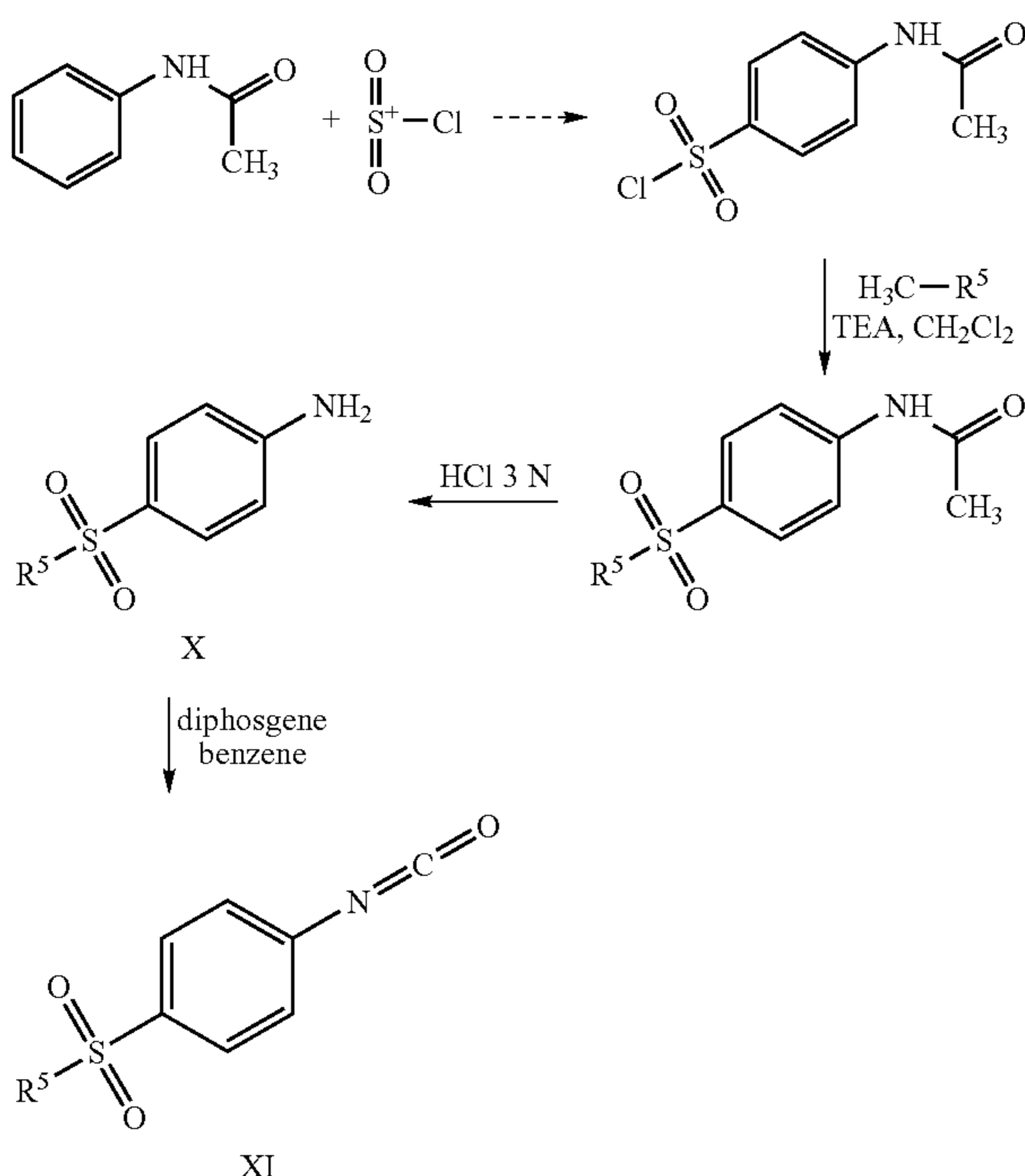
Scheme XI: General procedures for the preparation of sulfonyl-phenyl-isocyanates
