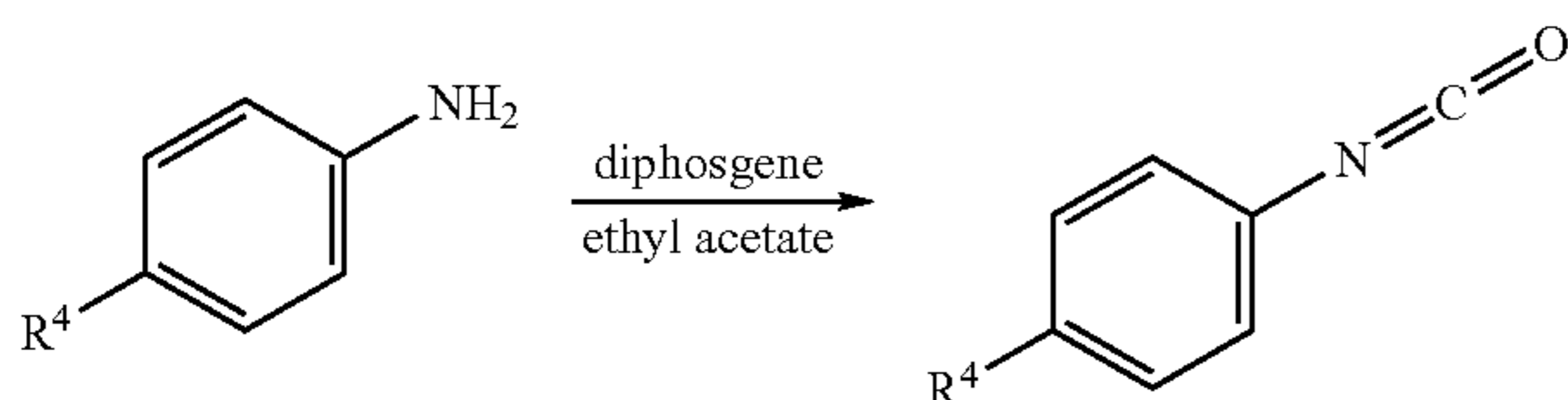
Scheme X: General procedures for the preparation of phenyl-isocyanates
