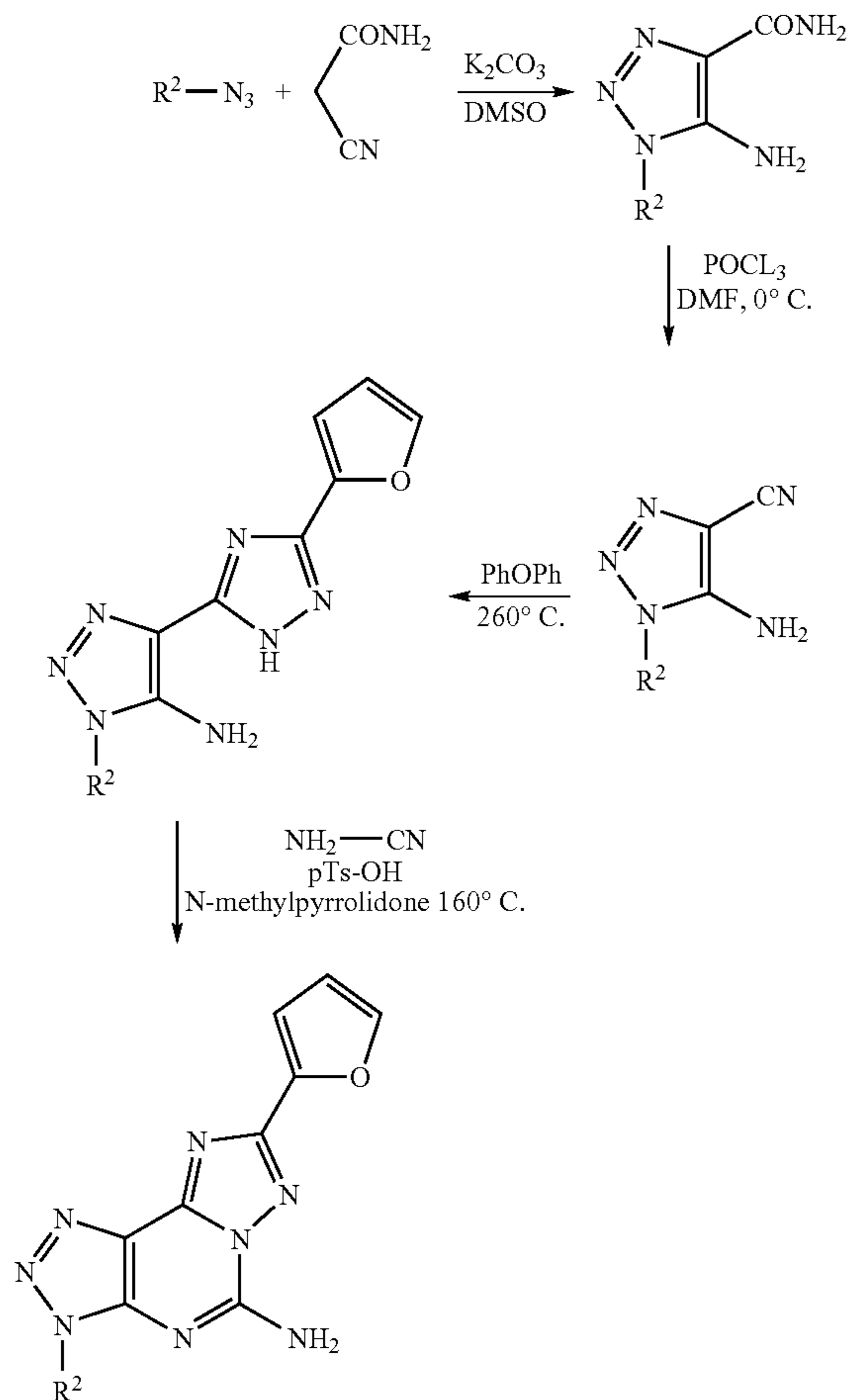
Scheme III Synthesis of 5-amino-7-substituted-2-(2-furyl)-1,2,3-triazolo-[5,4-e]-1,2,4-triazolo[1,5-c]pyrimidine derivatives
