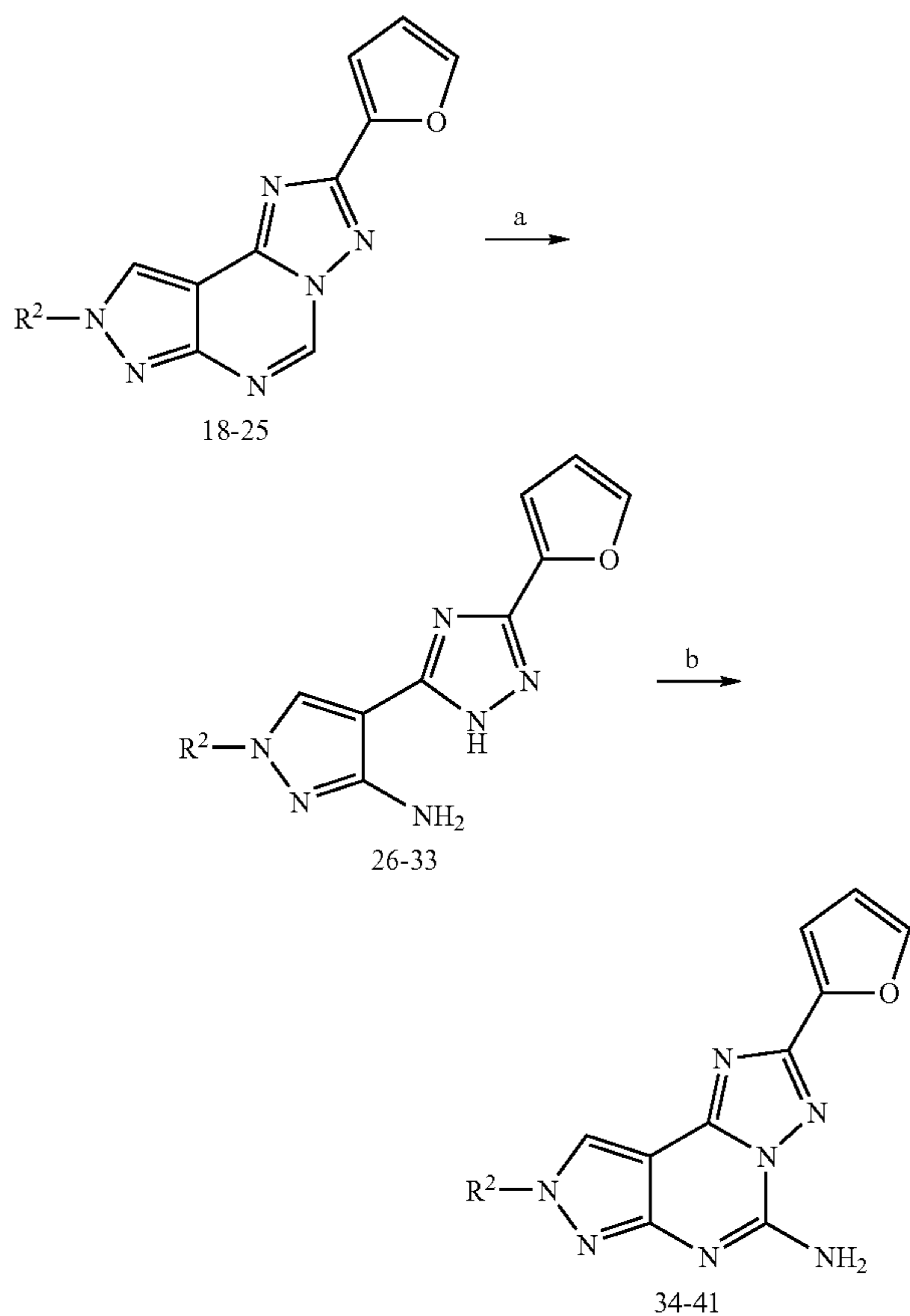
Scheme VII: General procedures for the preparation of 5-Amino-8-(ar)alkyl-2-(2-furyl)-pyrazolo[4,3-e]1,2,4-triazolo[1,5-c]pyrimidine (Compounds 34-41)
