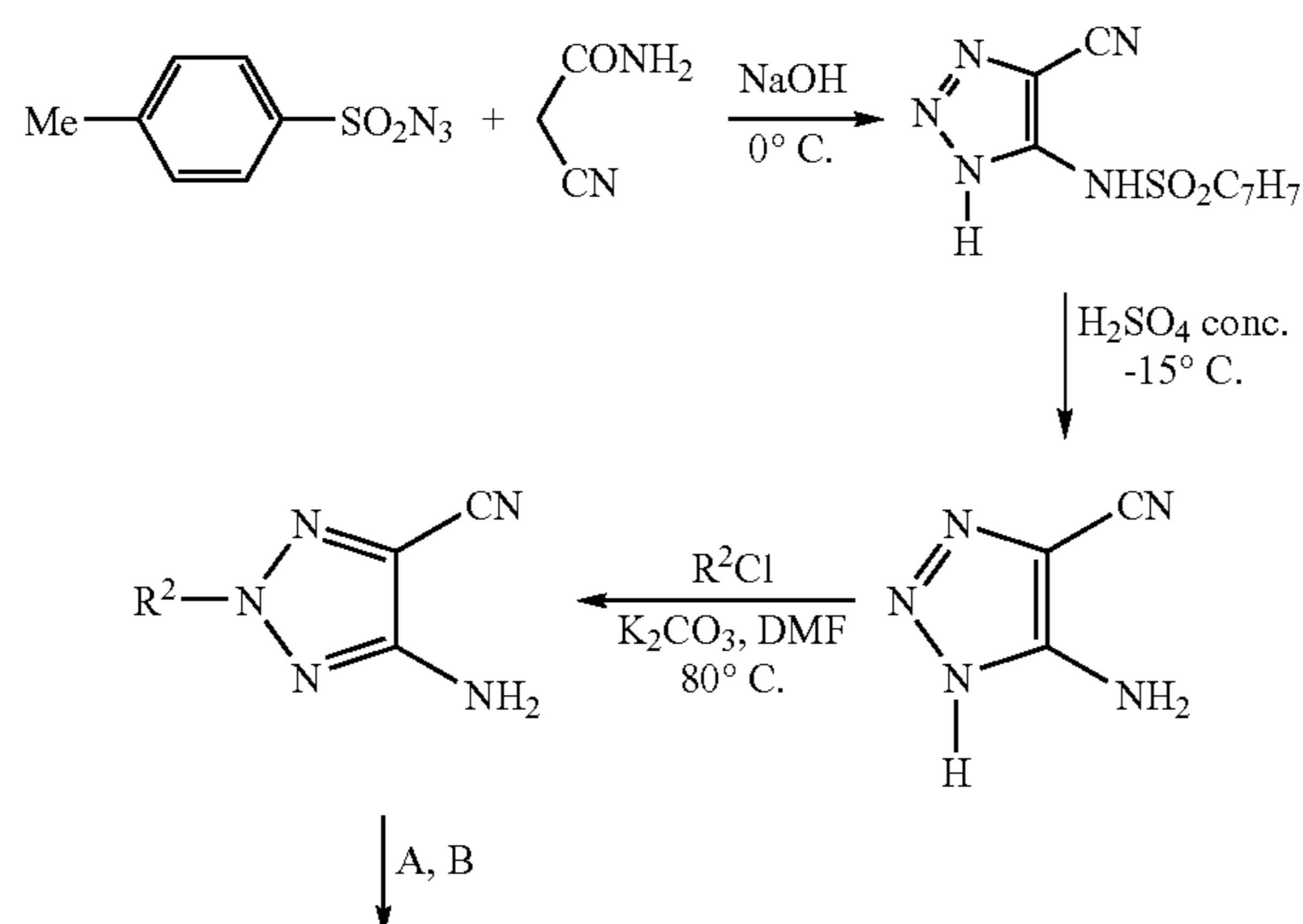
Scheme IV Synthesis of 5-amino-8-substituted-2-(2-furyl)-1,2,3-triazolo[5,4-e]1,2,4-triazolo[1,5-c]pyrimidine derivatives
