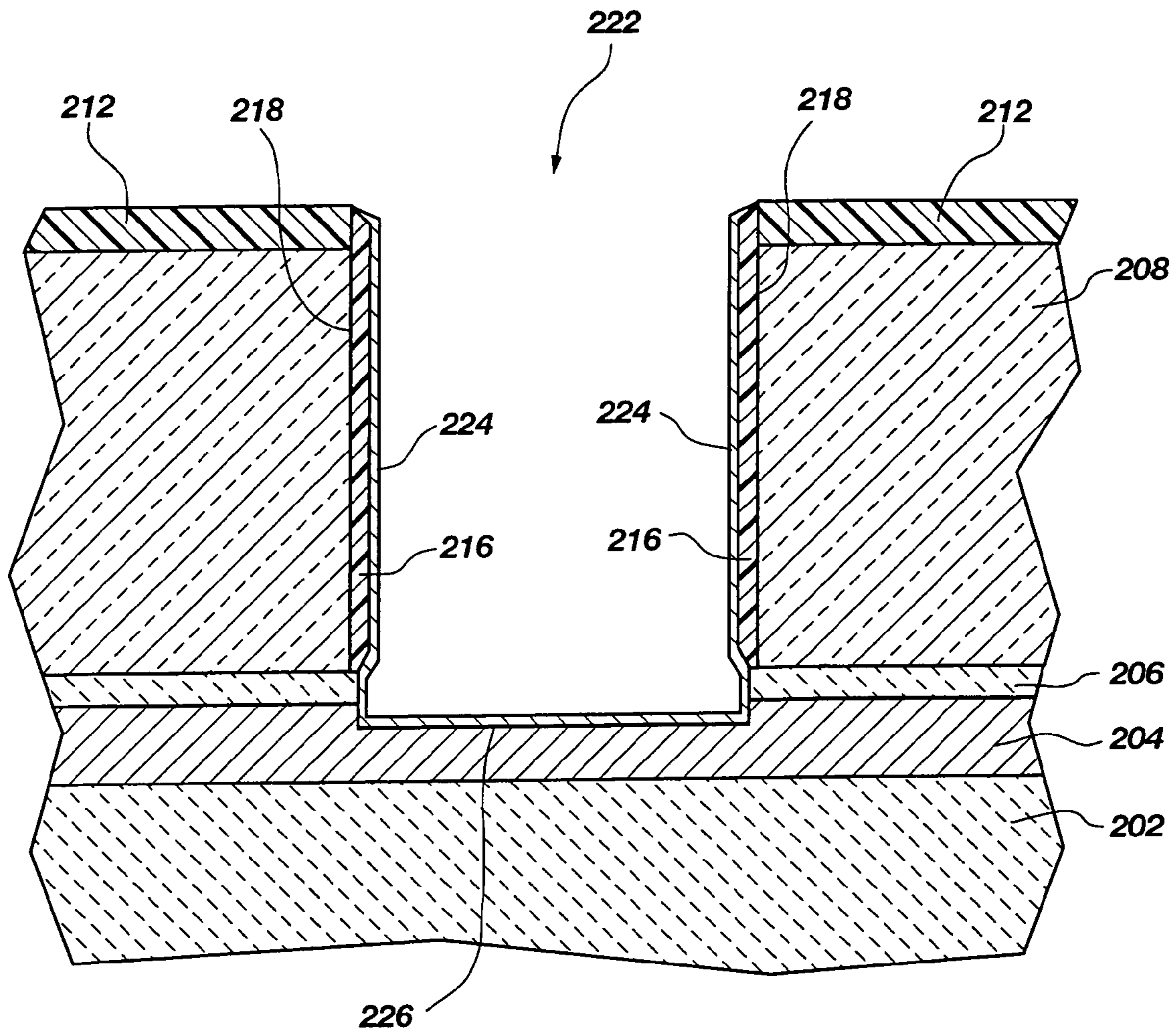
Fig. 14 (PRIOR ART)
