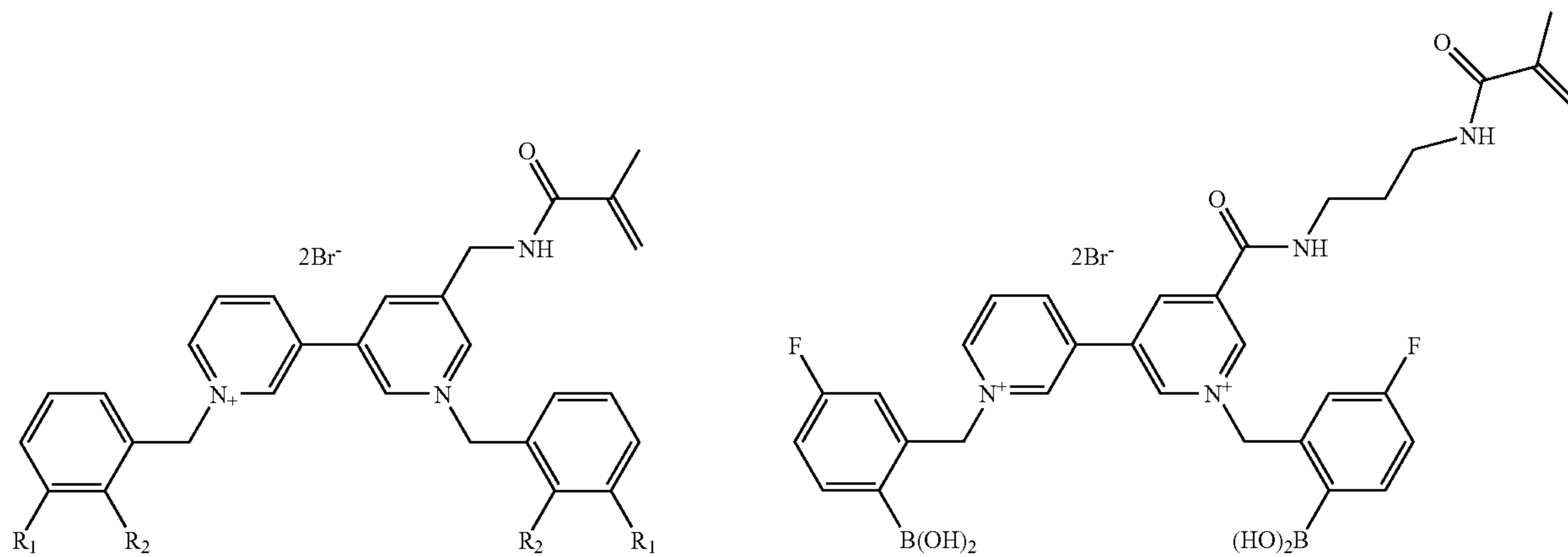
3,3'-oBBV; R_1 = H , R_2 = B(OH)_2 3,3'-mBBV; R_1 = B(OH)_2 , R_2 = H
