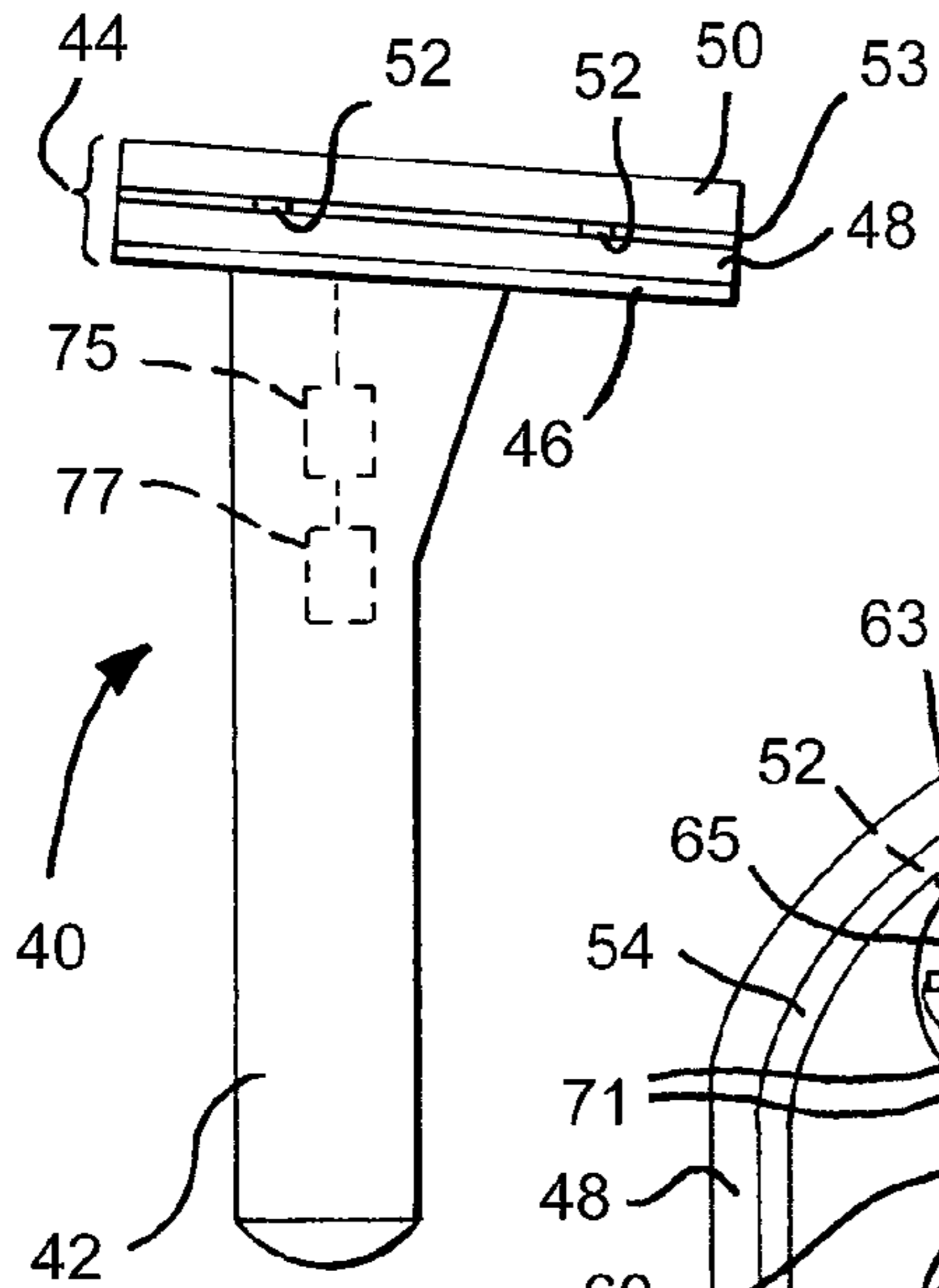
FIG. 2 (PRIOR ART)
