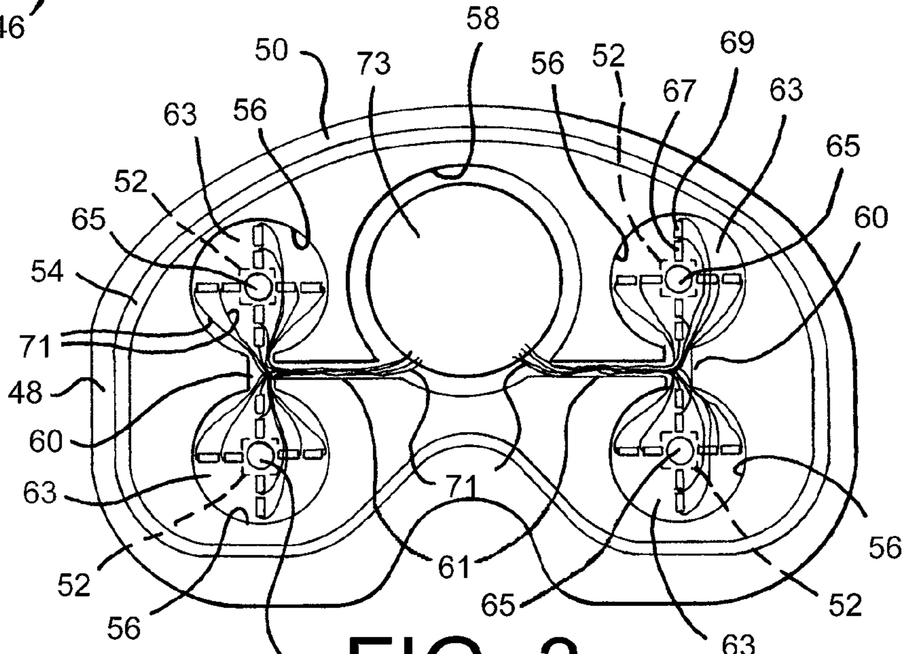
FIG. 2 (PRIOR ART)
