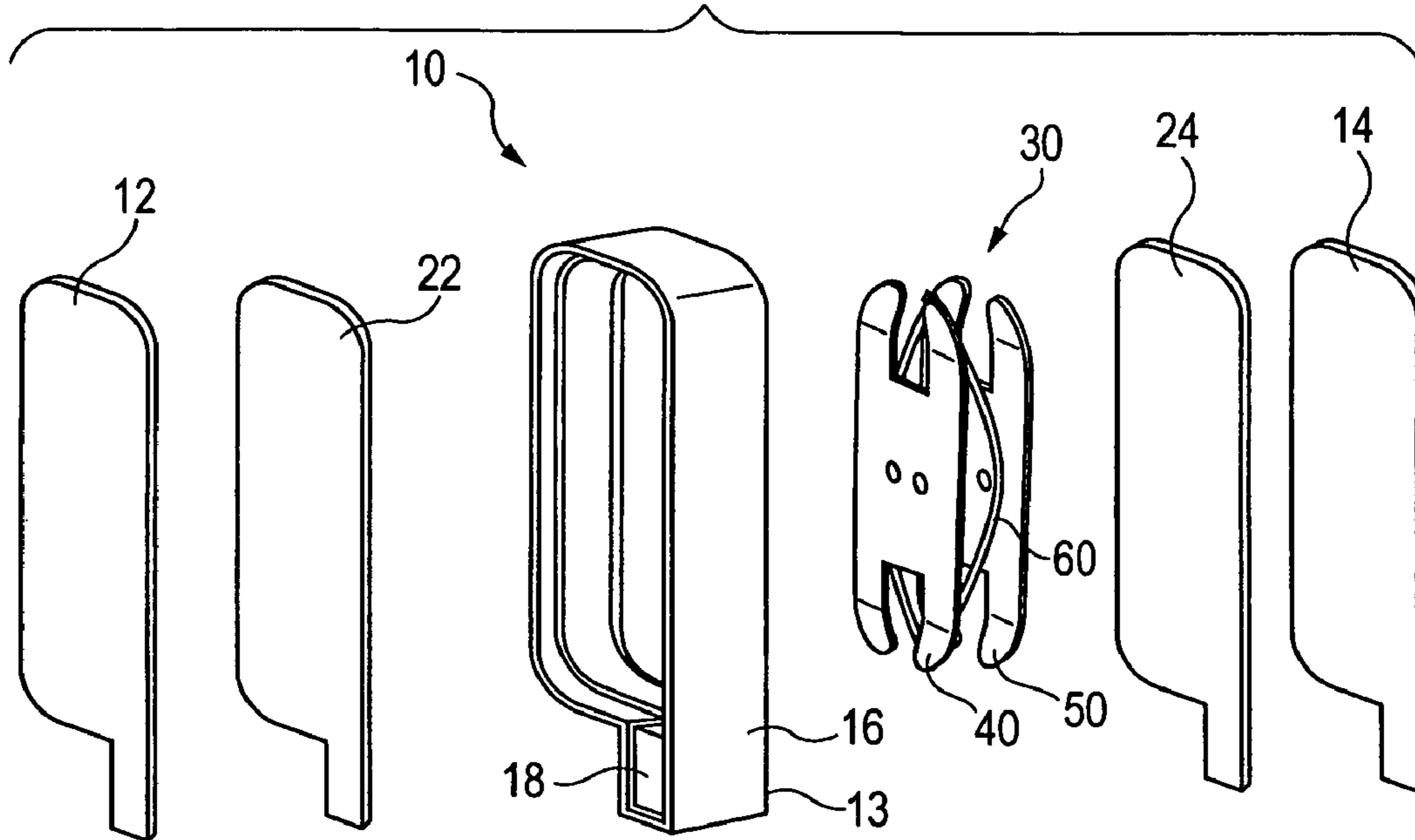
FIG. 6 PRIOR ART
