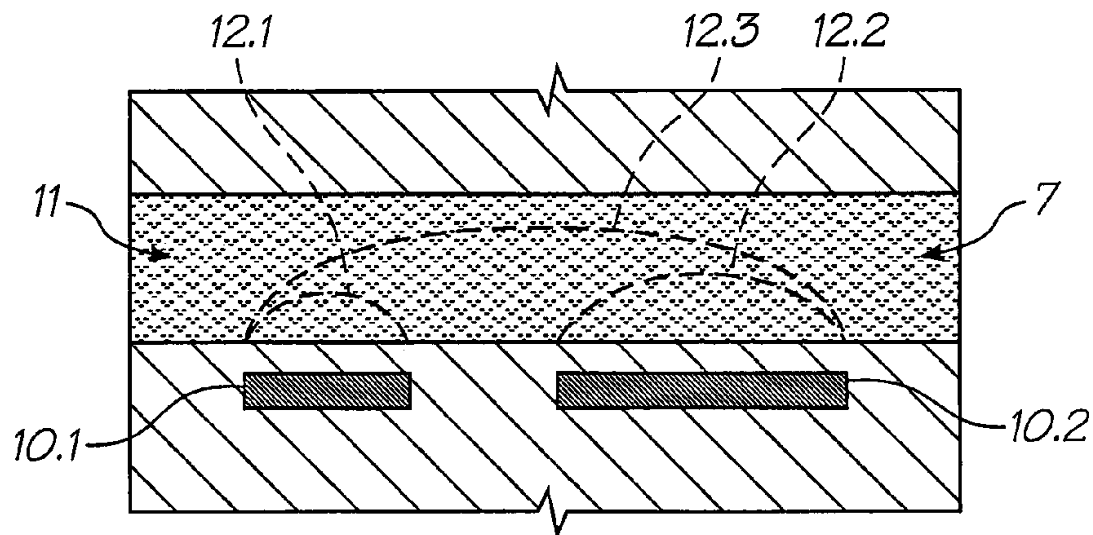
FIG. 52 (PRIOR ART)
