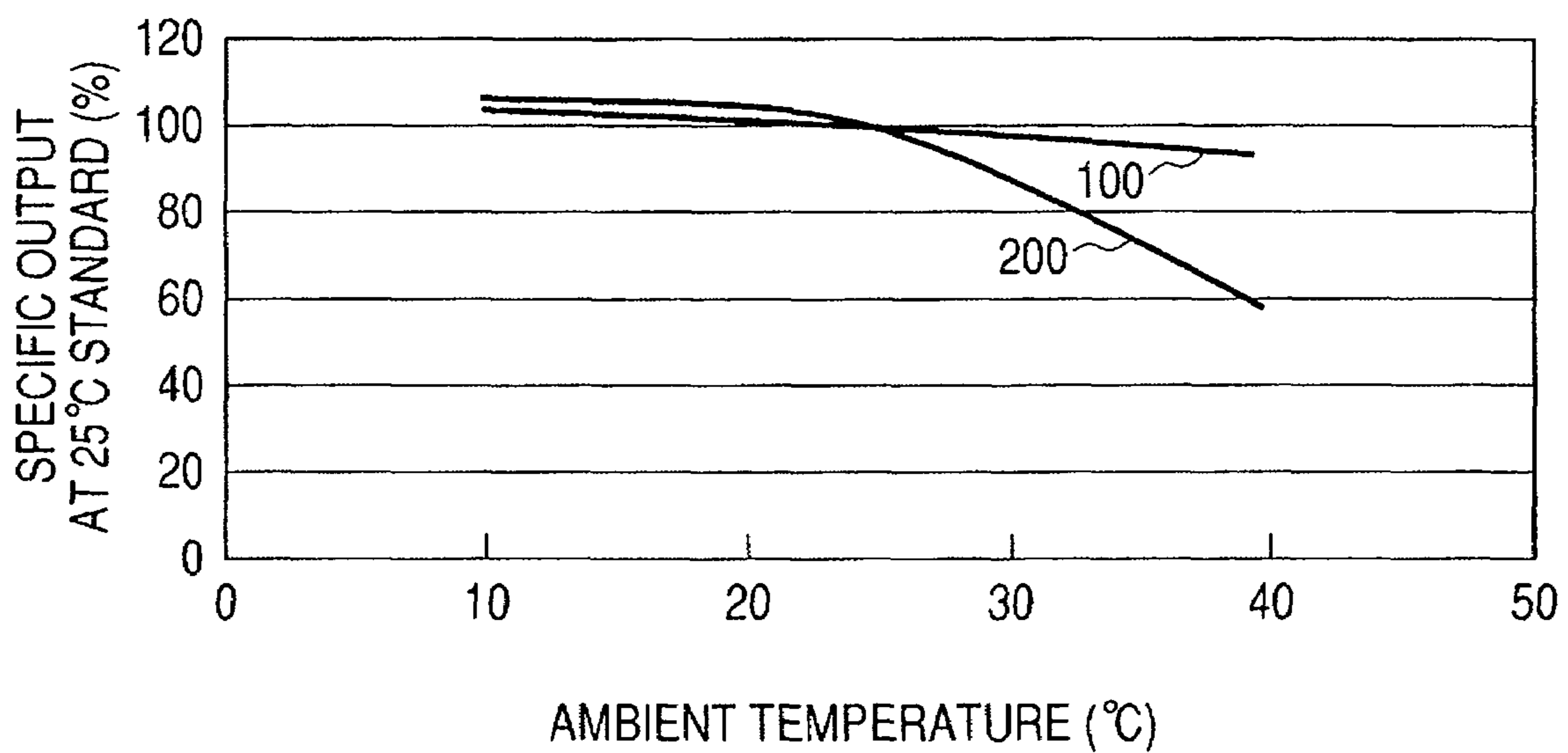
OUTPUT-TEMPERATURE CHARACTERISTIC GRAPH UNDER HUMIDITY OF 50%
