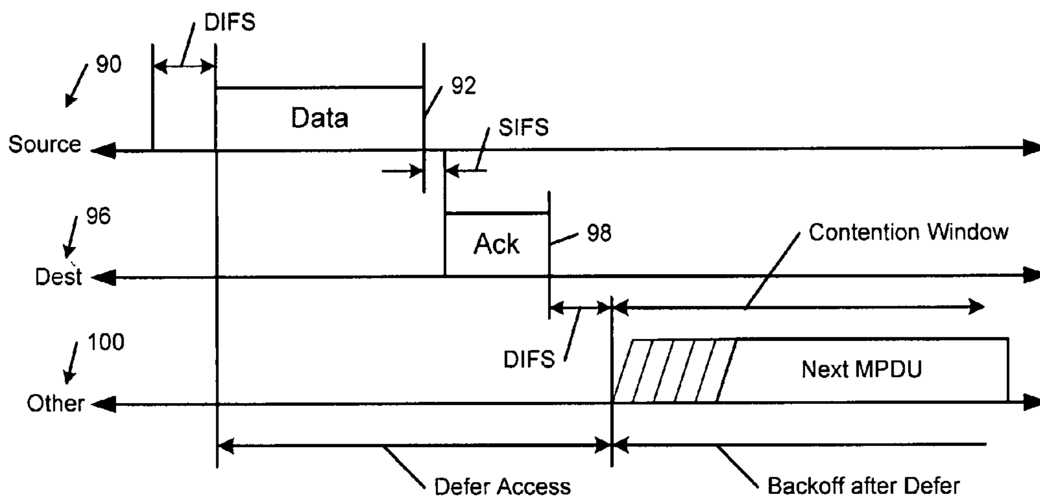
FIG. 6 Prior Art
