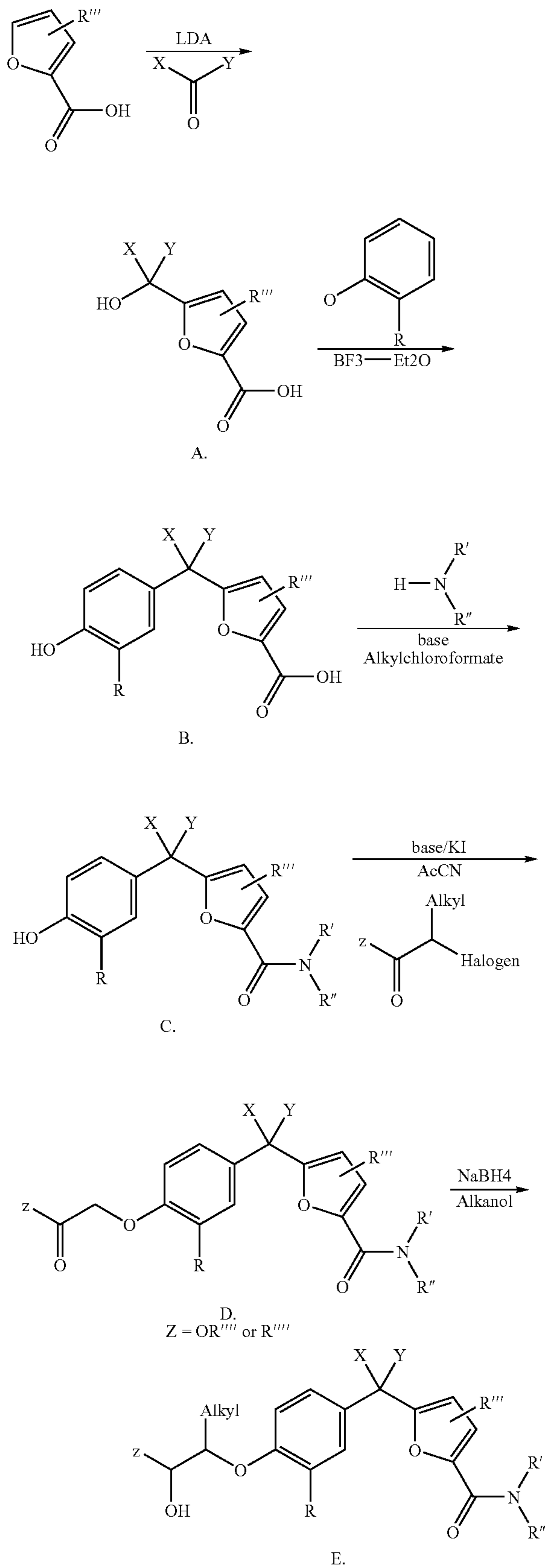
Scheme I
