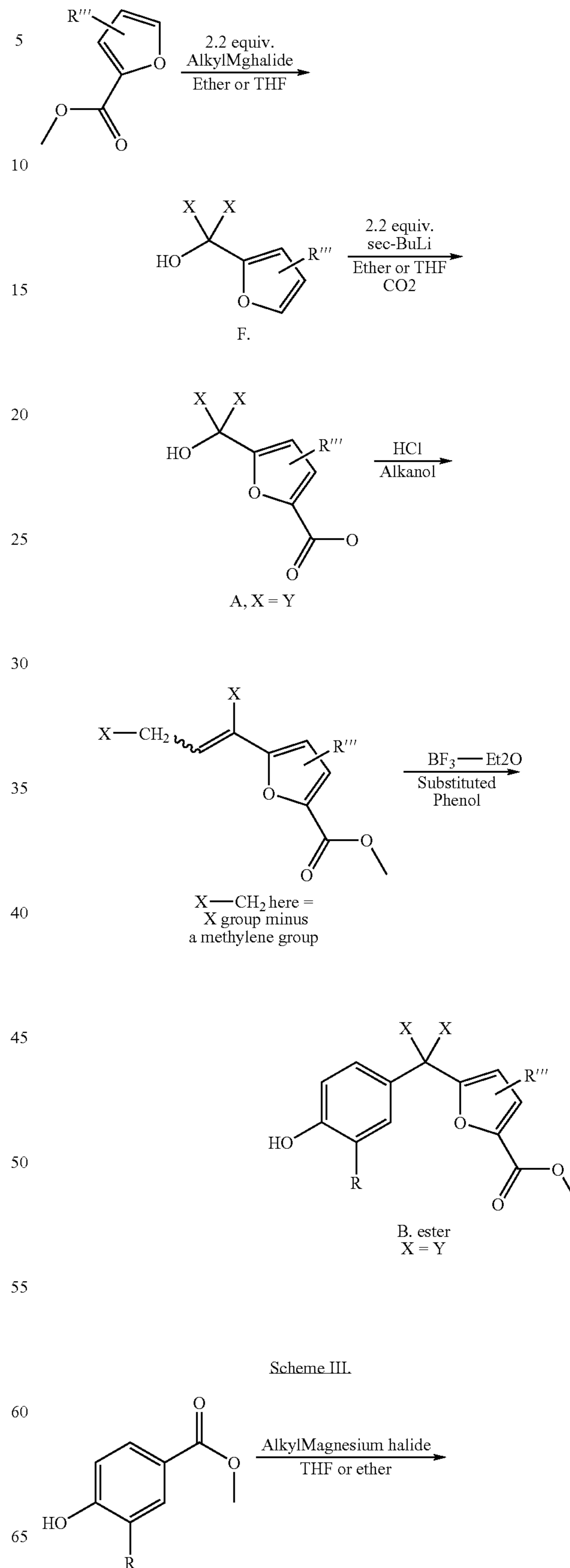
Scheme II.
