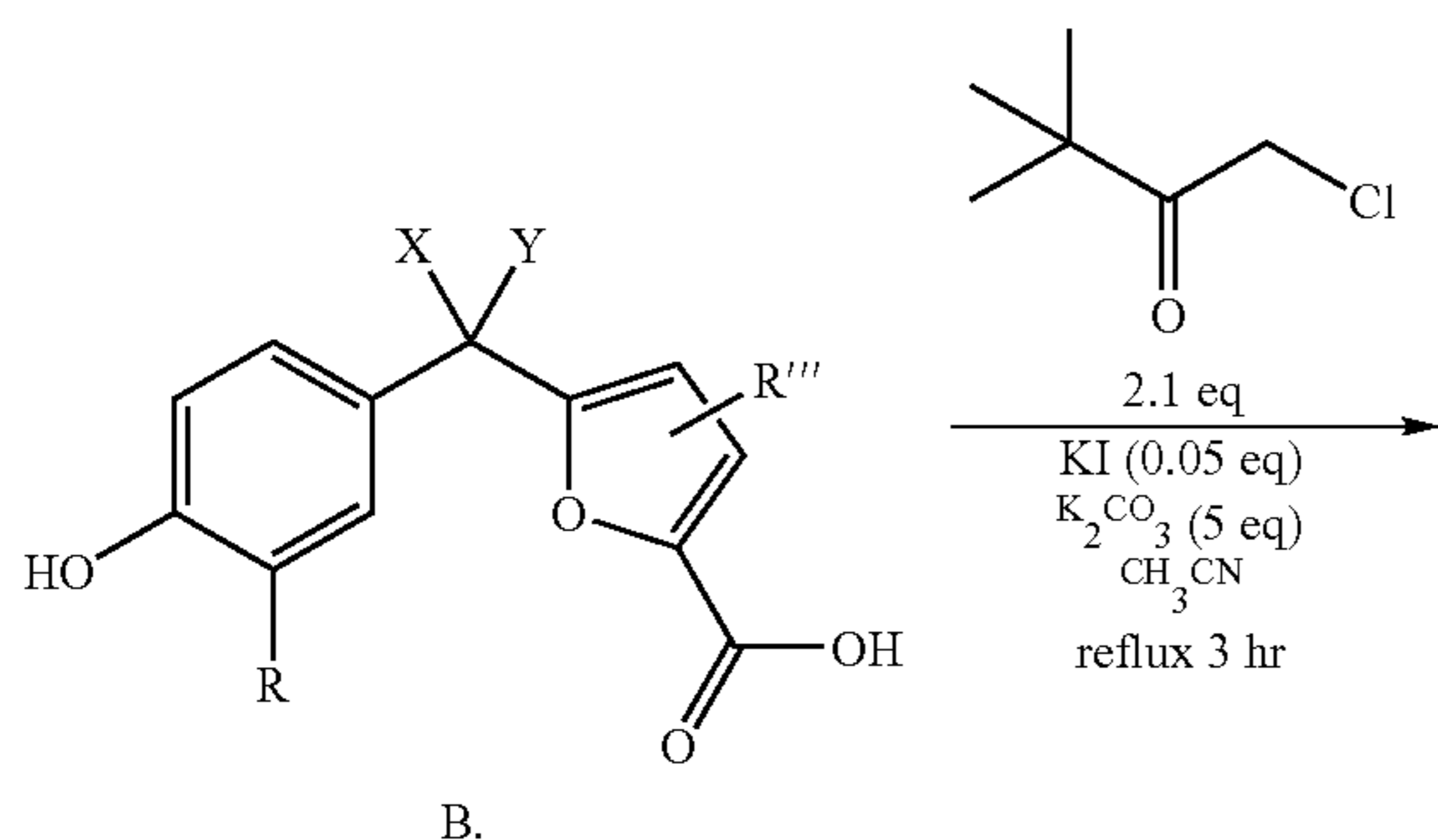
Scheme V
