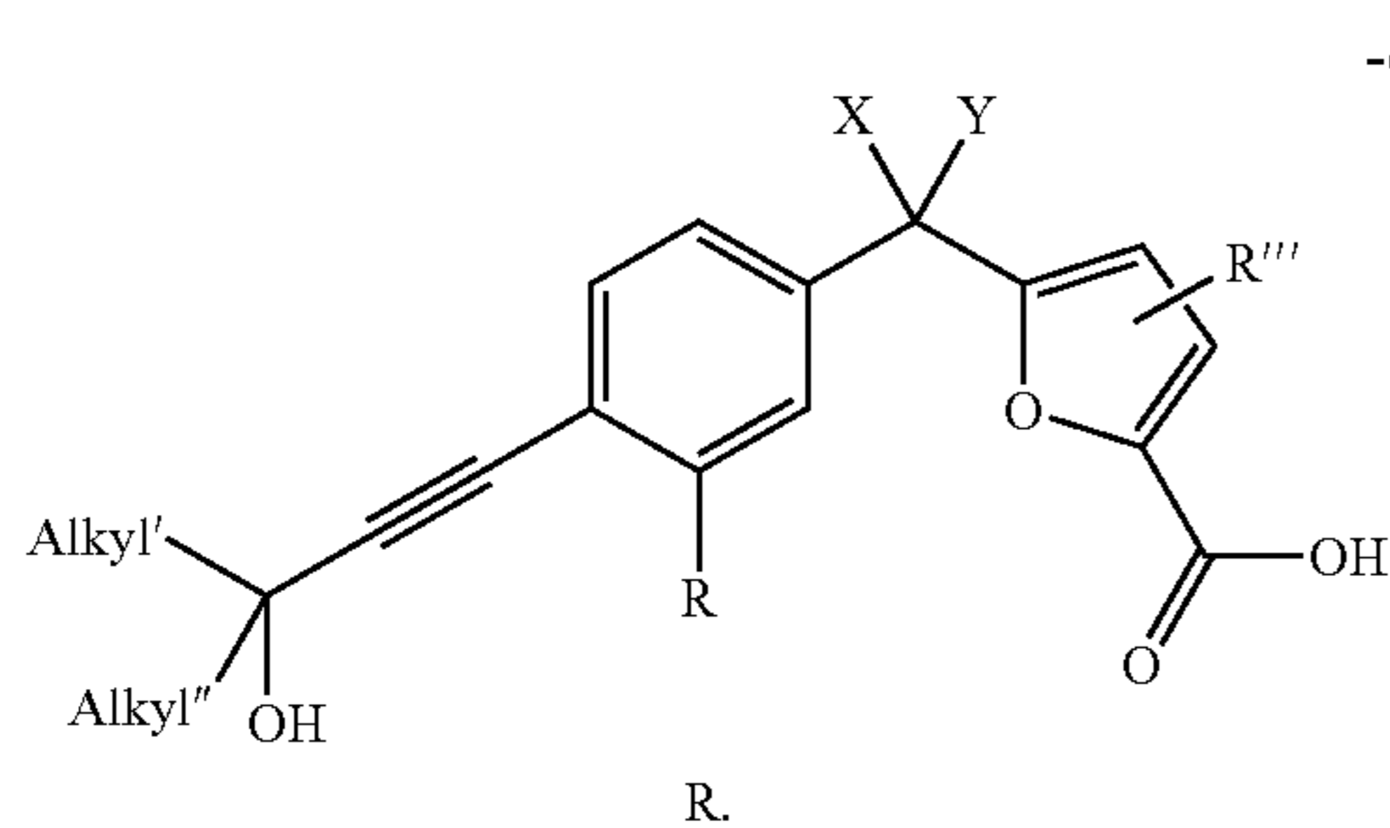
Scheme V
