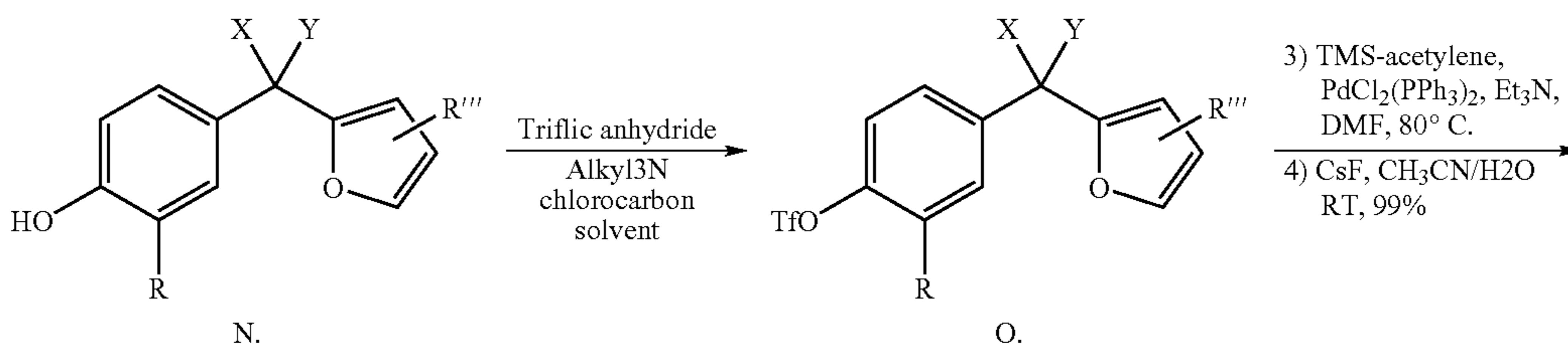
Scheme IV
