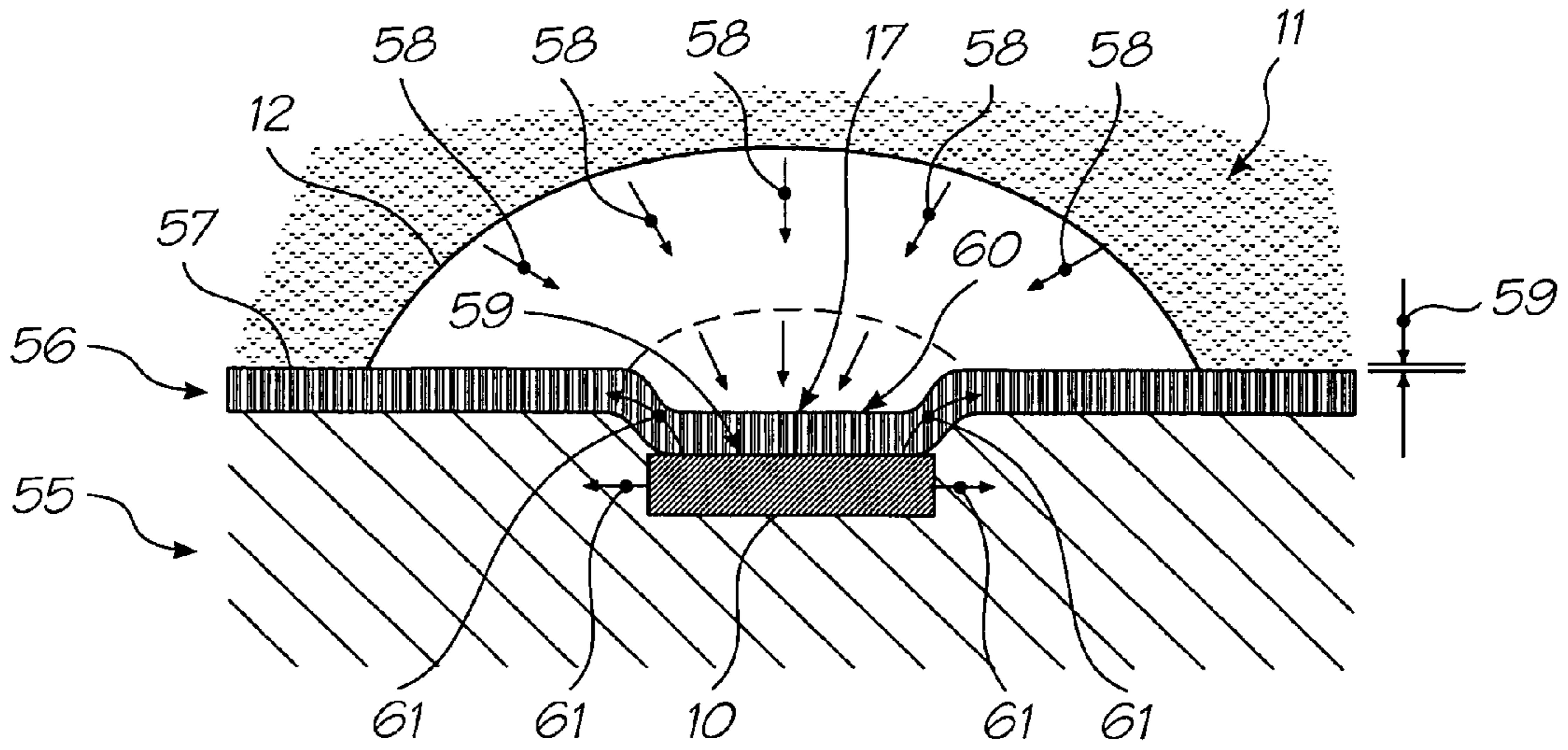
FIG. 47 (PRIOR ART)
