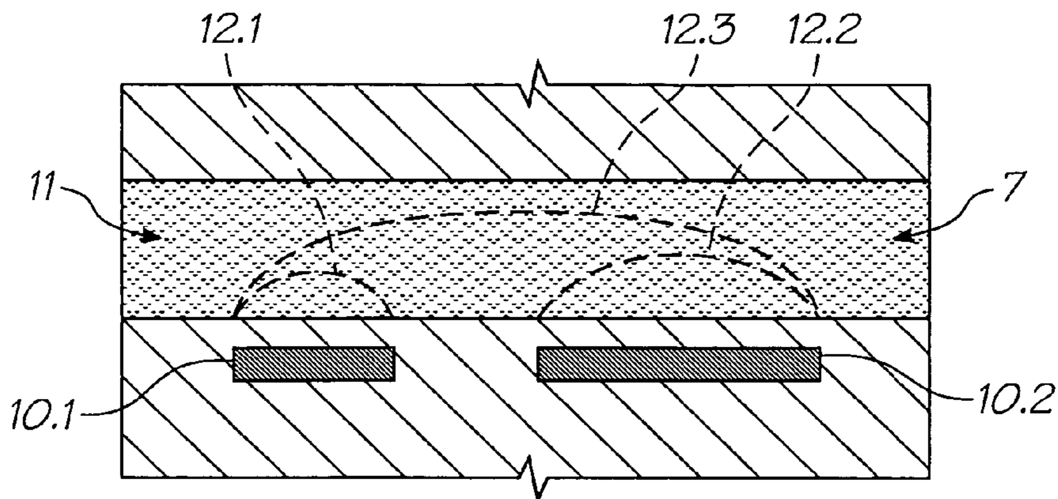
FIG. 52 (PRIOR ART)
