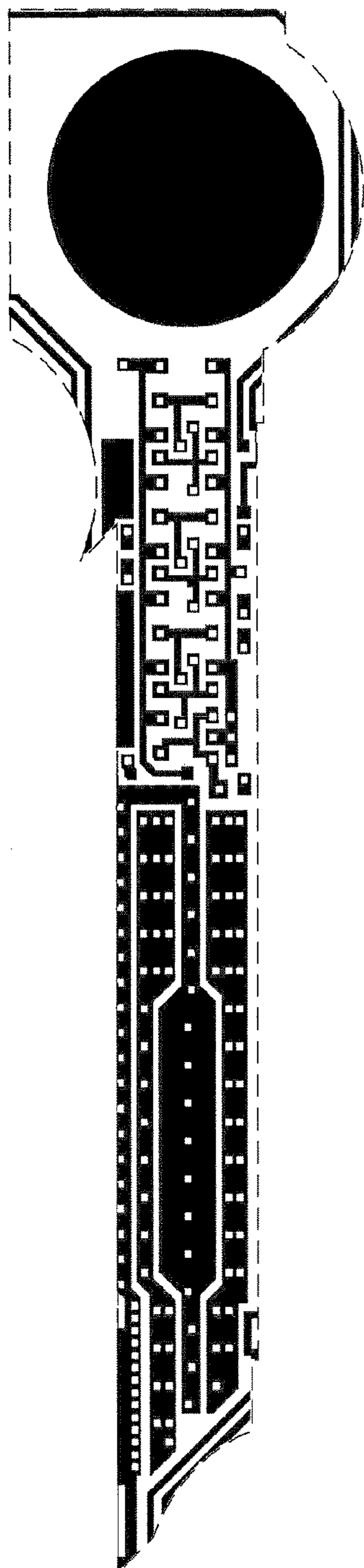
Metal 1 mask
