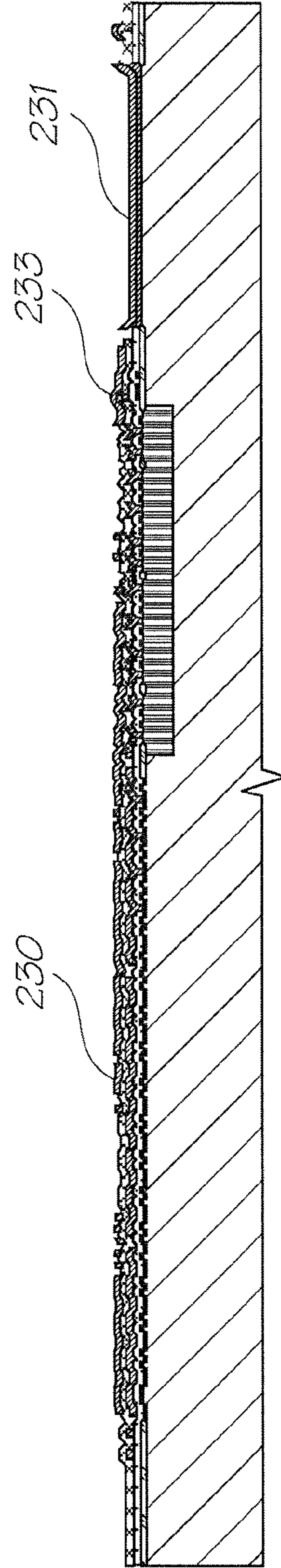
Deposit metal 2
