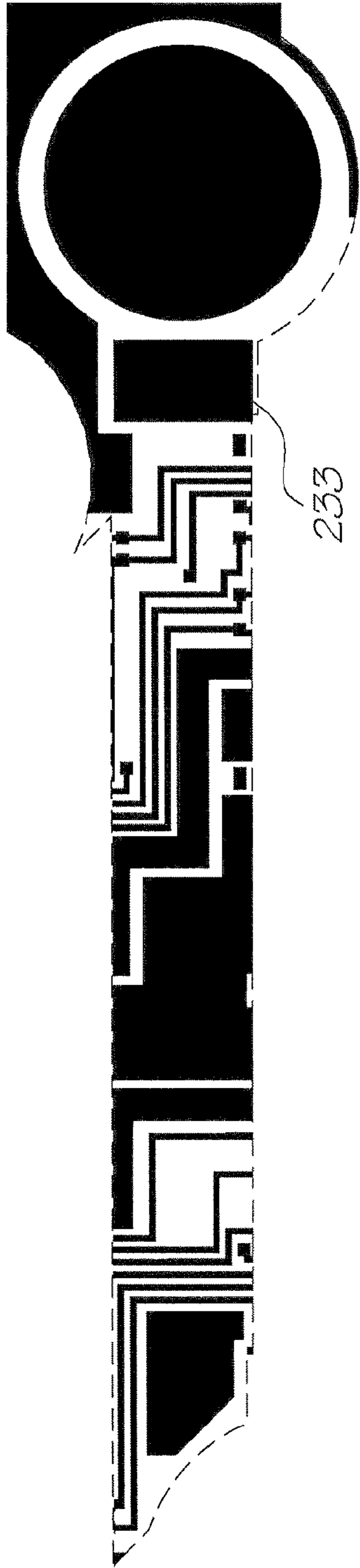
Metal 2 mask
