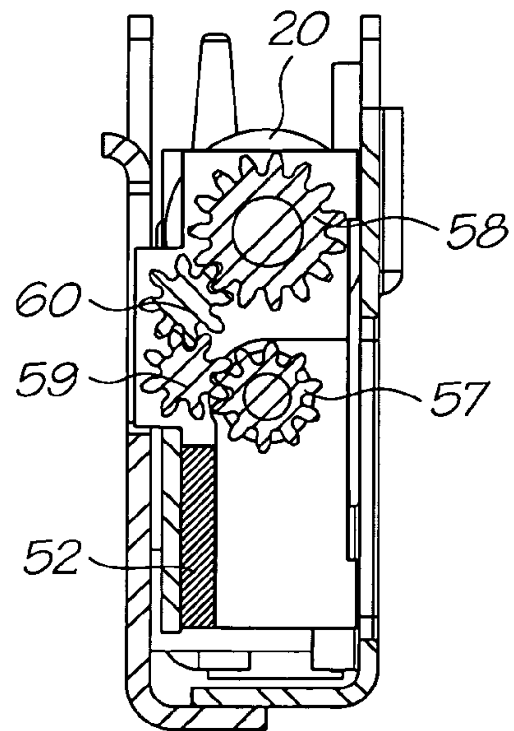
Section B-B
