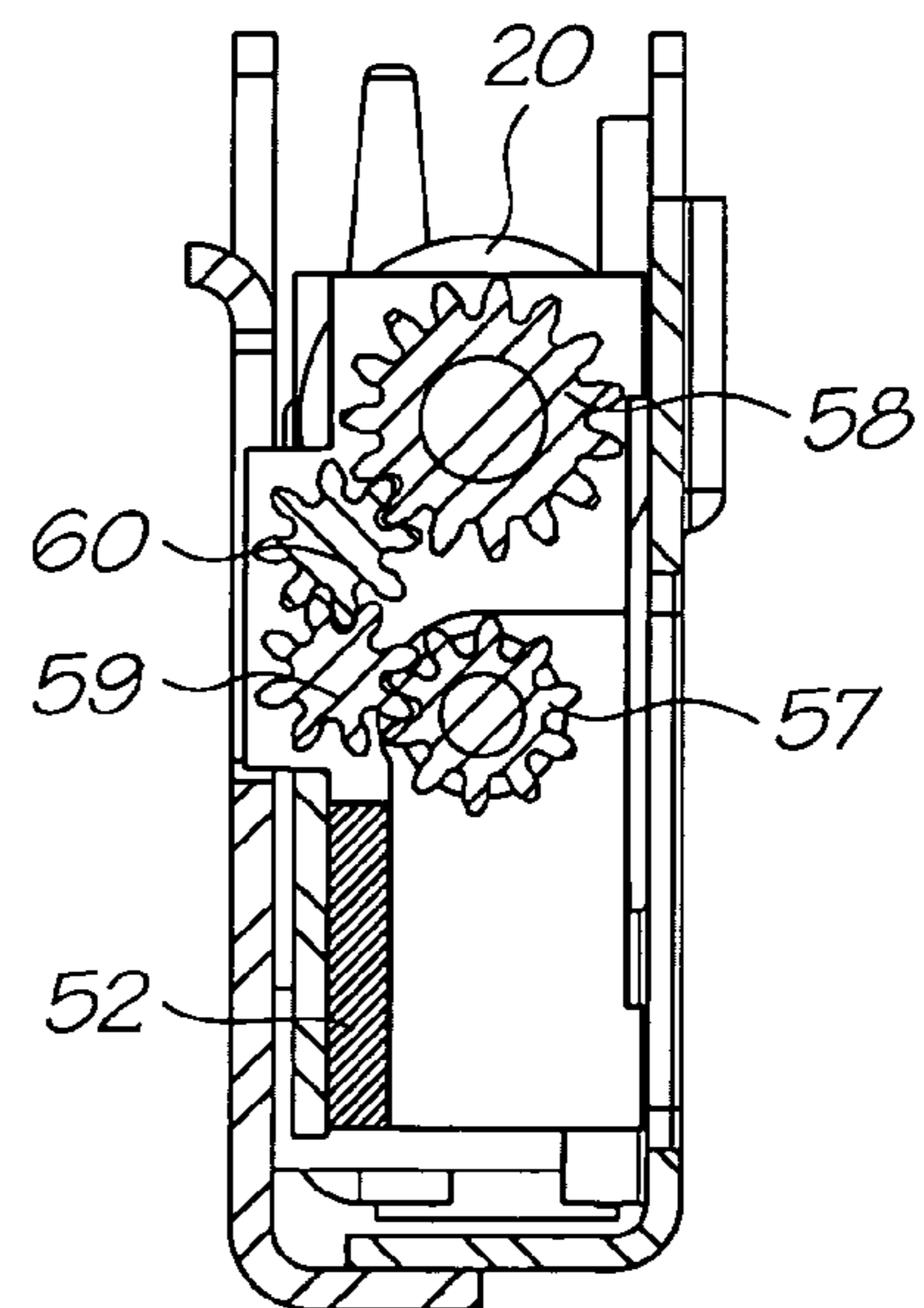
Section B-B
