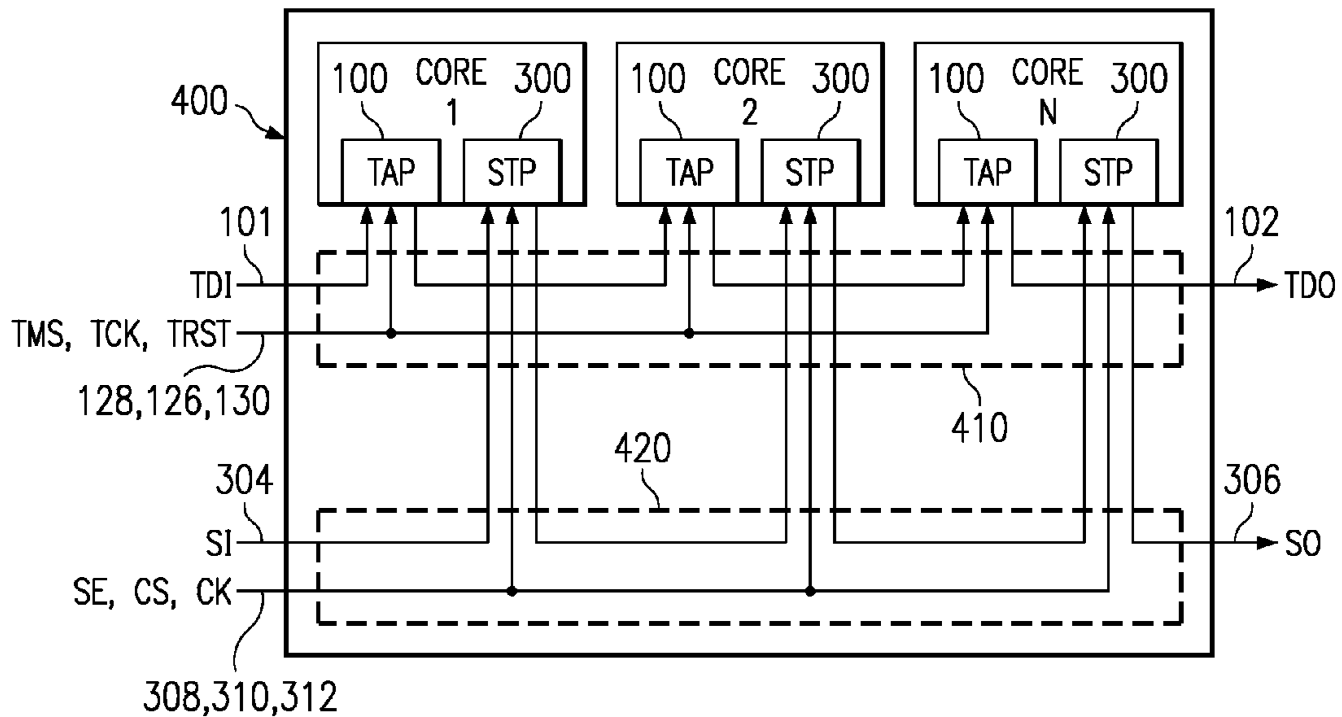
FIG. 4 (PRIOR ART)
