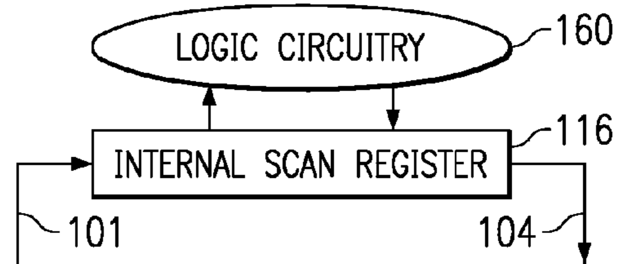
FIG. 1C (PRIOR ART)
