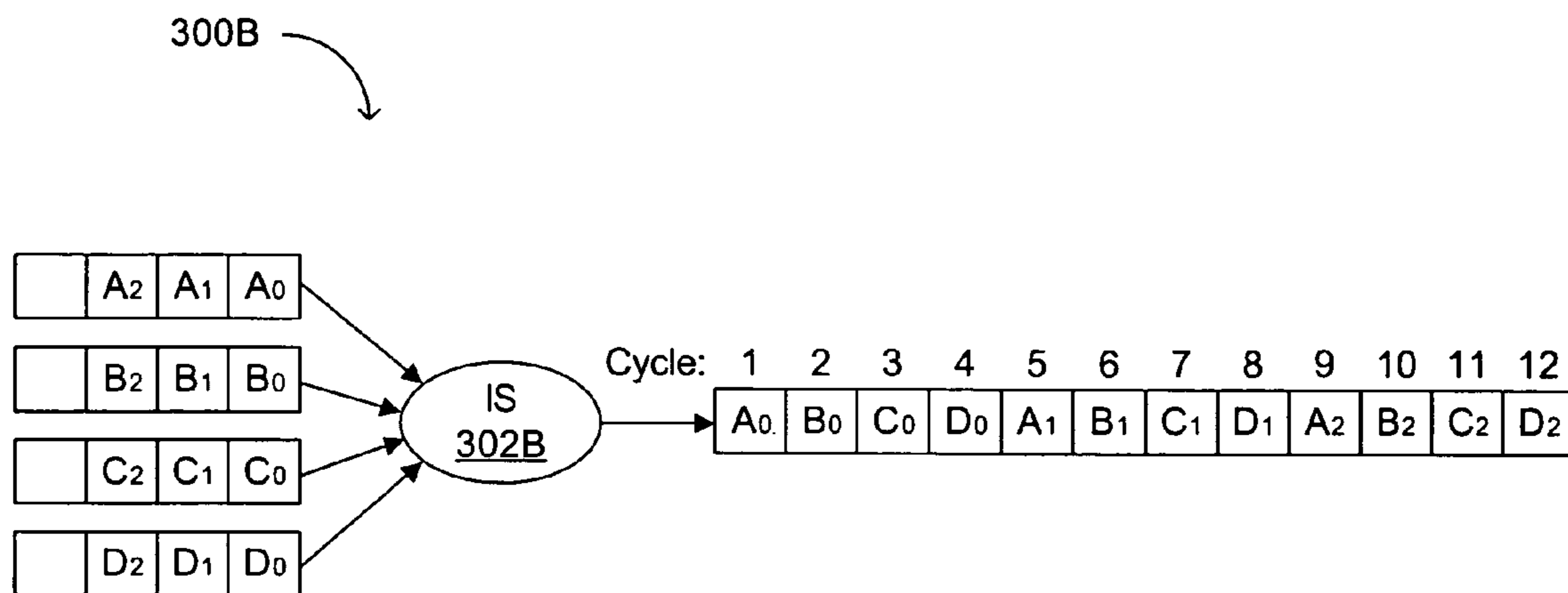
FIG. 3B (conventional)
