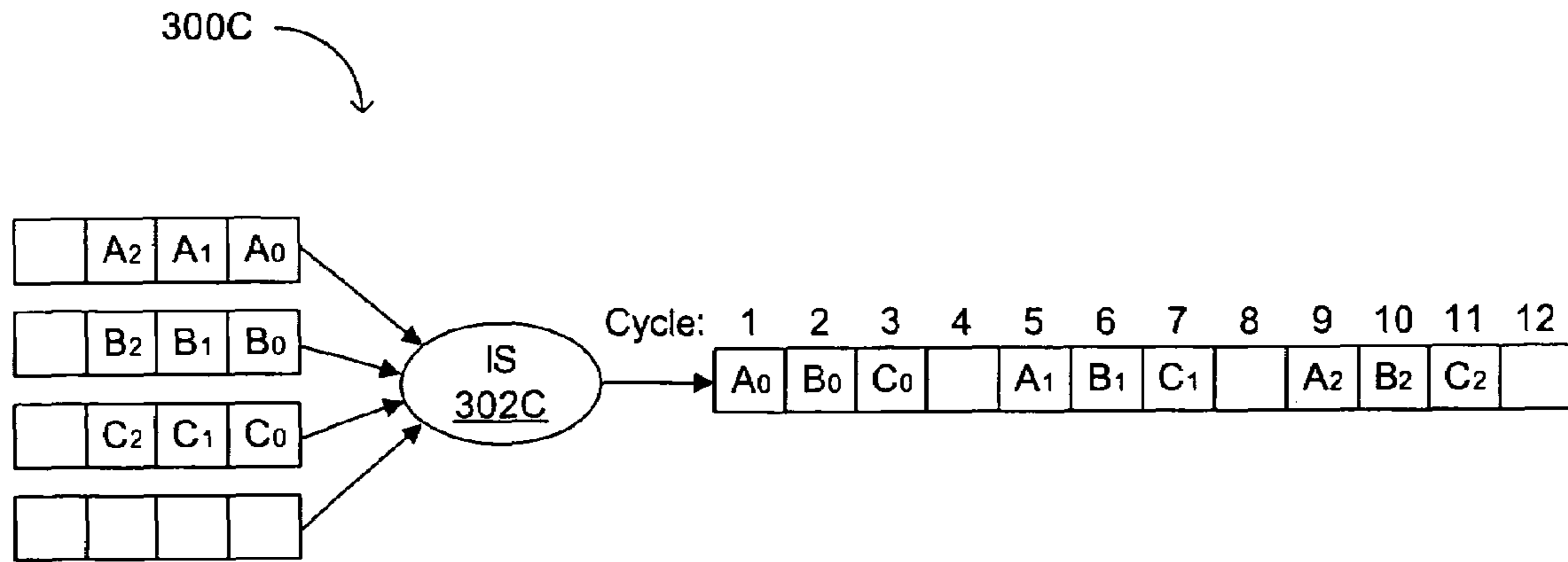
FIG. 3C (conventional)
