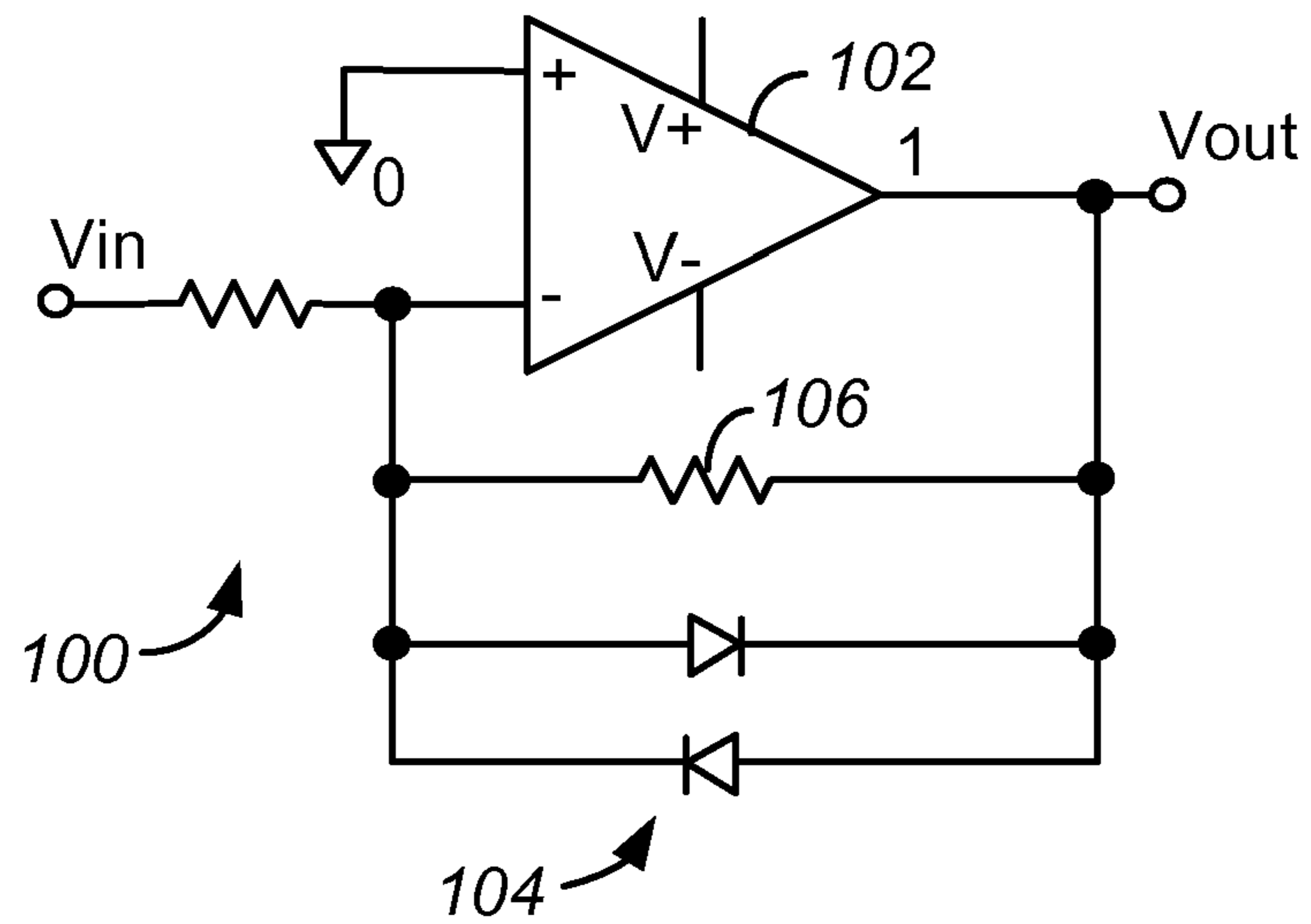
FIG. 4 PRIOR ART
